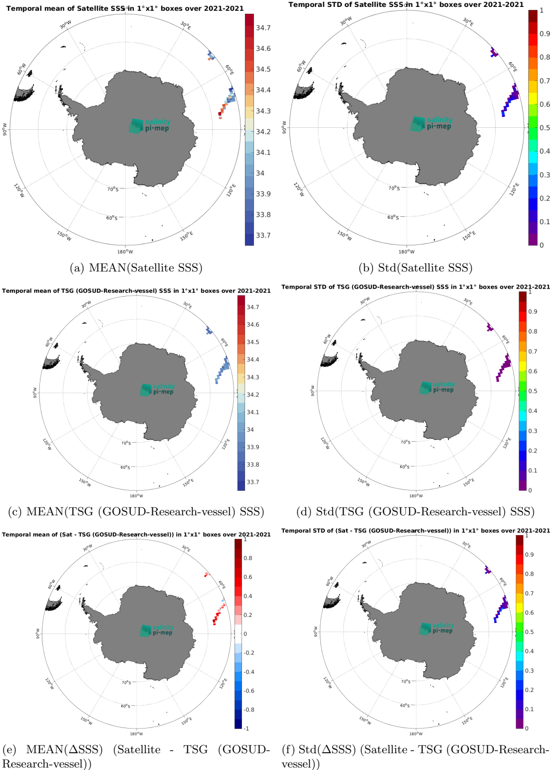
Figure 7: Temporal mean (left) and Std (right) of SSS from SMAP SSS L3 v5.3 - Monthly (RSS) (top), TSG (GOSUD-Research-vessel) (middle), and of \Delta SSS (Satellite - TSG (GOSUD-Research-vessel)). Only match-up pairs are used to generate these maps.
