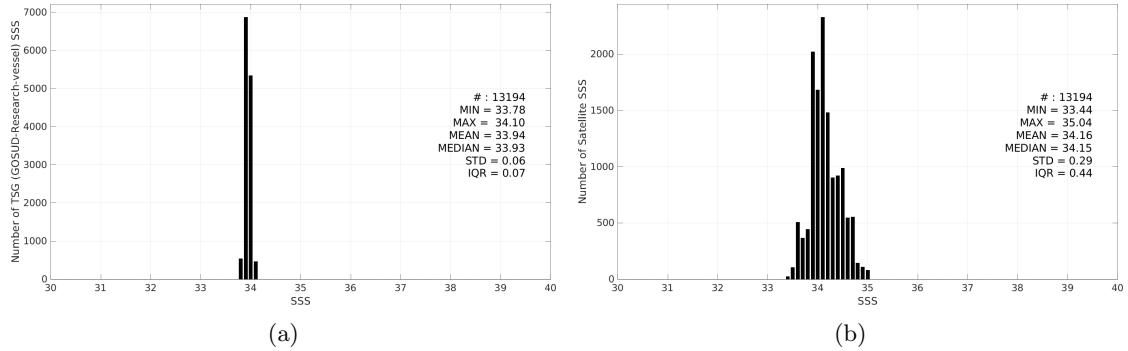
Figure 3: Histograms of SSS from TSG (GOSUD-Research-vessel) (a) and SMAP SSS L3 v5.3 - Monthly (RSS) (b) considering all match-up pairs per bins of 0.1 over the Southern Ocean Pi-MEP region and for the full satellite product period.
