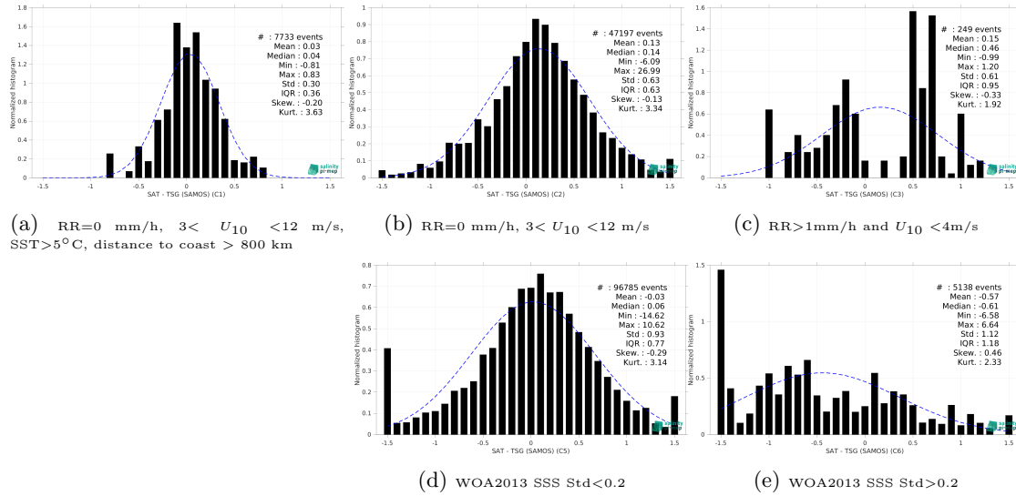
Figure 13: Normalized histogram of \Delta\text{SSS} (SMAP SSS L3 v5 - 8-Day running (RSS) - TSG (SAMOS)) for 5 different subdatasets corresponding to: RR=0 mm/h, 3 < U_{10} < 12 m/s, SST>5°C, distance to coast > 800 km (a), RR=0 mm/h, 3 < U_{10} < 12 m/s (b), RR>1mm/h and U_{10} < 4 m/s (c), WOA2013 SSS Std<0.2 (d), WOA2013 SSS Std>0.2 (e).
