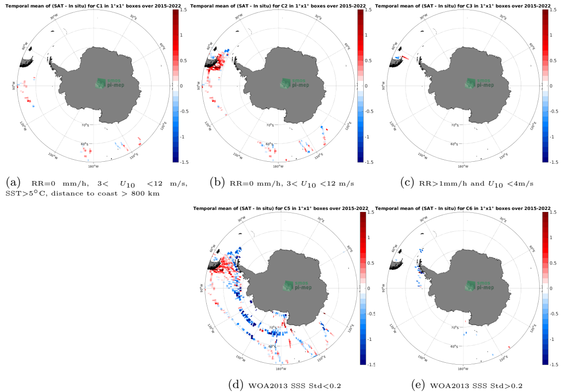
Figure 12: Temporal mean gridded over spatial boxes of size 1^{\circ}\times 1^{\circ} of \Delta\text{SSS} (SMAP SSS L3 v5 - 8-Day running (RSS) - TSG (SAMOS)) for 5 different subdatasets corresponding to:RR=0 mm/h, 3 < U_{10} < 12 m/s, SST > 5^{\circ}\text{C} , distance to coast > 800 km (a), RR=0 mm/h, 3 < U_{10} < 12 m/s (b), RR > 1 mm/h and U_{10} < 4 m/s (c), WOA2013 SSS Std < 0.2 (d), WOA2013 SSS Std > 0.2 (e).
