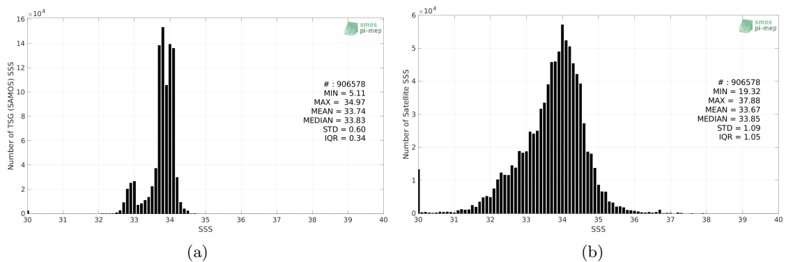
Figure 2: Histograms of SSS from TSG (SAMOS) (a) and SMAP SSS L3 v5 - 8-Day running (RSS) (b) considering all match-up pairs per bins of 0.1 over the Southern Ocean Pi-MEP region and for the full satellite product period.
