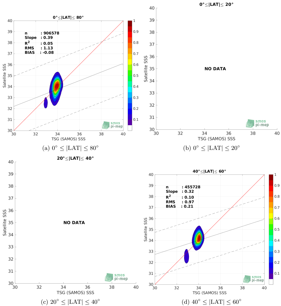
Figure 9: Contour maps of the concentration of SMAP SSS L3 v5 - 8-Day running (RSS) SSS (y-axis) versus TSG (SAMOS) SSS (x-axis) at match-up pairs for different latitude bands. For each plot, the red line shows x=y . The black thin and dashed lines indicate a linear fit through the data cloud and the \pm 95\% confidence levels, respectively. The number match-up pairs n , the slope and R^2 coefficient of the linear fit, the root mean square (RMS) and the mean bias between satellite and in situ data are indicated for each latitude band in each plots.
