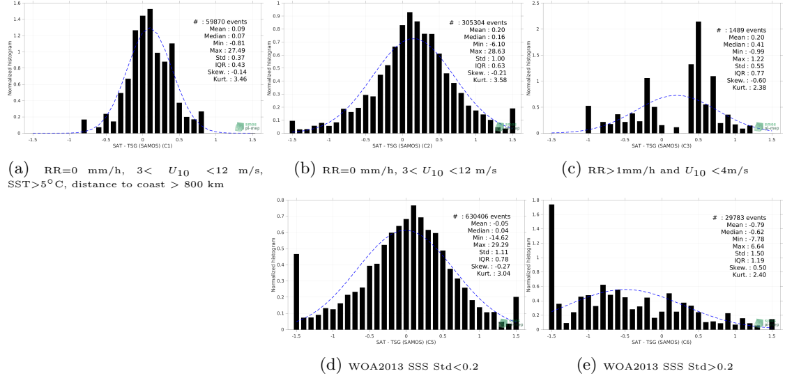
Figure 13: Normalized histogram of \Delta SSS (SMAP SSS L3 v5 - 8-Day running (RSS) - TSG (SAMOS)) for 5 different subdatasets corresponding to: RR=0 mm/h, 3 < U_{10} < 12 m/s, SST > 5°C, distance to coast > 800 km (a), RR=0 mm/h, 3 < U_{10} < 12 m/s (b), RR > 1mm/h and U_{10} < 4 m/s (c), WOA2013 SSS Std < 0.2 (d), WOA2013 SSS Std > 0.2 (e).
