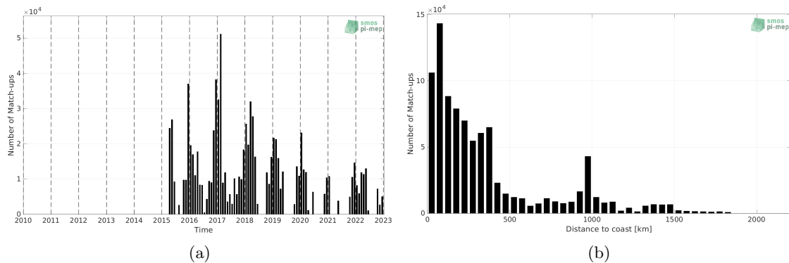
Figure 1: Number of match-ups between TSG (SAMOS) and SMAP SSS L3 v5 - 8-Day running (RSS) SSS as a function of time (a) and as function of the distance to coast (b) over the Southern Ocean Pi-MEP region and for the full satellite product period.
