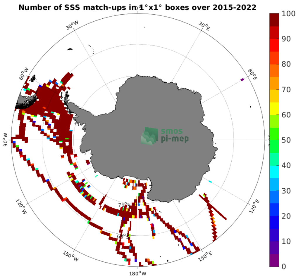
Figure 4: Number of SSS match-ups between TSG (SAMOS) SSS and the SMAP SSS L3 v5 - 8-Day running (RSS) SSS product for the Southern Ocean Pi-MEP region over 1^\circ \times 1^\circ boxes and for the full satellite product period.
