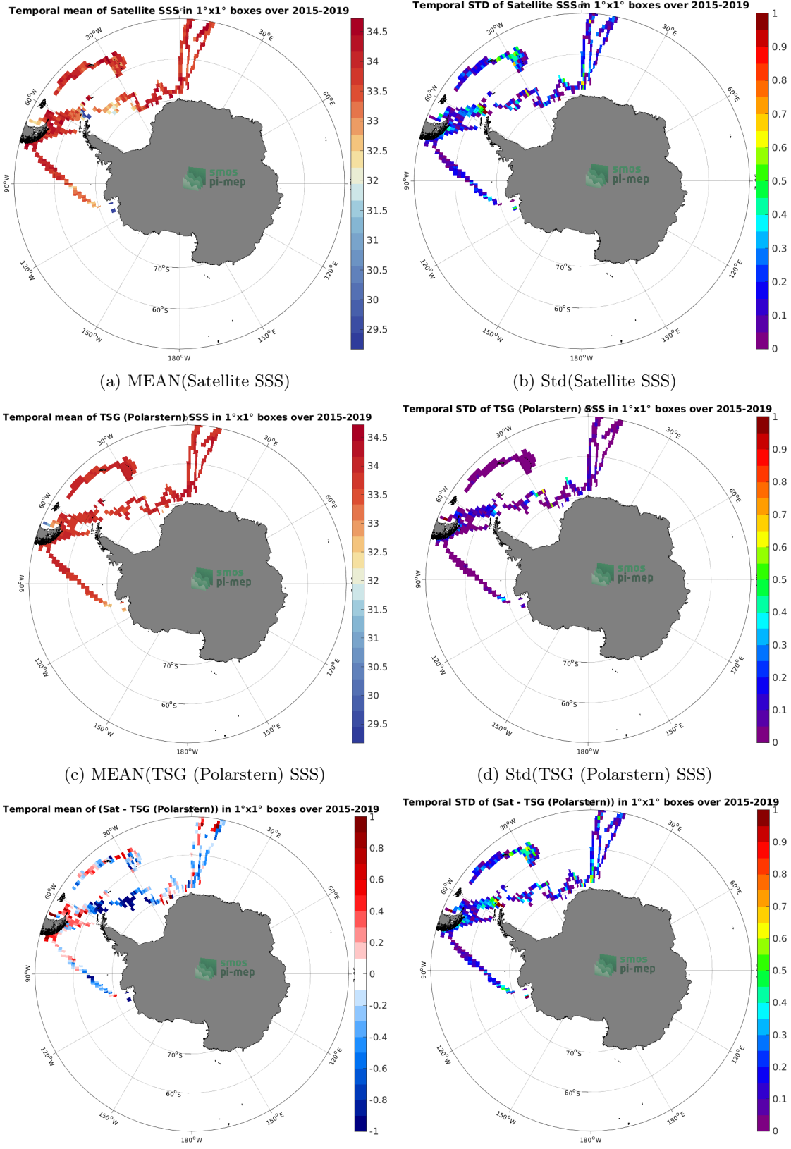
Figure 6: Temporal mean (left) and Std (right) of SSS from SMAP SSS L3 v5 - 8-Day running (RSS) (top), TSG (Polarstern) (middle), and of \Delta SSS (Satellite - TSG (Polarstern)). Only match-up pairs are used to generate these maps.
