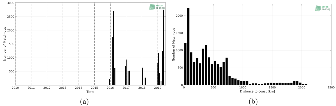
Figure 1: Number of match-ups between TSG (Polarstern) and SMAP SSS L3 v5 - 8-Day running (RSS) SSS as a function of time (a) and as function of the distance to coast (b) over the Southern Ocean Pi-MEP region and for the full satellite product period.
