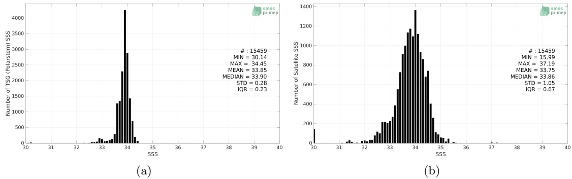
Figure 2: Histograms of SSS from TSG (Polarstern) (a) and SMAP SSS L3 v5 - 8-Day running (RSS) (b) considering all match-up pairs per bins of 0.1 over the Southern Ocean Pi-MEP region and for the full satellite product period.
