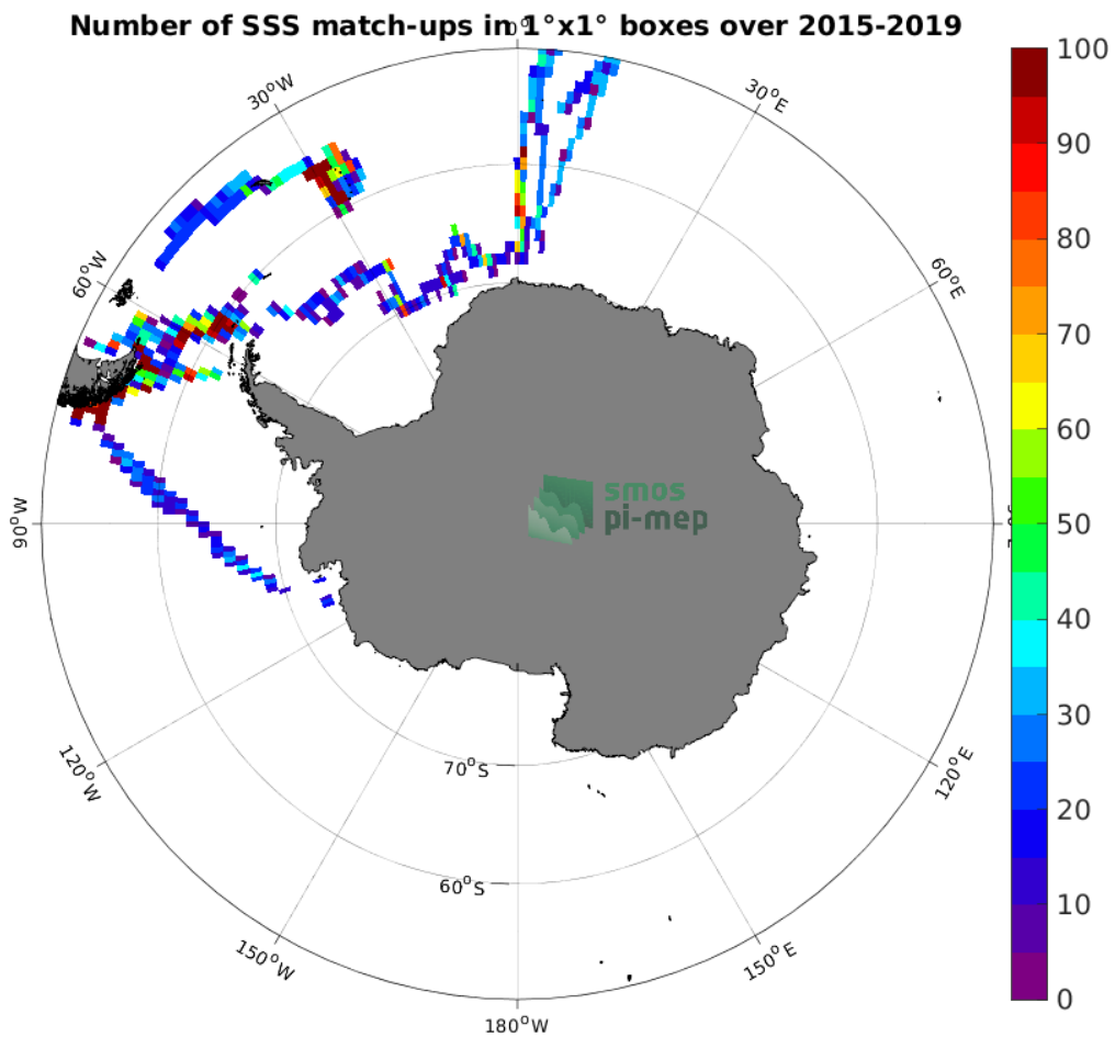
Figure 4: Number of SSS match-ups between TSG (Polarstern) SSS and the SMAP SSS L3 v5 - 8-Day running (RSS) SSS product for the Southern Ocean Pi-MEP region over 1^\circ \times 1^\circ boxes and for the full satellite product period.
