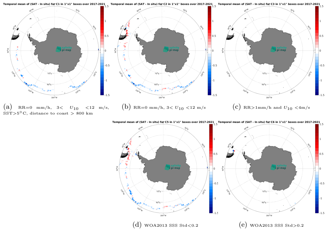
Figure 12: Temporal mean gridded over spatial boxes of size 1^{\circ} \times 1^{\circ} of \Delta SSS (SMAP SSS L3 v5 - 8-Day running (RSS) - TSG (GOSUD-Sailing-ship)) for 5 different subdatasets corresponding to: RR=0 mm/h, 3 < U_{10} < 12 m/s, SST > 5^{\circ}C , distance to coast > 800 km (a), RR=0 mm/h, 3 < U_{10} < 12 m/s (b), RR > 1 mm/h and U_{10} < 4 m/s (c), WOA2013 SSS Std < 0.2 (d), WOA2013 SSS Std > 0.2 (e).
