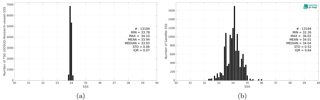
Figure 2: Histograms of SSS from TSG (GOSUD-Research-vessel) (a) and SMAP SSS L3 v5 - 8-Day running (RSS) (b) considering all match-up pairs per bins of 0.1 over the Southern Ocean Pi-MEP region and for the full satellite product period.
