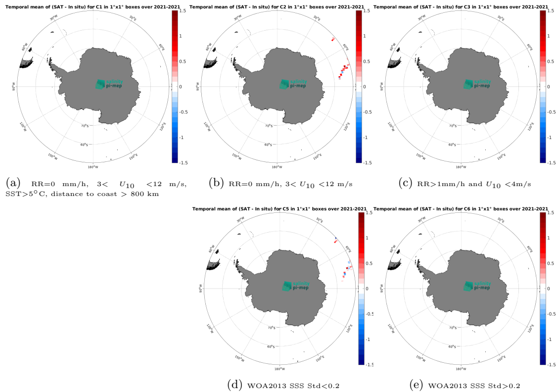
Figure 12: Temporal mean gridded over spatial boxes of size 1^\circ \times 1^\circ of \Delta\text{SSS} (SMAP SSS L3 v5 - 8-Day running (RSS) - TSG (GOSUD-Research-vessel)) for 5 different subdatasets corresponding to: RR=0 mm/h, 3 < U_{10} < 12 m/s, SST > 5^\circ\text{C} , distance to coast > 800 km (a), RR=0 mm/h, 3 < U_{10} < 12 m/s (b), RR > 1 mm/h and U_{10} < 4 m/s (c), WOA2013 SSS Std < 0.2 (d), WOA2013 SSS Std > 0.2 (e).
