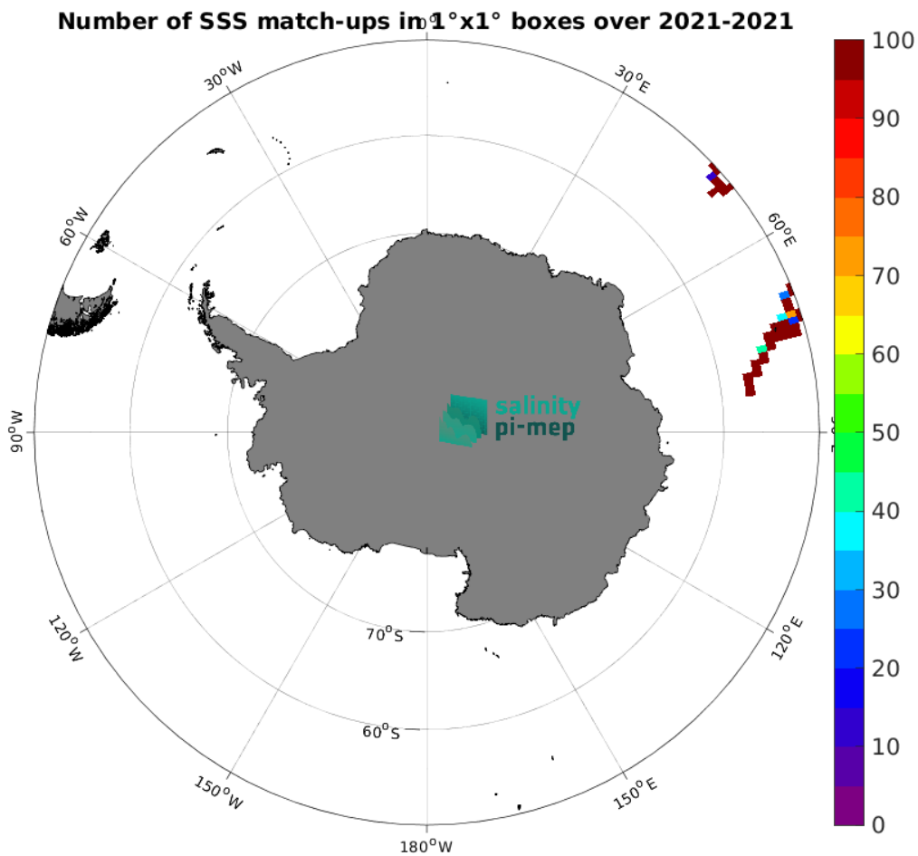
Figure 4: Number of SSS match-ups between TSG (GOSUD-Research-vessel) SSS and the SMAP SSS L3 v5 - 8-Day running (RSS) SSS product for the Southern Ocean Pi-MEP region over 1^\circ \times 1^\circ boxes and for the full satellite product period.
