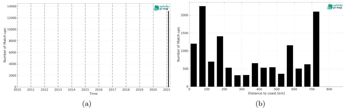
Figure 1: Number of match-ups between TSG (GOSUD-Research-vessel) and SMAP SSS L3 v5 - 8-Day running (RSS) SSS as a function of time (a) and as function of the distance to coast (b) over the Southern Ocean Pi-MEP region and for the full satellite product period.
