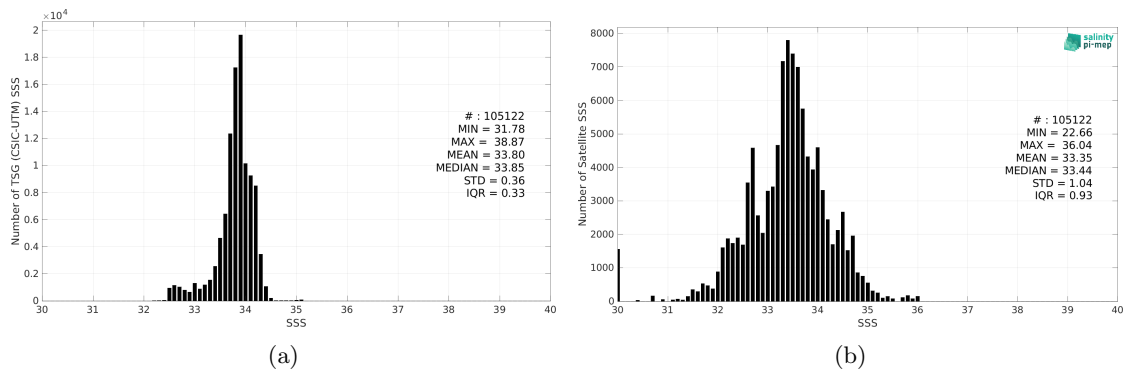
Figure 2: Histograms of SSS from TSG (CSIC-UTM) (a) and SMAP SSS L3 v5 - 8-Day running (RSS) (b) considering all match-up pairs per bins of 0.1 over the Southern Ocean Pi-MEP region and for the full satellite product period.
