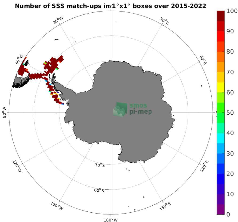
Figure 4: Number of SSS match-ups between TSG (CSIC-UTM) SSS and the SMAP SSS L3 v5 - 8-Day running (RSS) SSS product for the Southern Ocean Pi-MEP region over 1^\circ \times 1^\circ boxes and for the full satellite product period.
