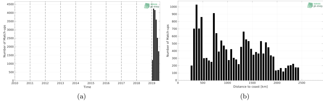
Figure 1: Number of match-ups between Saildrone and SMAP SSS L3 v5 - 8-Day running (RSS) SSS as a function of time (a) and as function of the distance to coast (b) over the Southern Ocean Pi-MEP region and for the full satellite product period.
