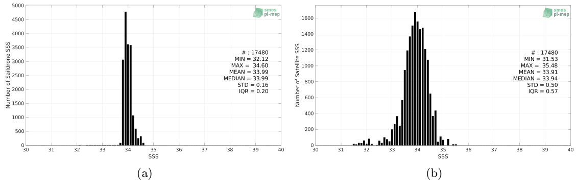
Figure 2: Histograms of SSS from Saildrone (a) and SMAP SSS L3 v5 - 8-Day running (RSS) (b) considering all match-up pairs per bins of 0.1 over the Southern Ocean Pi-MEP region and for the full satellite product period.
