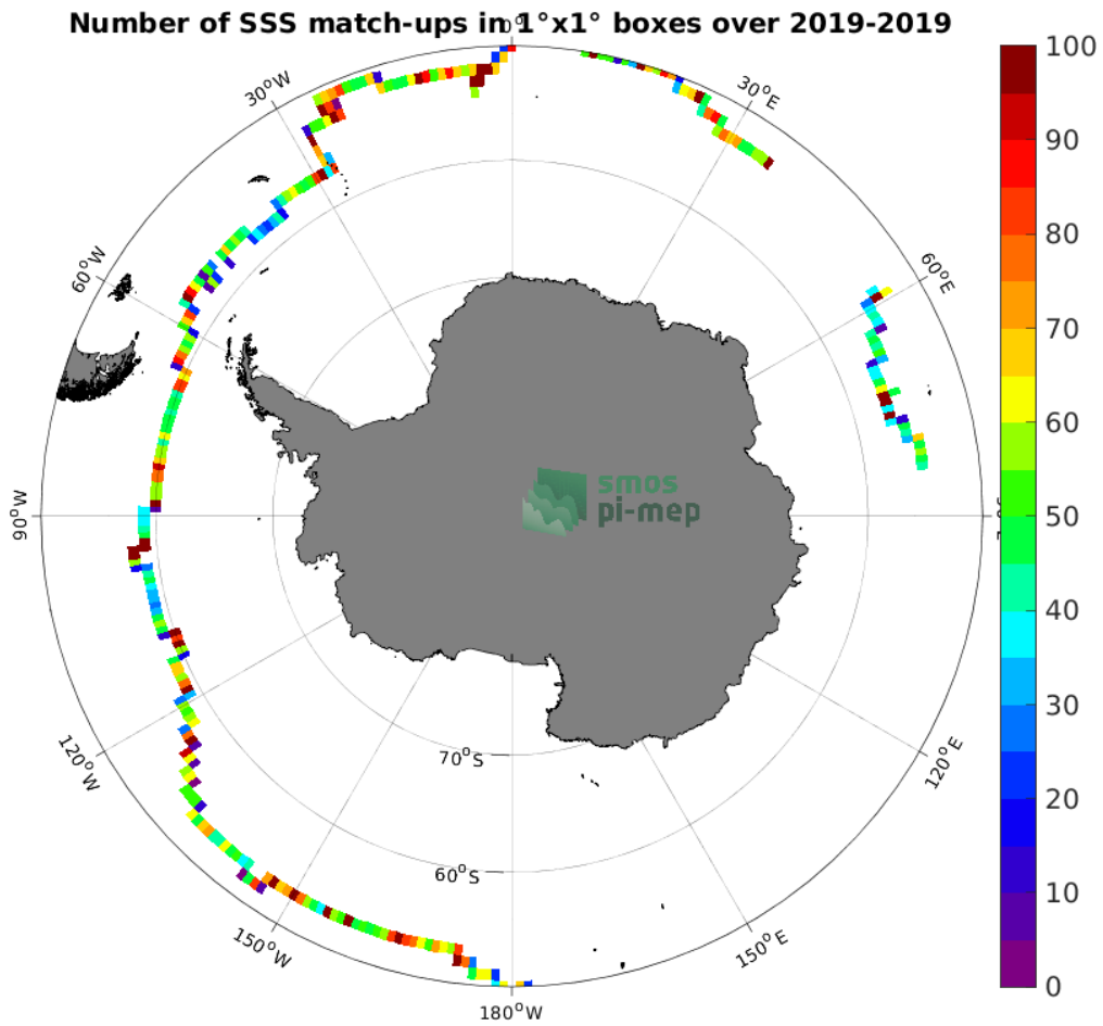
Figure 4: Number of SSS match-ups between Saildrone SSS and the SMAP SSS L3 v5 - 8-Day running (RSS) SSS product for the Southern Ocean Pi-MEP region over 1^\circ \times 1^\circ boxes and for the full satellite product period.
