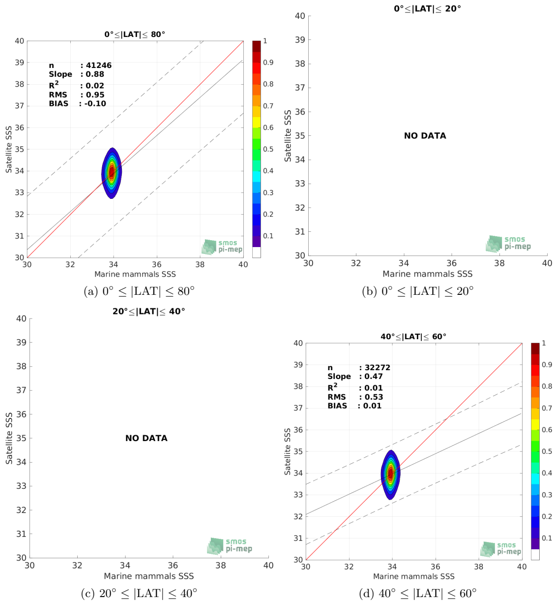
Figure 9: Contour maps of the concentration of SMAP SSS L3 v5 - 8-Day running (RSS) SSS (y-axis) versus Marine mammals SSS (x-axis) at match-up pairs for different latitude bands. For each plot, the red line shows x=y . The black thin and dashed lines indicate a linear fit through the data cloud and the \pm 95\% confidence levels, respectively. The number match-up pairs n , the slope and R^2 coefficient of the linear fit, the root mean square (RMS) and the mean bias between satellite and in situ data are indicated for each latitude band in each plots.
