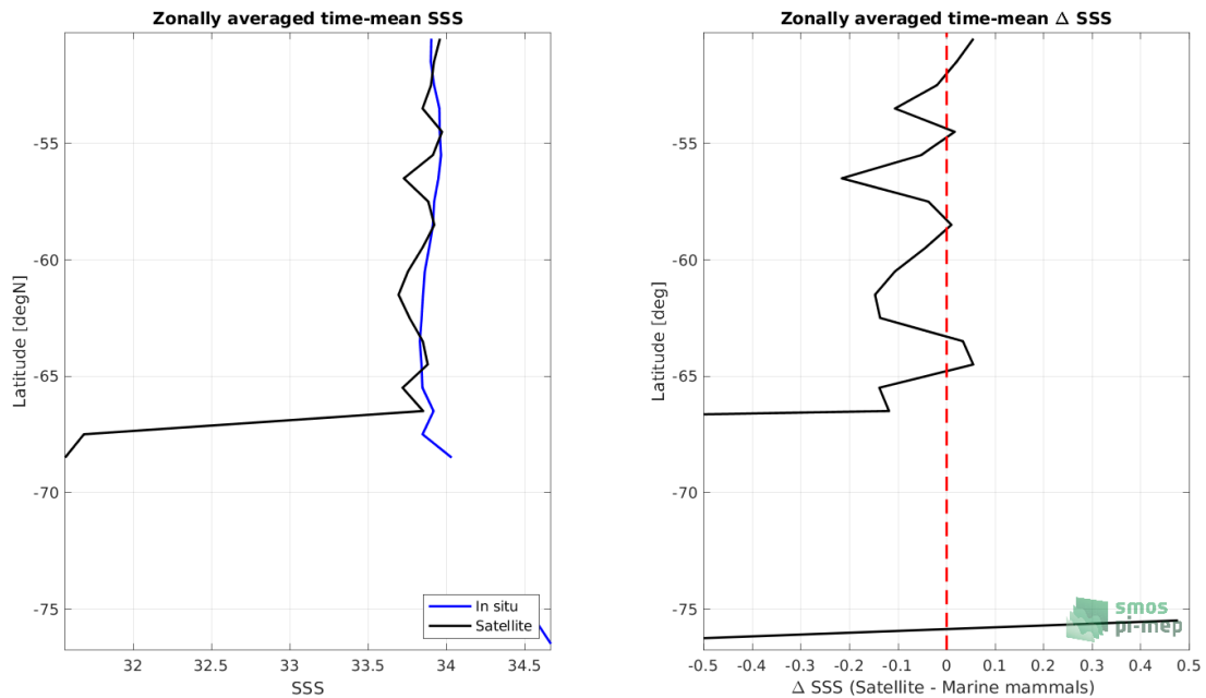
Figure 8: Left panel: Zonal mean SSS from SMAP SSS L3 v5 - 8-Day running (RSS) satellite product (black) and from Marine mammals (blue). Right panel: Zonal mean of \Delta SSS (Satellite - Marine mammals) for all the collected Pi-MEP match-up pairs estimated over the full satellite product period.
