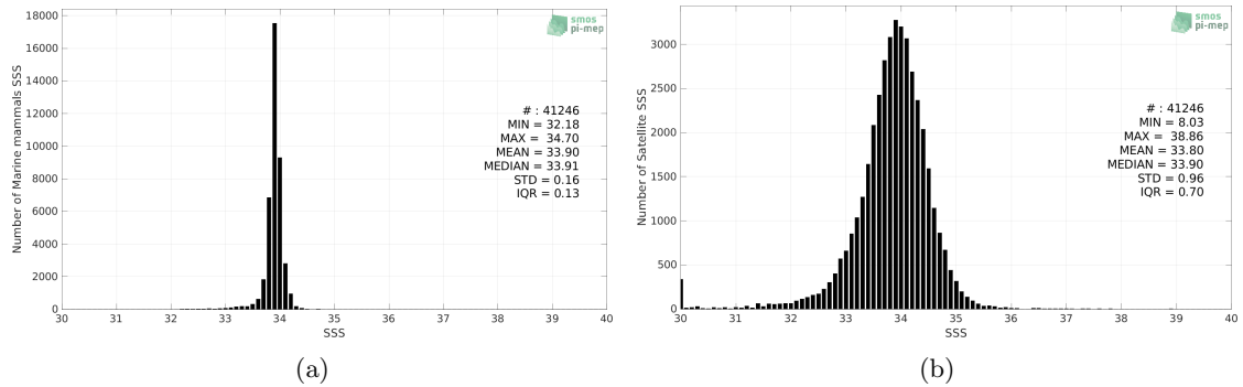
Figure 2: Histograms of SSS from Marine mammals (a) and SMAP SSS L3 v5 - 8-Day running (RSS) (b) considering all match-up pairs per bins of 0.1 over the Southern Ocean Pi-MEP region and for the full satellite product period.
