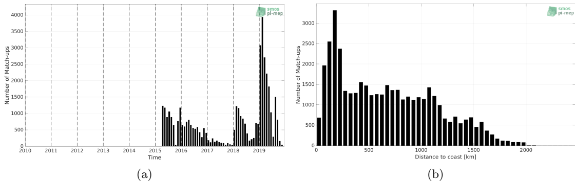
Figure 1: Number of match-ups between Marine mammals and SMAP SSS L3 v5 - 8-Day running (RSS) SSS as a function of time (a) and as function of the distance to coast (b) over the Southern Ocean Pi-MEP region and for the full satellite product period.
