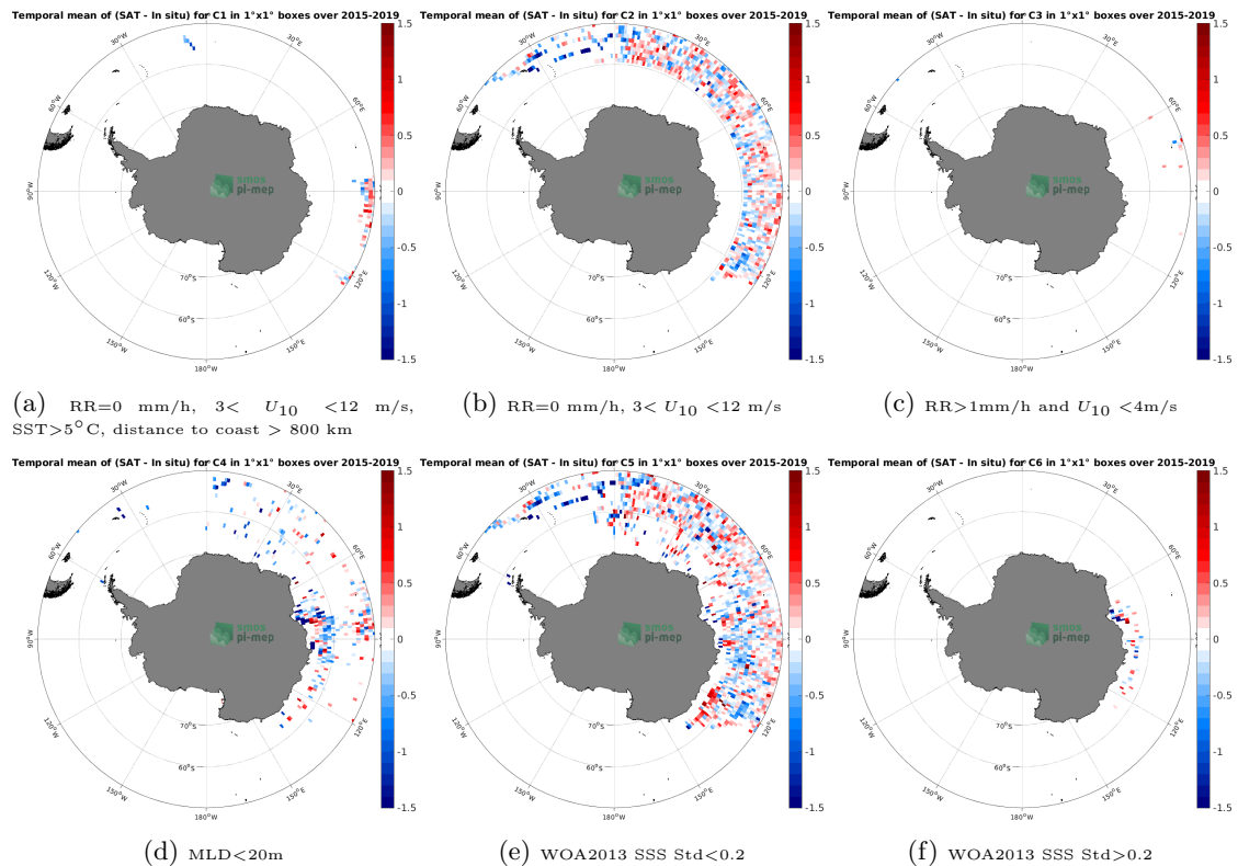
Figure 12: Temporal mean gridded over spatial boxes of size 1^{\circ}\times 1^{\circ} of \Delta\text{SSS} (SMAP SSS L3 v5 - 8-Day running (RSS) - Marine mammals) for 6 different subdatasets corresponding to:RR=0 mm/h, 3 < U_{10} < 12 m/s, SST >5^{\circ}\text{C} , distance to coast > 800 km (a), RR=0 mm/h, 3 < U_{10} < 12 m/s (b), RR >1\text{mm/h} and U_{10} < 4\text{m/s} (c),MLD <20\text{m} (d),WOA2013 SSS Std <0.2 (e),WOA2013 SSS Std >0.2 (f).
