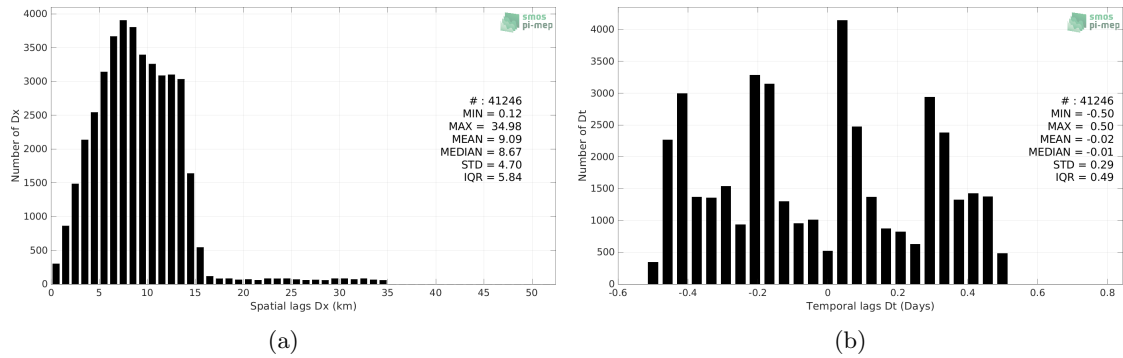
Figure 5: Histograms of the spatial (a) and temporal (b) lags between the location/time of the Marine mammals measurement and the date of the corresponding SMAP SSS L3 v5 - 8-Day running (RSS) SSS pixel.
