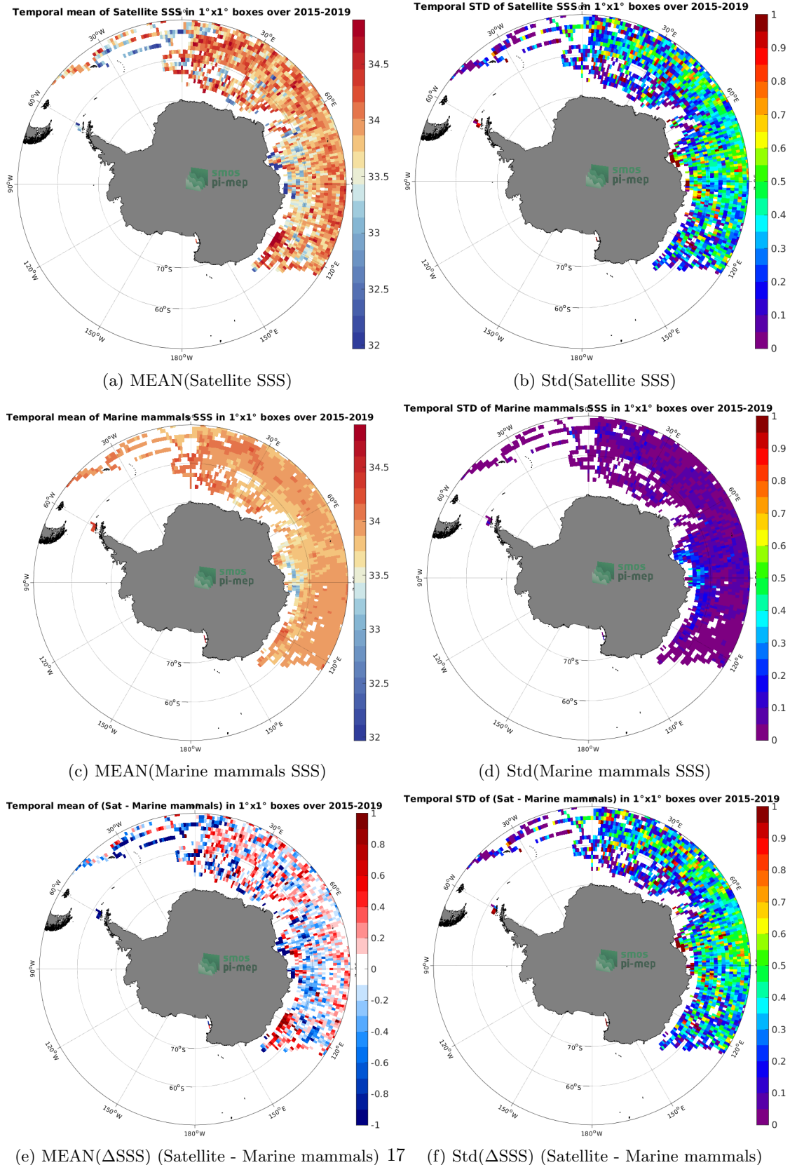
Figure 6: Temporal mean (left) and Std (right) of SSS from SMAP SSS L3 v5 - 8-Day running (RSS) (top), Marine mammals (middle), and of \Delta SSS (Satellite - Marine mammals). Only match-up pairs are used to generate these maps.
