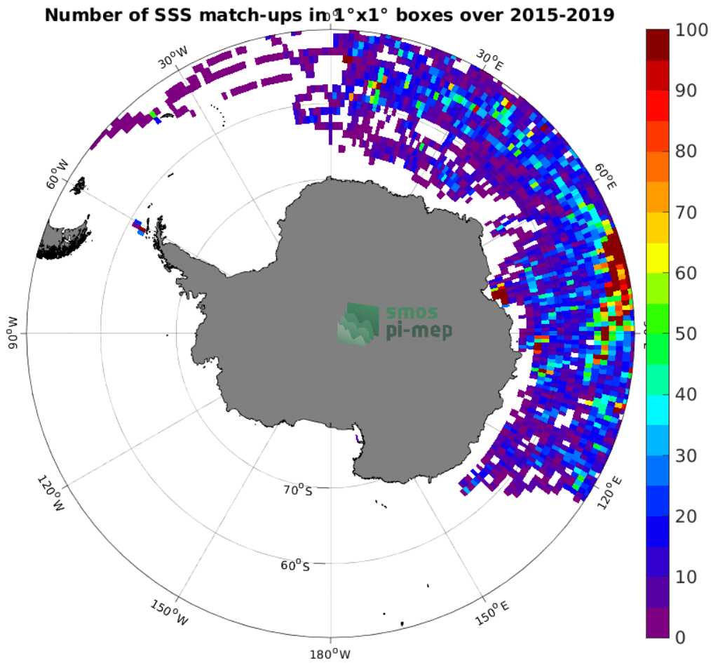
Figure 4: Number of SSS match-ups between Marine mammals SSS and the SMAP SSS L3 v5 - 8-Day running (RSS) SSS product for the Southern Ocean Pi-MEP region over 1^\circ \times 1^\circ boxes and for the full satellite product period.
