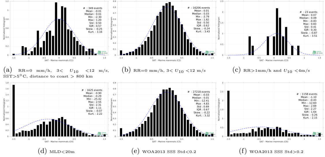
Figure 13: Normalized histogram of \Delta SSS (SMAP SSS L3 v5 - 8-Day running (RSS) - Marine mammals) for 6 different subdatasets corresponding to: RR=0 mm/h, 3 < U_{10} < 12 m/s, SST>5°C, distance to coast > 800 km (a), RR=0 mm/h, 3 < U_{10} < 12 m/s (b), RR>1mm/h and U_{10} < 4 m/s (c), MLD<20m (d), WOA2013 SSS Std<0.2 (e), WOA2013 SSS Std>0.2 (f).
