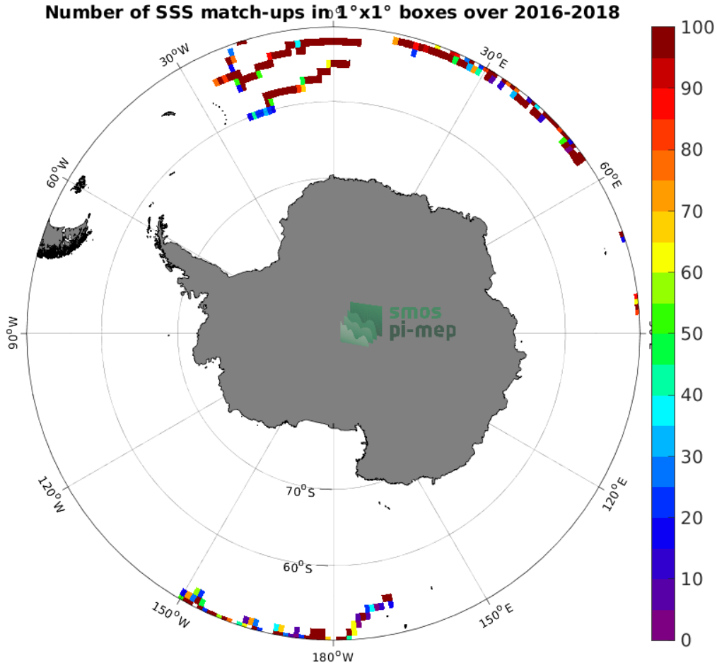
Figure 3: Number of SSS match-ups between Surface drifters SSS and the SMAP SSS L3 v5 - 8-Day running (RSS) SSS product for the Southern Ocean Pi-MEP region over 1^\circ \times 1^\circ boxes and for the full satellite product period.
