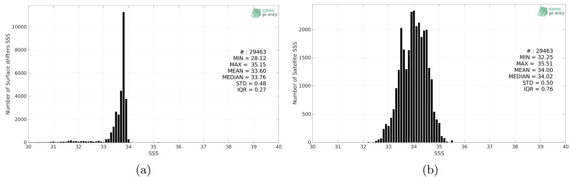
Figure 2: Histograms of SSS from Surface drifters (a) and SMAP SSS L3 v5 - 8-Day running (RSS) (b) considering all match-up pairs per bins of 0.1 over the Southern Ocean Pi-MEP region and for the full satellite product period.
