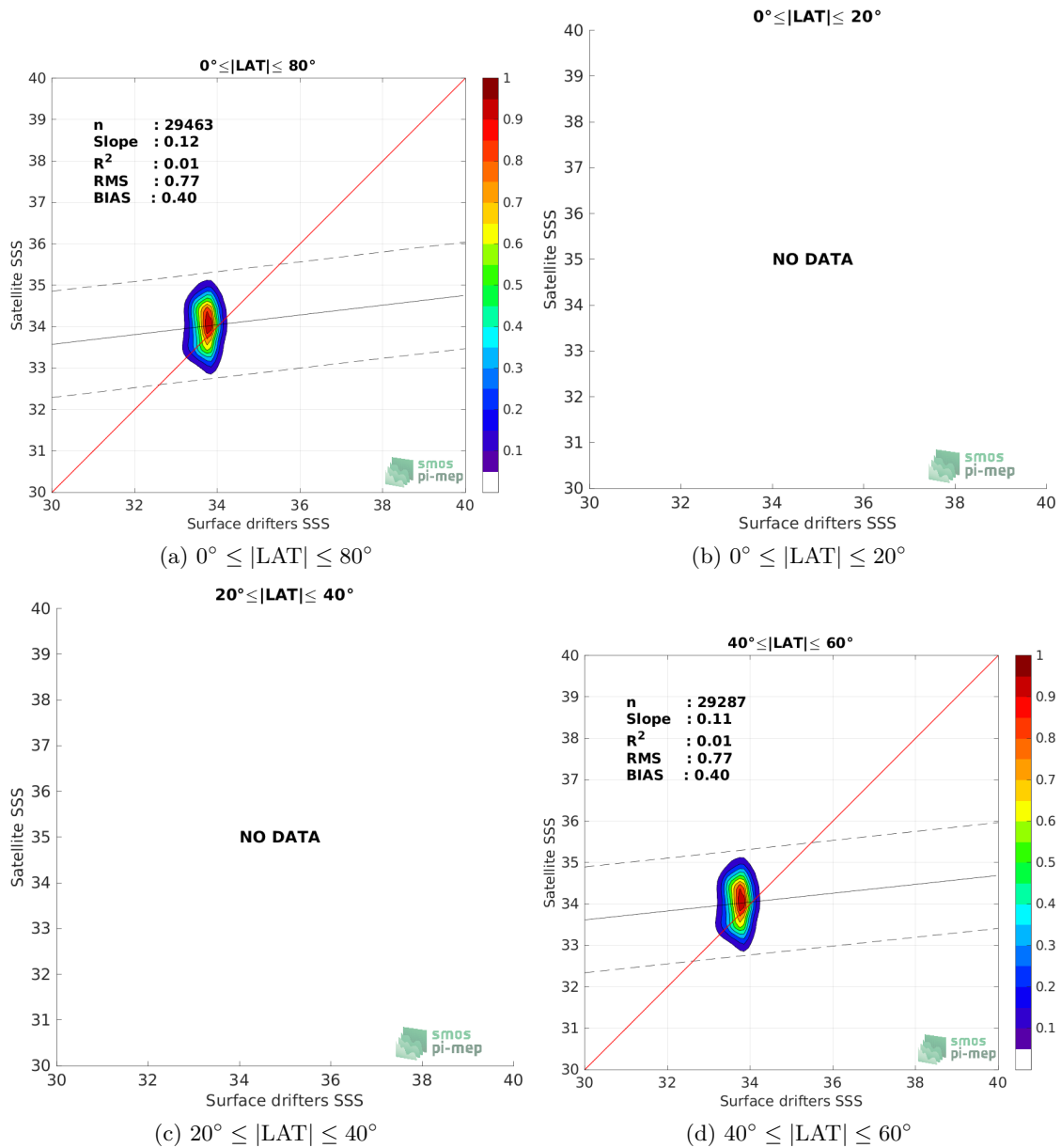
Figure 8: Contour maps of the concentration of SMAP SSS L3 v5 - 8-Day running (RSS) SSS (y-axis) versus Surface drifters SSS (x-axis) at match-up pairs for different latitude bands. For each plot, the red line shows x=y . The black thin and dashed lines indicate a linear fit through the data cloud and the \pm 95\% confidence levels, respectively. The number match-up pairs n , the slope and R^2 coefficient of the linear fit, the root mean square (RMS) and the mean bias between satellite and in situ data are indicated for each latitude band in each plots.
