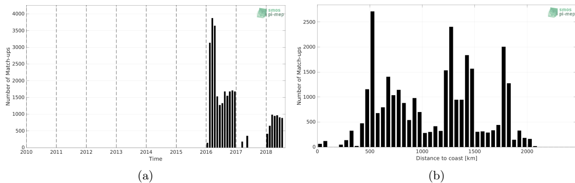
Figure 1: Number of match-ups between Surface drifters and SMAP SSS L3 v5 - 8-Day running (RSS) SSS as a function of time (a) and as function of the distance to coast (b) over the Southern Ocean Pi-MEP region and for the full satellite product period.
