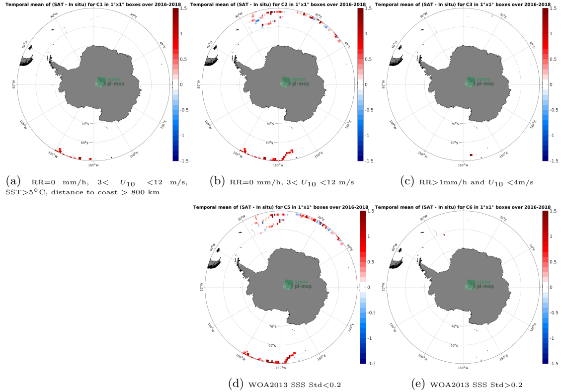
Figure 11: Temporal mean gridded over spatial boxes of size 1^{\circ}\times 1^{\circ} of \Delta\text{SSS} (SMAP SSS L3 v5 - 8-Day running (RSS) - Surface drifters) for 5 different subdatasets corresponding to:RR=0 mm/h, 3 < U_{10} < 12 m/s, SST >5^{\circ}\text{C} , distance to coast > 800 km (a), RR=0 mm/h, 3 < U_{10} < 12 m/s (b), RR >1 mm/h and U_{10} < 4 m/s (c), WOA2013 SSS Std <0.2 (d), WOA2013 SSS Std >0.2 (e).
