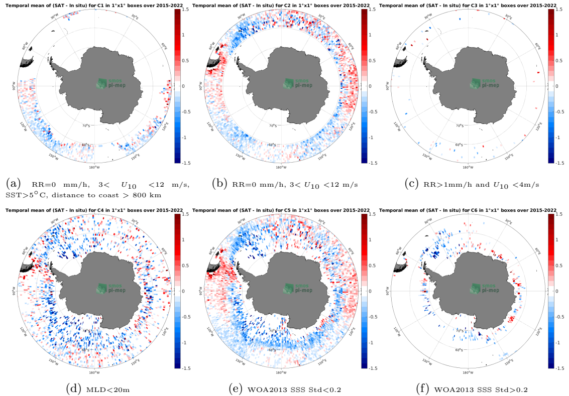
Figure 12: Temporal mean gridded over spatial boxes of size 1^{\circ}\times 1^{\circ} of \Delta\text{SSS} (SMAP SSS L3 v5 - 8-Day running (RSS) - Argo) for 6 different subdatasets corresponding to:RR=0 mm/h, 3 < U_{10} < 12 m/s, SST >5^{\circ}\text{C} , distance to coast > 800 km (a), RR=0 mm/h, 3 < U_{10} < 12 m/s (b), RR >1\text{mm/h} and U_{10} < 4\text{m/s} (c),MLD <20\text{m} (d),WOA2013 SSS Std <0.2 (e),WOA2013 SSS Std >0.2 (f).
