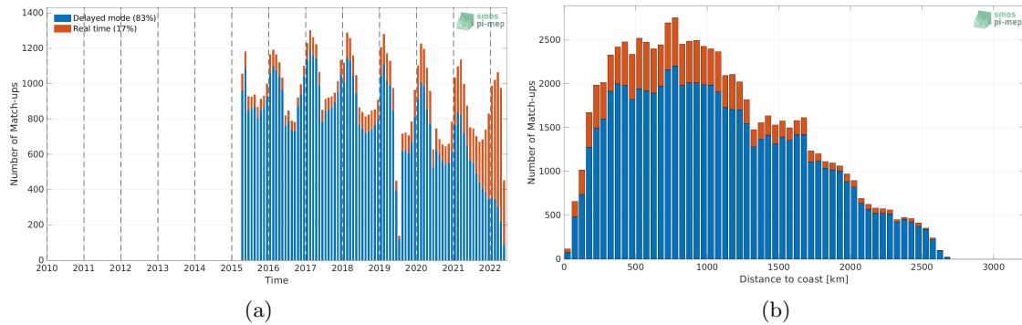
Figure 1: Number of match-ups between Argo and SMAP SSS L3 v5 - 8-Day running (RSS) SSS as a function of time (a) and as function of the distance to coast (b) over the Southern Ocean Pi-MEP region and for the full satellite product period.
