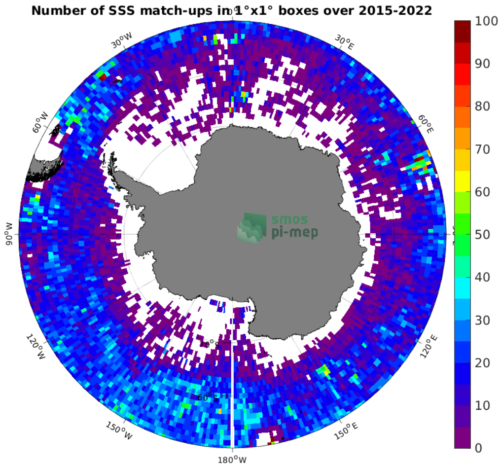
Figure 4: Number of SSS match-ups between Argo SSS and the SMAP SSS L3 v5 - 8-Day running (RSS) SSS product for the Southern Ocean Pi-MEP region over 1^\circ \times 1^\circ boxes and for the full satellite product period.
