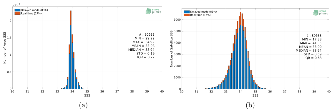
Figure 2: Histograms of SSS from Argo (a) and SMAP SSS L3 v5 - 8-Day running (RSS) (b) considering all match-up pairs per bins of 0.1 over the Southern Ocean Pi-MEP region and for the full satellite product period.
