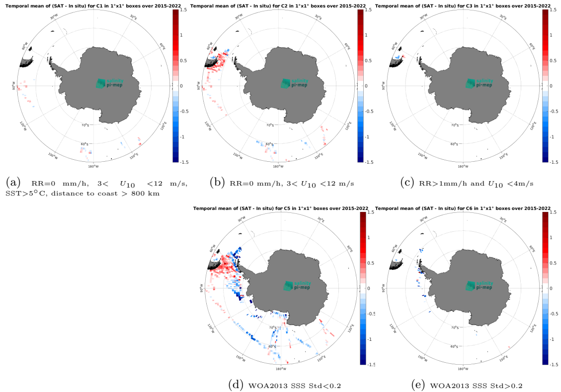
Figure 12: Temporal mean gridded over spatial boxes of size 1^{\circ}\times 1^{\circ} of \Delta\text{SSS} (SMAP SSS L3 v5 - Monthly (RSS) - TSG (SAMOS)) for 5 different subdatasets corresponding to: \text{RR}=0 mm/h, 3 < U_{10} < 12 m/s, \text{SST}>5^{\circ}\text{C} , distance to coast > 800 km (a), \text{RR}=0 mm/h, 3 < U_{10} < 12 m/s (b), \text{RR}>1 mm/h and U_{10} < 4 m/s (c), WOA2013 SSS Std < 0.2 (d), WOA2013 SSS Std > 0.2 (e).
