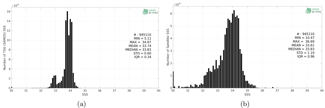
Figure 2: Histograms of SSS from TSG (SAMOS) (a) and SMAP SSS L3 v5 - Monthly (RSS) (b) considering all match-up pairs per bins of 0.1 over the Southern Ocean Pi-MEP region and for the full satellite product period.
