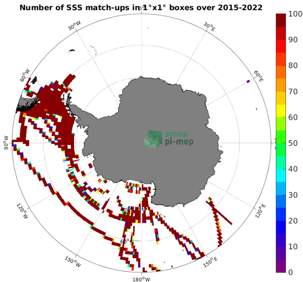
Figure 4: Number of SSS match-ups between TSG (SAMOS) SSS and the SMAP SSS L3 v5 - Monthly (RSS) SSS product for the Southern Ocean Pi-MEP region over 1^\circ \times 1^\circ boxes and for the full satellite product period.
