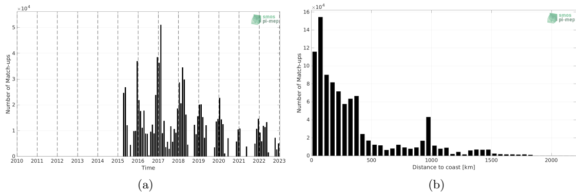
Figure 1: Number of match-ups between TSG (SAMOS) and SMAP SSS L3 v5 - Monthly (RSS) SSS as a function of time (a) and as function of the distance to coast (b) over the Southern Ocean Pi-MEP region and for the full satellite product period.
