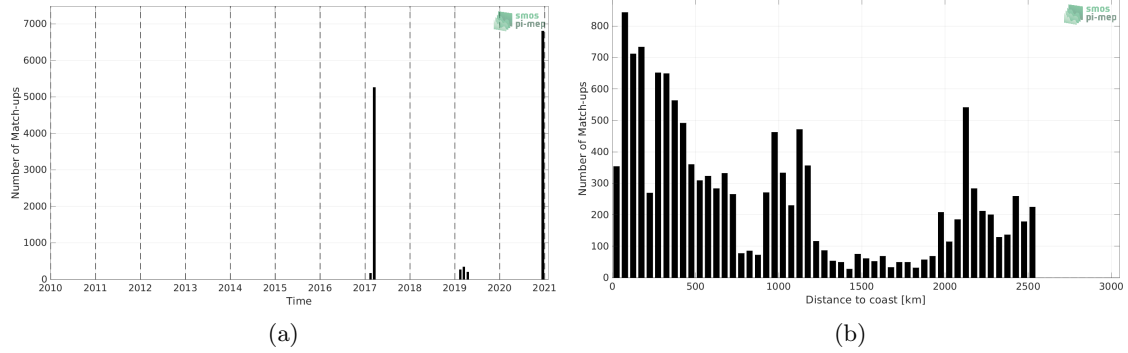
Figure 1: Number of match-ups between TSG (GOSUD-Sailing-ship) and SMAP SSS L3 v5 - Monthly (RSS) SSS as a function of time (a) and as function of the distance to coast (b) over the Southern Ocean Pi-MEP region and for the full satellite product period.
