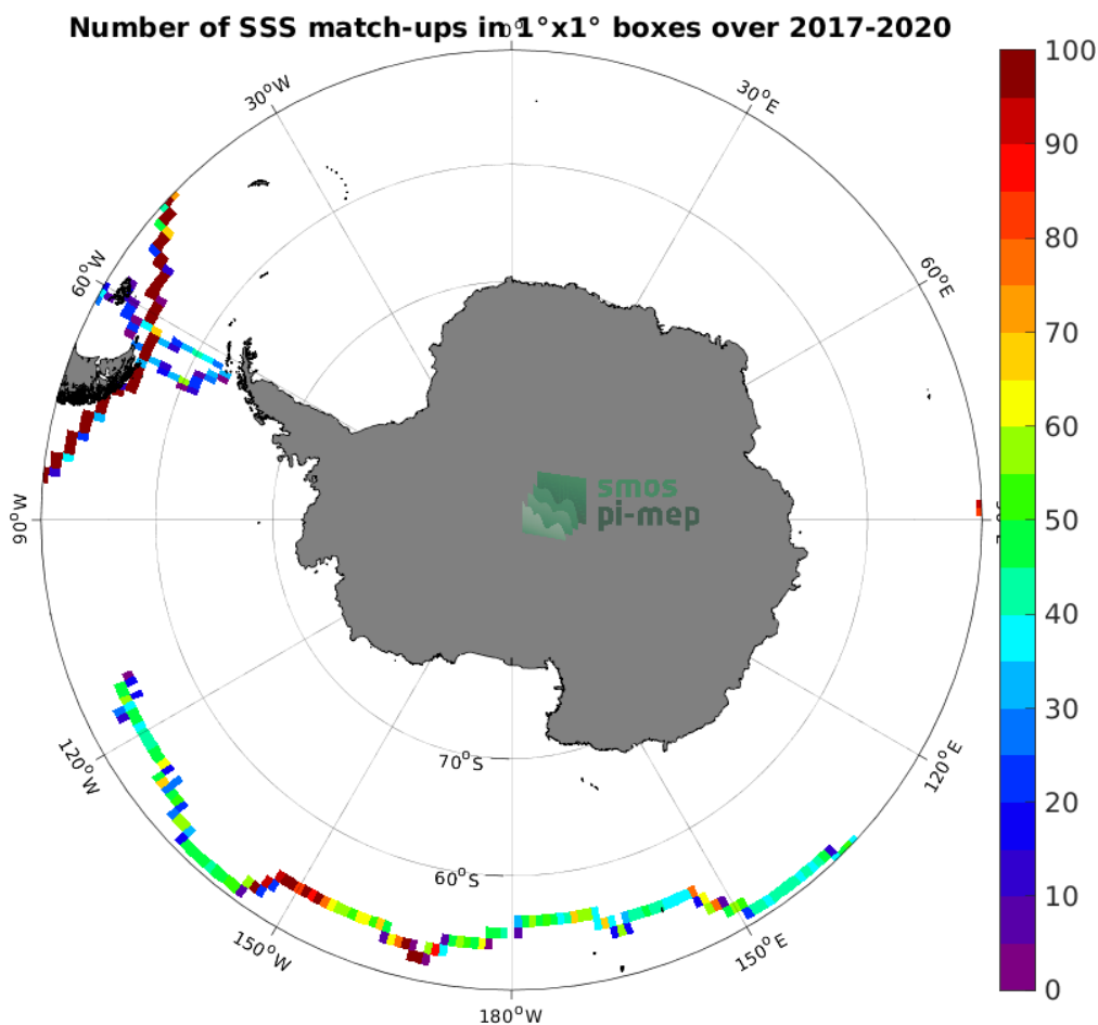
Figure 4: Number of SSS match-ups between TSG (GOSUD-Sailing-ship) SSS and the SMAP SSS L3 v5 - Monthly (RSS) SSS product for the Southern Ocean Pi-MEP region over 1^\circ \times 1^\circ boxes and for the full satellite product period.
