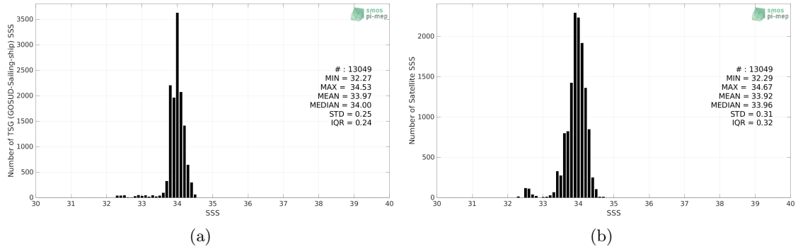
Figure 2: Histograms of SSS from TSG (GOSUD-Sailing-ship) (a) and SMAP SSS L3 v5 - Monthly (RSS) (b) considering all match-up pairs per bins of 0.1 over the Southern Ocean Pi-MEP region and for the full satellite product period.
