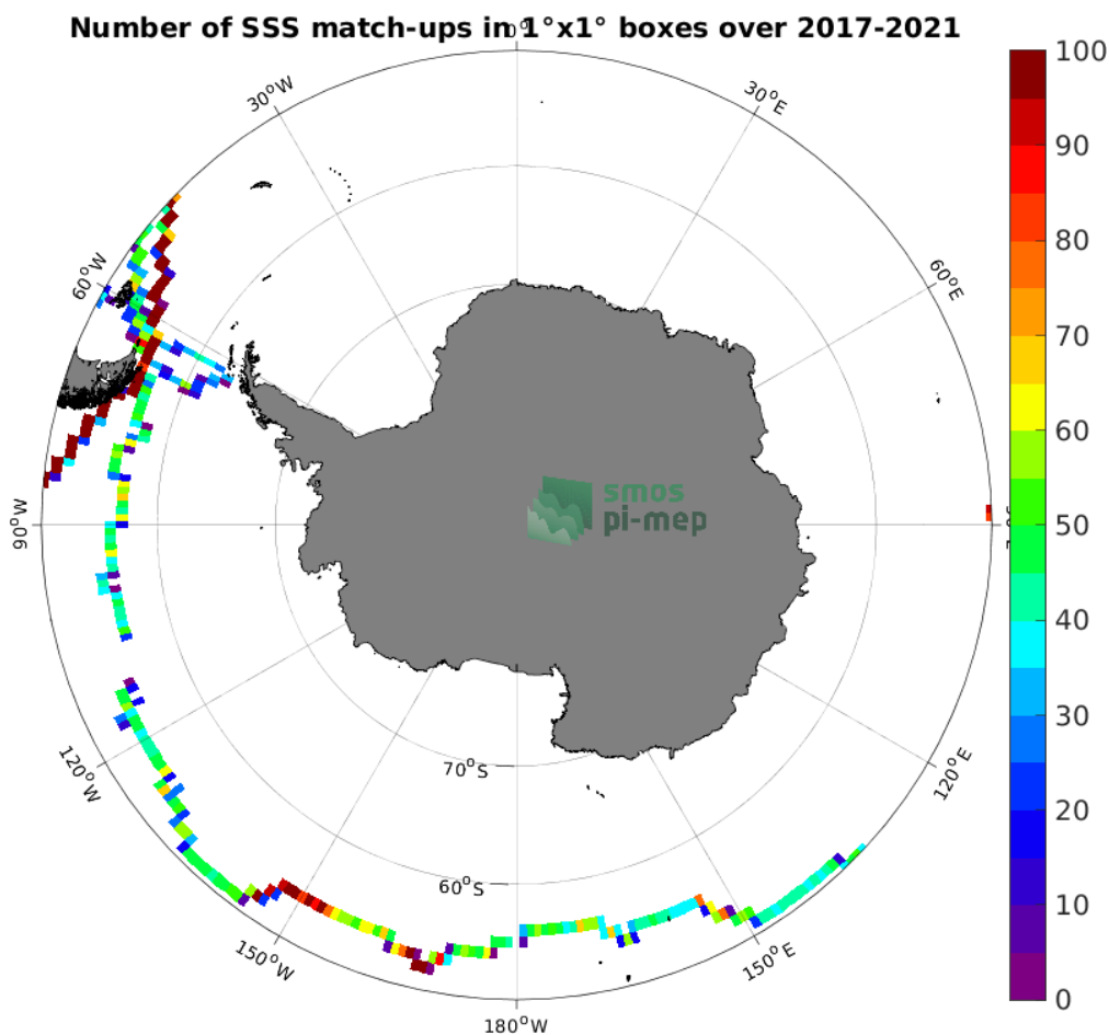
Figure 4: Number of SSS match-ups between TSG (GOSUD-Sailing-ship) SSS and the SMAP SSS L3 v5 - Monthly (RSS) SSS product for the Southern Ocean Pi-MEP region over 1^{\circ} \times 1^{\circ} boxes and for the full satellite product period.
