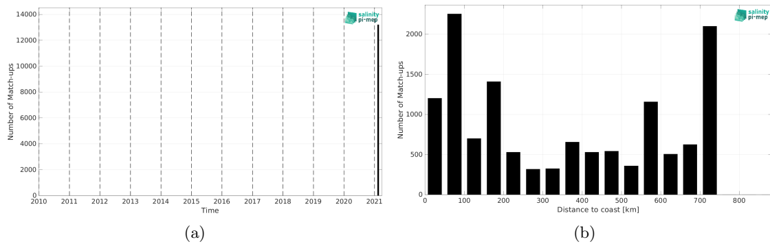
Figure 1: Number of match-ups between TSG (GOSUD-Research-vessel) and SMAP SSS L3 v5 - Monthly (RSS) SSS as a function of time (a) and as function of the distance to coast (b) over the Southern Ocean Pi-MEP region and for the full satellite product period.
