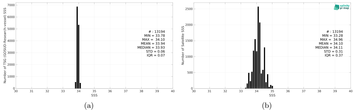
Figure 2: Histograms of SSS from TSG (GOSUD-Research-vessel) (a) and SMAP SSS L3 v5 - Monthly (RSS) (b) considering all match-up pairs per bins of 0.1 over the Southern Ocean Pi-MEP region and for the full satellite product period.
