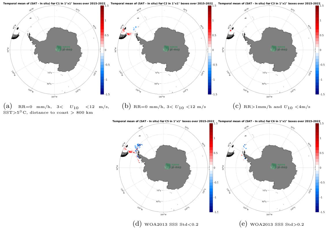
Figure 12: Temporal mean gridded over spatial boxes of size 1^{\circ}\times 1^{\circ} of \Delta\text{SSS} (SMAP SSS L3 v5 - Monthly (RSS) - TSG (CSIC-UTM)) for 5 different subdatasets corresponding to: \text{RR}=0 mm/h, 3 < U_{10} < 12 m/s, \text{SST}>5^{\circ}\text{C} , distance to coast > 800 km (a), \text{RR}=0 mm/h, 3 < U_{10} < 12 m/s (b), \text{RR}>1\text{mm/h} and U_{10} < 4\text{m/s} (c), WOA2013 SSS Std < 0.2 (d), WOA2013 SSS Std > 0.2 (e).
