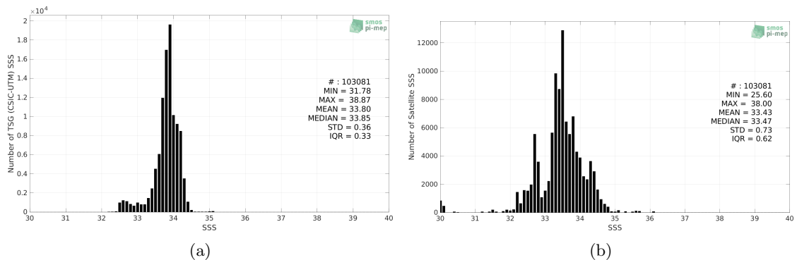
Figure 2: Histograms of SSS from TSG (CSIC-UTM) (a) and SMAP SSS L3 v5 - Monthly (RSS) (b) considering all match-up pairs per bins of 0.1 over the Southern Ocean Pi-MEP region and for the full satellite product period.
