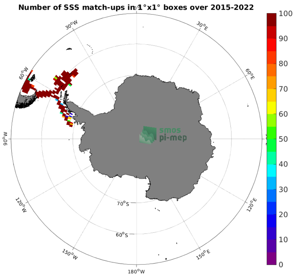
Figure 4: Number of SSS match-ups between TSG (CSIC-UTM) SSS and the SMAP SSS L3 v5 - Monthly (RSS) SSS product for the Southern Ocean Pi-MEP region over 1^\circ \times 1^\circ boxes and for the full satellite product period.
