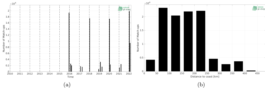
Figure 1: Number of match-ups between TSG (CSIC-UTM) and SMAP SSS L3 v5 - Monthly (RSS) SSS as a function of time (a) and as function of the distance to coast (b) over the Southern Ocean Pi-MEP region and for the full satellite product period.
