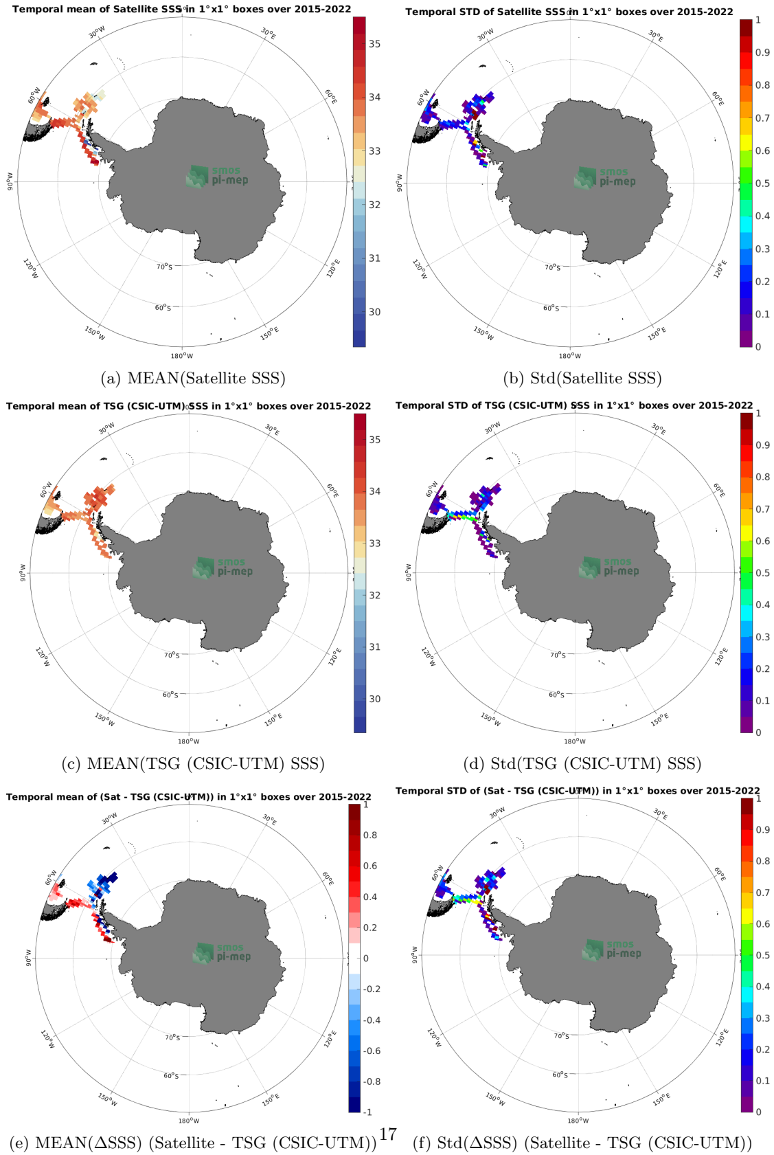
Figure 6: Temporal mean (left) and Std (right) of SSS from SMAP SSS L3 v5 - Monthly (RSS) (top), TSG (CSIC-UTM) (middle), and of \Delta SSS (Satellite - TSG (CSIC-UTM)). Only match-up pairs are used to generate these maps.
