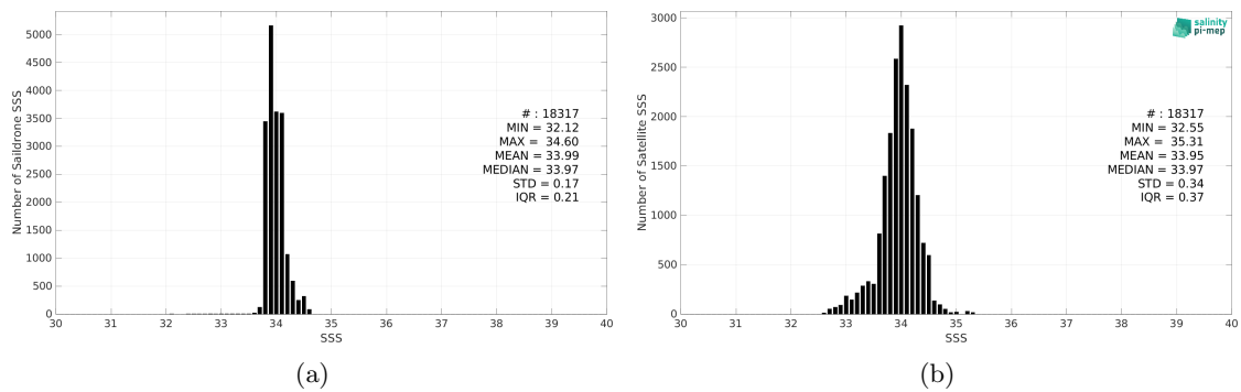
Figure 2: Histograms of SSS from Saildrone (a) and SMAP SSS L3 v5 - Monthly (RSS) (b) considering all match-up pairs per bins of 0.1 over the Southern Ocean Pi-MEP region and for the full satellite product period.
