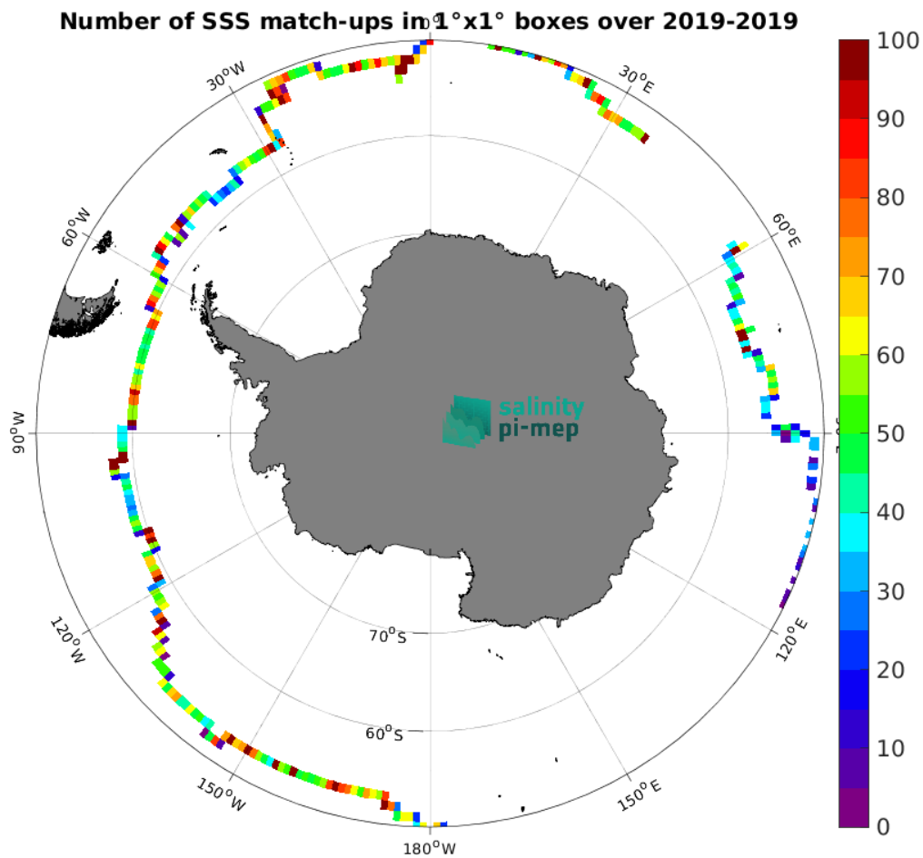
Figure 4: Number of SSS match-ups between Saildrone SSS and the SMAP SSS L3 v5 - Monthly (RSS) SSS product for the Southern Ocean Pi-MEP region over 1^\circ \times 1^\circ boxes and for the full satellite product period.
