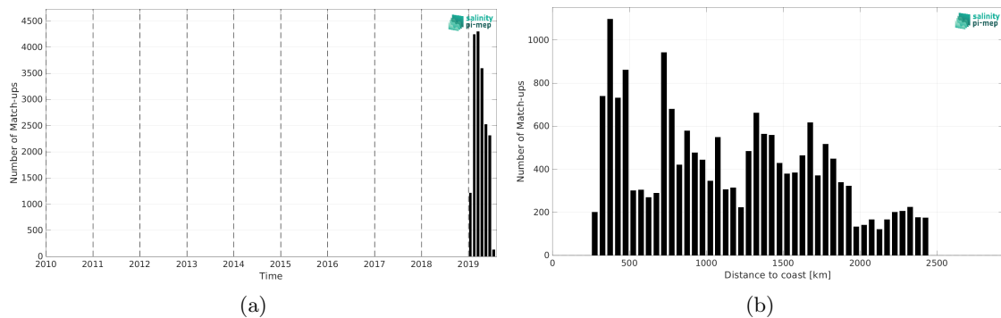
Figure 1: Number of match-ups between Saildrone and SMAP SSS L3 v5 - Monthly (RSS) SSS as a function of time (a) and as function of the distance to coast (b) over the Southern Ocean Pi-MEP region and for the full satellite product period.
