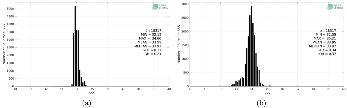
Figure 2: Histograms of SSS from Sairdrone (a) and SMAP SSS L3 v5 - Monthly (RSS) (b) considering all match-up pairs per bins of 0.1 over the Southern Ocean Pi-MEP region and for the full satellite product period.
