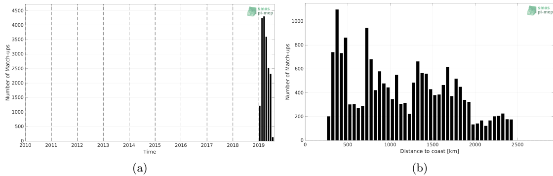
Figure 1: Number of match-ups between Sairdrone and SMAP SSS L3 v5 - Monthly (RSS) SSS as a function of time (a) and as function of the distance to coast (b) over the Southern Ocean Pi-MEP region and for the full satellite product period.
