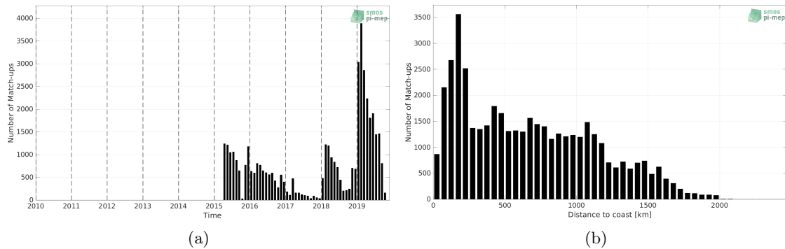
Figure 1: Number of match-ups between Marine mammals and SMAP SSS L3 v5 - Monthly (RSS) SSS as a function of time (a) and as function of the distance to coast (b) over the Southern Ocean Pi-MEP region and for the full satellite product period.
