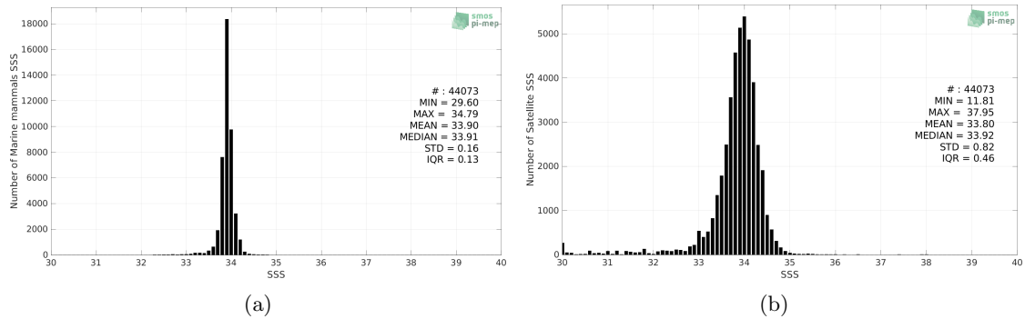
Figure 2: Histograms of SSS from Marine mammals (a) and SMAP SSS L3 v5 - Monthly (RSS) (b) considering all match-up pairs per bins of 0.1 over the Southern Ocean Pi-MEP region and for the full satellite product period.
