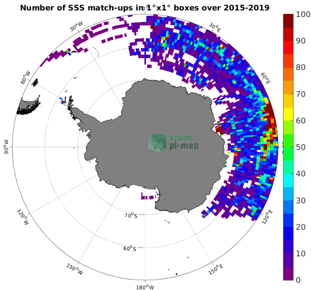
Figure 4: Number of SSS match-ups between Marine mammals SSS and the SMAP SSS L3 v5 - Monthly (RSS) SSS product for the Southern Ocean Pi-MEP region over 1^\circ \times 1^\circ boxes and for the full satellite product period.
