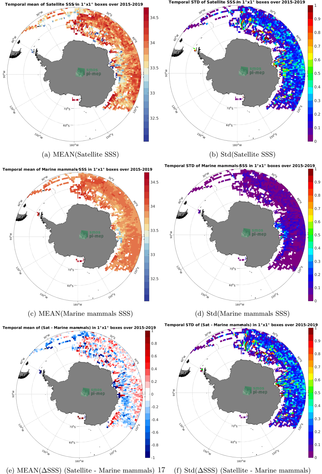
Figure 6: Temporal mean (left) and Std (right) of SSS from SMAP SSS L3 v5 - Monthly (RSS) (top), Marine mammals (middle), and of \Delta SSS (Satellite - Marine mammals). Only match-up pairs are used to generate these maps.
