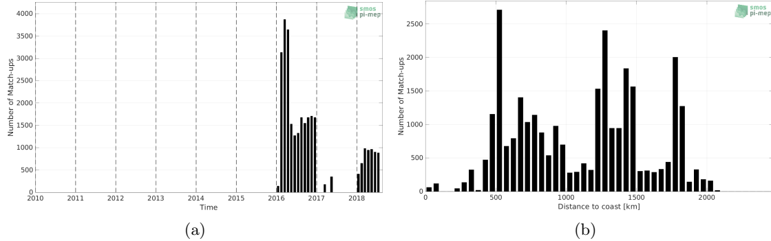
Figure 1: Number of match-ups between Surface drifters and SMAP SSS L3 v5 - Monthly (RSS) SSS as a function of time (a) and as function of the distance to coast (b) over the Southern Ocean Pi-MEP region and for the full satellite product period.
