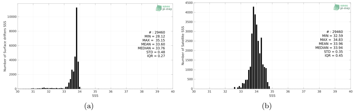
Figure 2: Histograms of SSS from Surface drifters (a) and SMAP SSS L3 v5 - Monthly (RSS) (b) considering all match-up pairs per bins of 0.1 over the Southern Ocean Pi-MEP region and for the full satellite product period.
