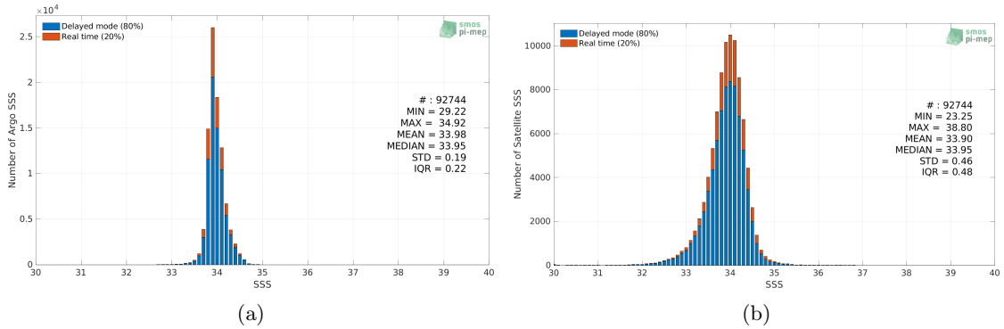
Figure 2: Histograms of SSS from Argo (a) and SMAP SSS L3 v5 - Monthly (RSS) (b) considering all match-up pairs per bins of 0.1 over the Southern Ocean Pi-MEP region and for the full satellite product period.
