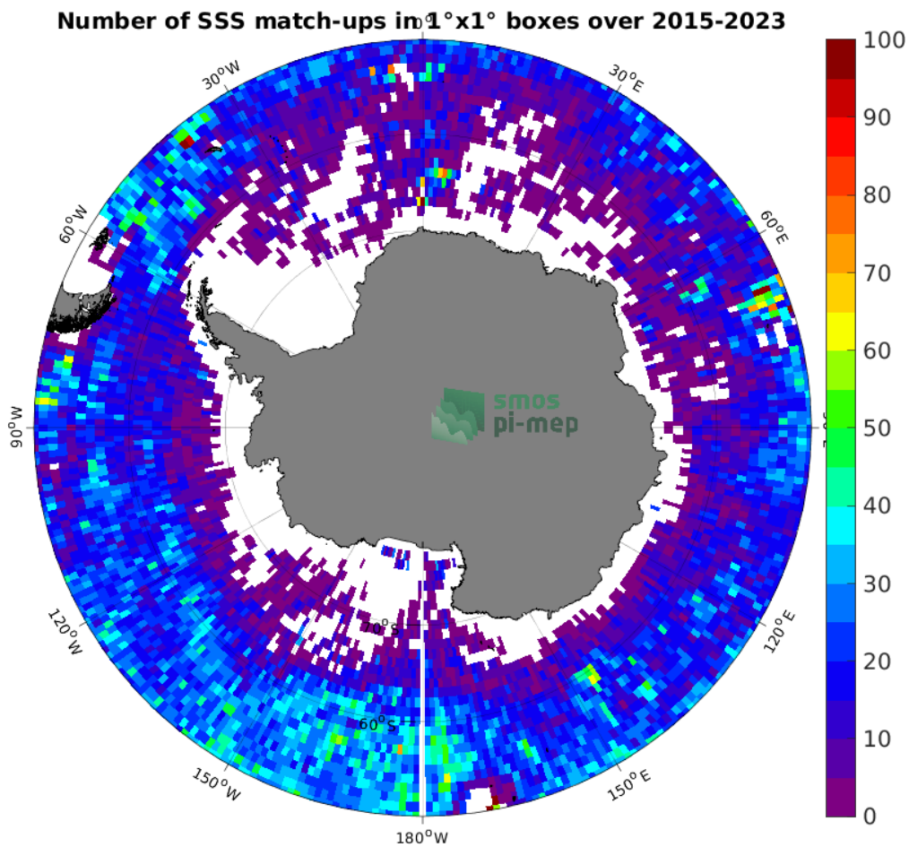
Figure 4: Number of SSS match-ups between Argo SSS and the SMAP SSS L3 v5 - Monthly (RSS) SSS product for the Southern Ocean Pi-MEP region over 1^\circ \times 1^\circ boxes and for the full satellite product period.
