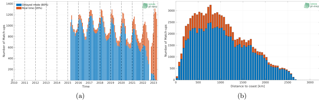
Figure 1: Number of match-ups between Argo and SMAP SSS L3 v5 - Monthly (RSS) SSS as a function of time (a) and as function of the distance to coast (b) over the Southern Ocean Pi-MEP region and for the full satellite product period.
