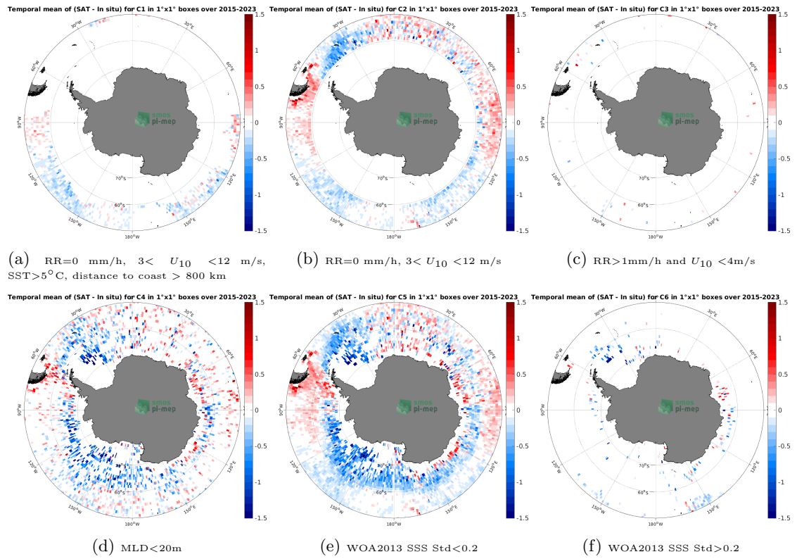
Figure 12: Temporal mean gridded over spatial boxes of size 1^{\circ}\times 1^{\circ} of \Delta\text{SSS} (SMAP SSS L3 v5 - Monthly (RSS) - Argo) for 6 different subdatasets corresponding to:RR=0 mm/h, 3 < U_{10} < 12 m/s, SST > 5^{\circ}\text{C} , distance to coast > 800 km (a), RR=0 mm/h, 3 < U_{10} < 12 m/s (b), RR > 1 mm/h and U_{10} < 4 m/s (c),MLD < 20\text{m} (d),WOA2013 SSS Std < 0.2 (e),WOA2013 SSS Std > 0.2 (f).
