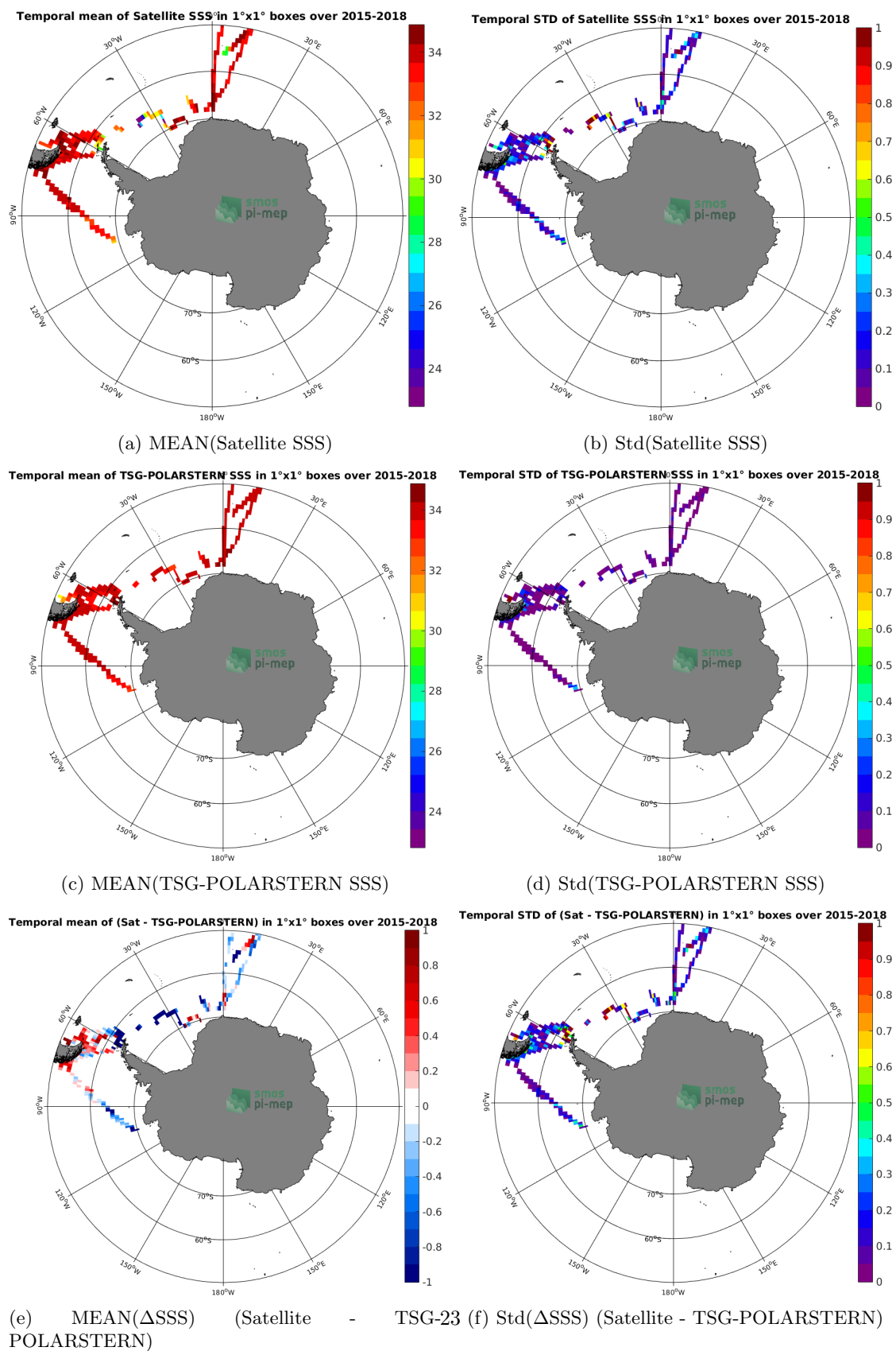
Figure 6: Temporal mean (left) and Std (right) of SSS from SMAP-L3-RSS-V4-8DAY-RUNNING (top), TSG-POLARSTERN (middle), and of \Delta SSS (Satellite - TSG-POLARSTERN). Only match-up pairs are used to generate these maps.
