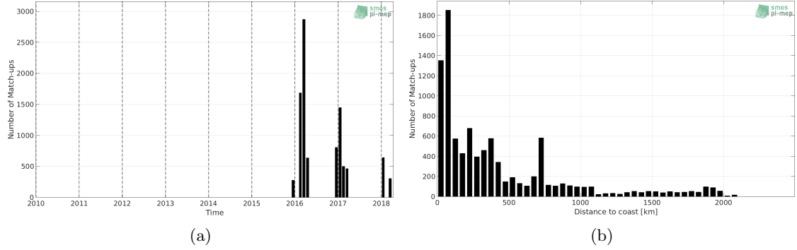
Figure 1: Number of match-ups between TSG-POLARSTERN and SMAP-L3-RSS-V4-8DAY-RUNNING SSS as a function of time (a) and as function of the distance to coast (b) over the Southern Ocean Pi-MEP region and for the full satellite product period.
