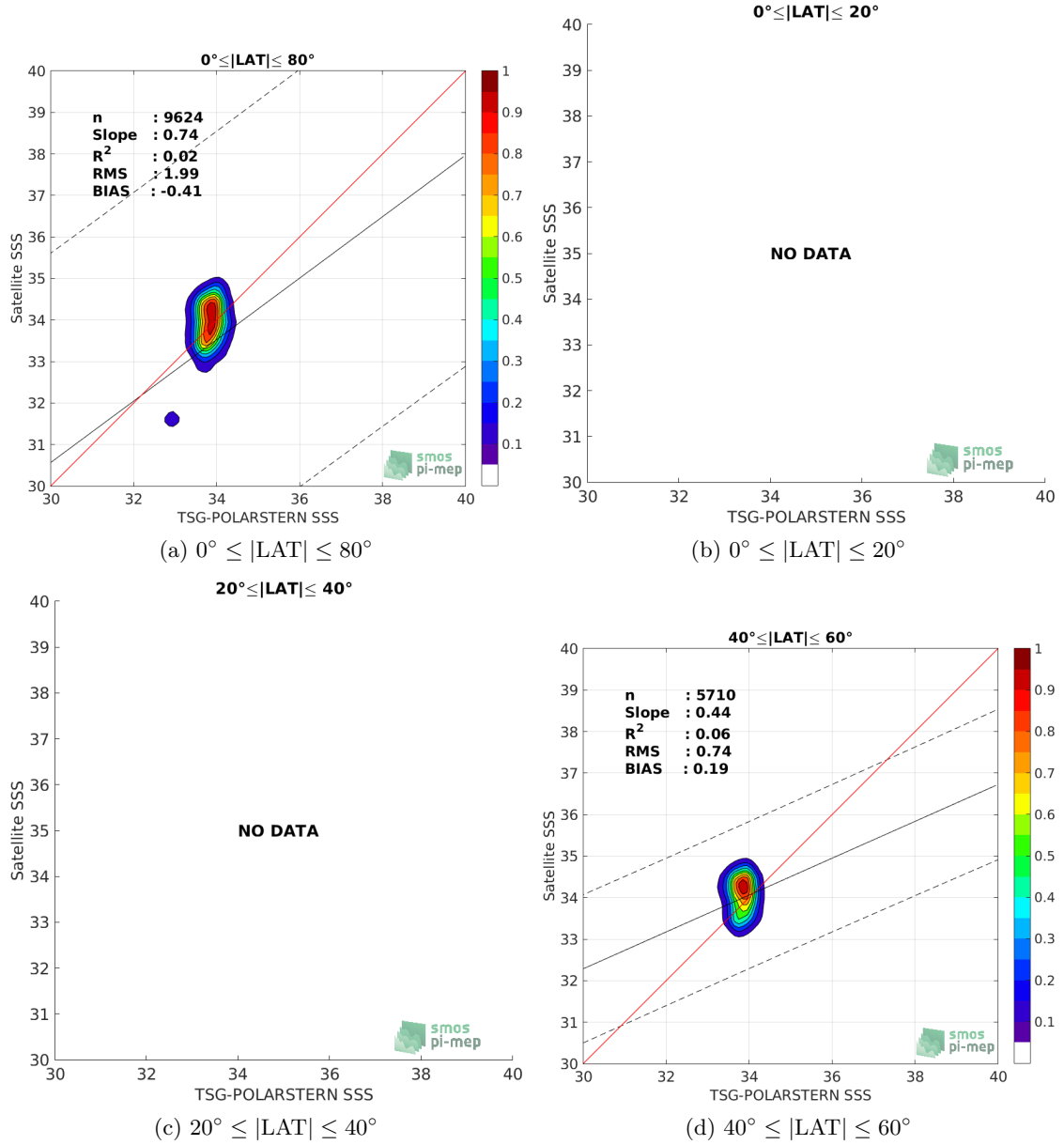
Figure 9: Contour maps of the concentration of SMAP-L3-RSS-V4-8DAY-RUNNING SSS (y-axis) versus TSG-POLARSTERN SSS (x-axis) at match-up pairs for different latitude bands. For each plot, the red line shows x=y . The black thin and dashed lines indicate a linear fit through the data cloud and the \pm 95\% confidence levels, respectively. The number match-up pairs n , the slope and R^2 coefficient of the linear fit, the root mean square (RMS) and the mean bias between satellite and in situ data are indicated for each latitude band in each plots.
