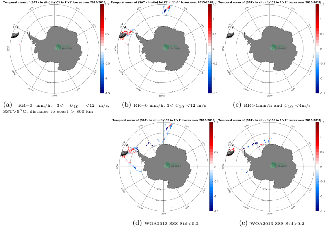
Figure 12: Temporal mean gridded over spatial boxes of size 1^\circ \times 1^\circ of \Delta SSS (SMAP-L3-RSS-V4-8DAY-RUNNING - TSG-POLARSTERN) for 5 different subdatasets corresponding to:RR=0 mm/h, 3 < U_{10} < 12 m/s, SST >5^\circ\text{C} , distance to coast > 800 km (a), RR=0 mm/h, 3 < U_{10} < 12 m/s (b), RR >1 mm/h and U_{10} < 4 m/s (c), WOA2013 SSS Std <0.2 (d), WOA2013 SSS Std >0.2 (e).
