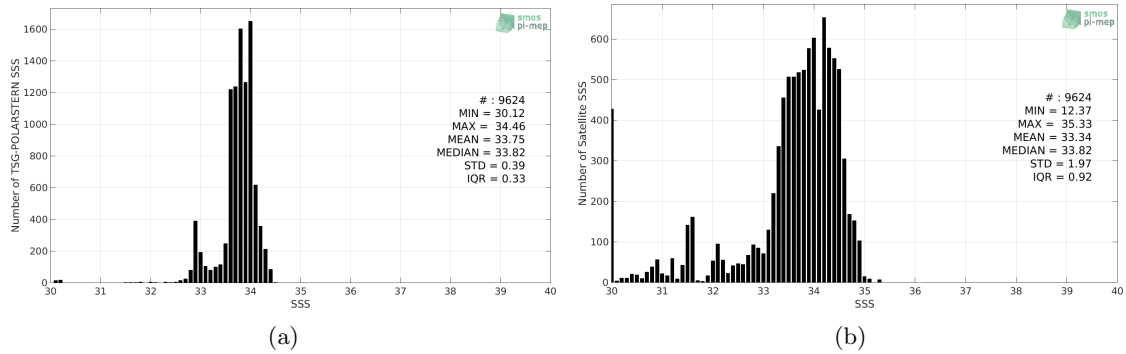
Figure 2: Histograms of SSS from TSG-POLARSTERN (a) and SMAP-L3-RSS-V4-8DAY-RUNNING (b) considering all match-up pairs per bins of 0.1 over the Southern Ocean Pi-MEP region and for the full satellite product period.
