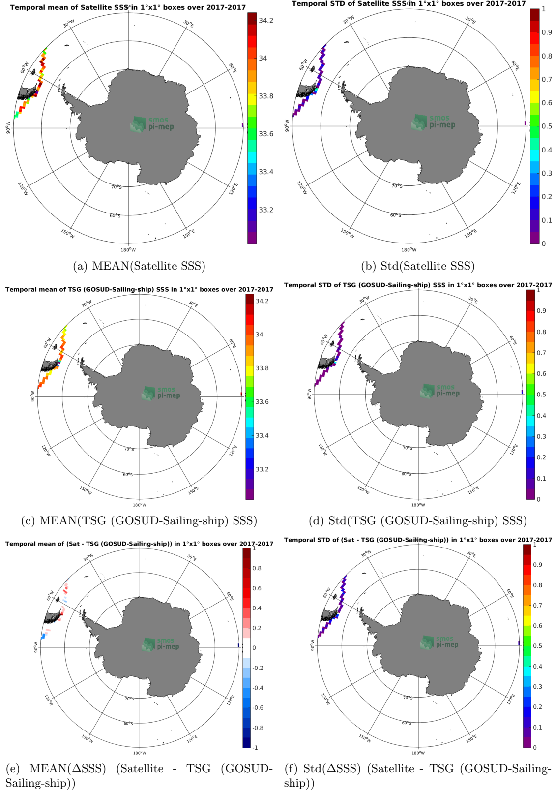
Figure 6: Temporal mean (left) and Std (right), of SSS from SMAP SSS L3 v4 - 8-Day running (RSS) (top), TSG (GOSUD-Sailing-ship) (middle), and of \Delta SSS (Satellite - TSG (GOSUD-Sailing-ship)). Only match-up pairs are used to generate these maps.
