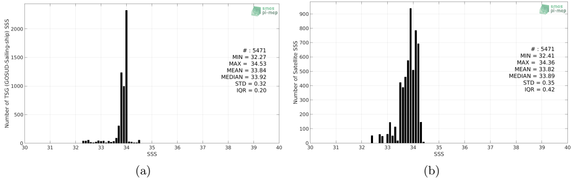
Figure 2: Histograms of SSS from TSG (GOSUD-Sailing-ship) (a) and SMAP SSS L3 v4 - 8-Day running (RSS) (b) considering all match-up pairs per bins of 0.1 over the Southern Ocean Pi-MEP region and for the full satellite product period.
