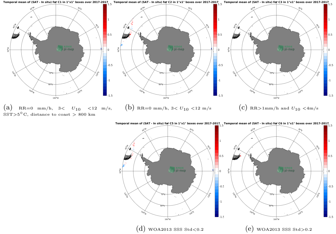
Figure 12: Temporal mean gridded over spatial boxes of size 1°x1° of \Delta SSS (SMAP SSS L3 v4 - 8-Day running (RSS) - TSG (GOSUD-Sailing-ship)) for 5 different subdatasets corresponding to: RR=0 mm/h, 3 < U_{10} < 12 m/s, SST>5°C, distance to coast > 800 km (a), RR=0 mm/h, 3 < U_{10} < 12 m/s (b), RR>1 mm/h and U_{10} < 4 m/s (c), WOA2013 SSS Std<0.2 (d), WOA2013 SSS Std>0.2 (e).
