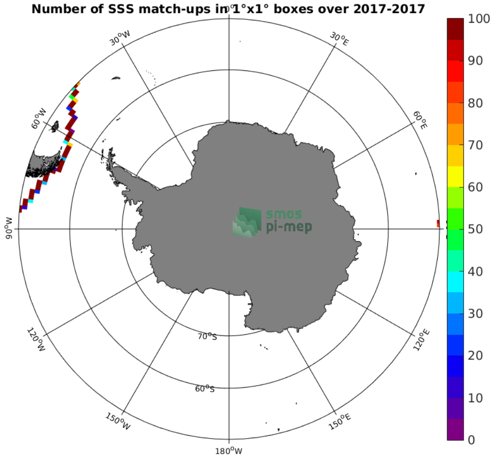
Figure 4: Number of SSS match-ups between TSG (GOSUD-Sailing-ship) SSS and the SMAP SSS L3 v4 - 8-Day running (RSS) SSS product for the Southern Ocean Pi-MEP region over 1^\circ \times 1^\circ boxes and for the full satellite product period.
