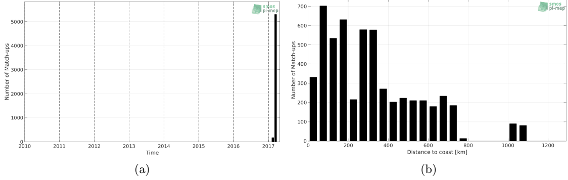
Figure 1: Number of match-ups between TSG (GOSUD-Sailing-ship) and SMAP SSS L3 v4 - 8-Day running (RSS) SSS as a function of time (a) and as function of the distance to coast (b) over the Southern Ocean Pi-MEP region and for the full satellite product period.
