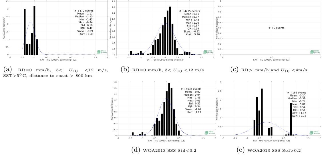
Figure 13: Normalized histogram of \Delta SSS (SMAP SSS L3 v4 - 8-Day running (RSS) - TSG (GOSUD-Sailing-ship)) for 5 different subdatasets corresponding to: RR=0 mm/h, 3 < U_{10} < 12 m/s, SST > 5^\circ\text{C} , distance to coast > 800 km (a), RR=0 mm/h, 3 < U_{10} < 12 m/s (b), RR > 1\text{mm/h} and U_{10} < 4\text{m/s} (c), WOA2013 SSS Std < 0.2 (d), WOA2013 SSS Std > 0.2 (e).
