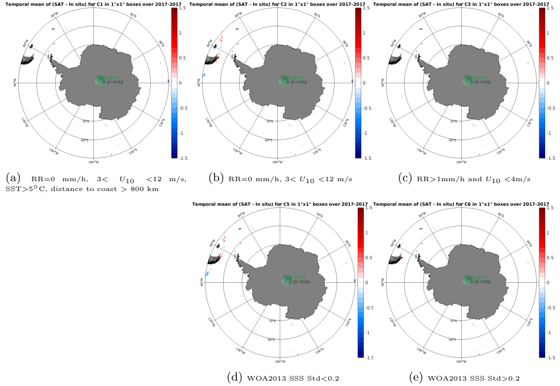
Figure 12: Temporal mean gridded over spatial boxes of size 1°x1° of \Delta\text{SSS} (SMAP SSS L3 v4 - 8-Day running (RSS) - TSG (GOSUD-Sailing-ship)) for 5 different subdatasets corresponding to: RR=0 mm/h, 3 < U_{10} < 12 m/s, SST > 5^\circ\text{C} , distance to coast > 800 km (a), RR=0 mm/h, 3 < U_{10} < 12 m/s (b), RR > 1 mm/h and U_{10} < 4 m/s (c), WOA2013 SSS Std < 0.2 (d), WOA2013 SSS Std > 0.2 (e).
