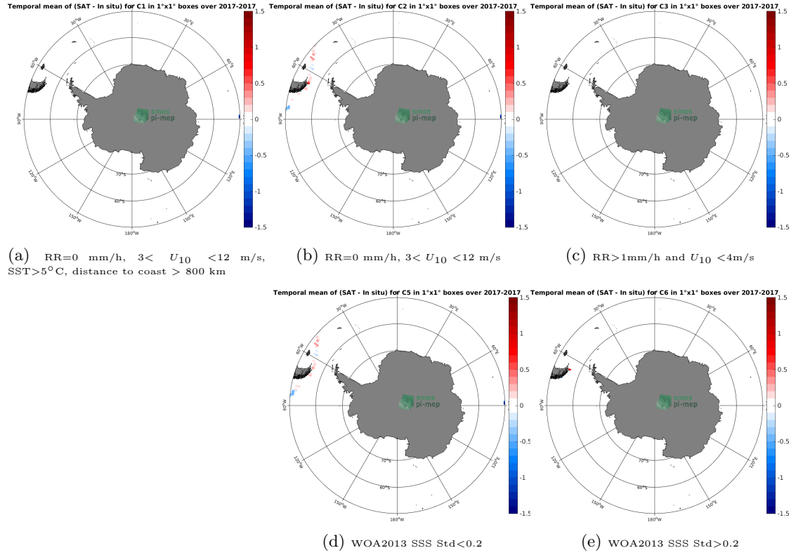
Figure 12: Temporal mean gridded over spatial boxes of size 1°x1° of \Delta\text{SSS} (SMAP-L3-RSS-V4-8DAY-RUNNING - TSG-GOSUD-Sailing-ship) for 5 different subdatasets corresponding to: RR=0 mm/h, 3 < U_{10} < 12 m/s, SST > 5^{\circ}\text{C} , distance to coast > 800 km (a), RR=0 mm/h, 3 < U_{10} < 12 m/s (b), RR > 1 mm/h and U_{10} < 4 m/s (c), WOA2013 SSS Std < 0.2 (d), WOA2013 SSS Std > 0.2 (e).
