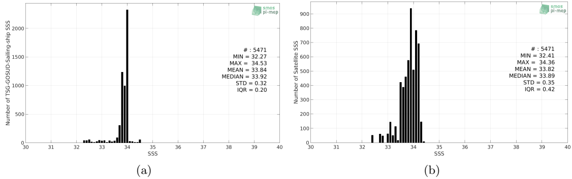
Figure 2: Histograms of SSS from TSG-GOSUD-Sailing-ship (a) and SMAP-L3-RSS-V4-8DAY-RUNNING (b) considering all match-up pairs per bins of 0.1 over the Southern Ocean Pi-MEP region and for the full satellite product period.
