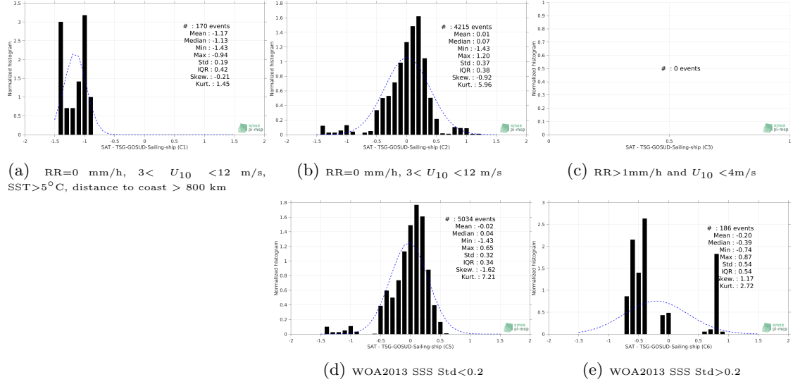
Figure 13: Normalized histogram of \Delta SSS (SMAP-L3-RSS-V4-8DAY-RUNNING - TSG-GOSUD-Sailing-ship) for 5 different subdatasets corresponding to: RR=0 mm/h, 3 < U_{10} < 12 m/s, SST>5°C, distance to coast > 800 km (a), RR=0 mm/h, 3 < U_{10} < 12 m/s (b), RR>1 mm/h and U_{10} < 4 m/s (c), WOA2013 SSS Std<0.2 (d), WOA2013 SSS Std>0.2 (e).
