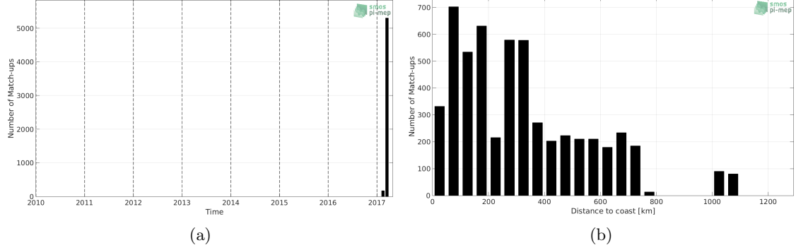
Figure 1: Number of match-ups between TSG-GOSUD-Sailing-ship and SMAP-L3-RSS-V4-8DAY-RUNNING SSS as a function of time (a) and as function of the distance to coast (b) over the Southern Ocean Pi-MEP region and for the full satellite product period.
