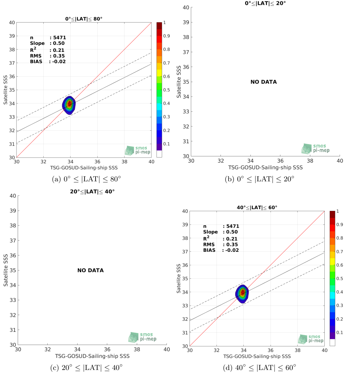
Figure 9: Contour maps of the concentration of SMAP-L3-RSS-V4-8DAY-RUNNING SSS (y-axis) versus TSG-GOSUD-Sailing-ship SSS (x-axis) at match-up pairs for different latitude bands. For each plot, the red line shows x=y . The black thin and dashed lines indicate a linear fit through the data cloud and the \pm 95\% confidence levels, respectively. The number match-up pairs n , the slope and R^2 coefficient of the linear fit, the root mean square (RMS) and the mean bias between satellite and in situ data are indicated for each latitude band in each plots.
