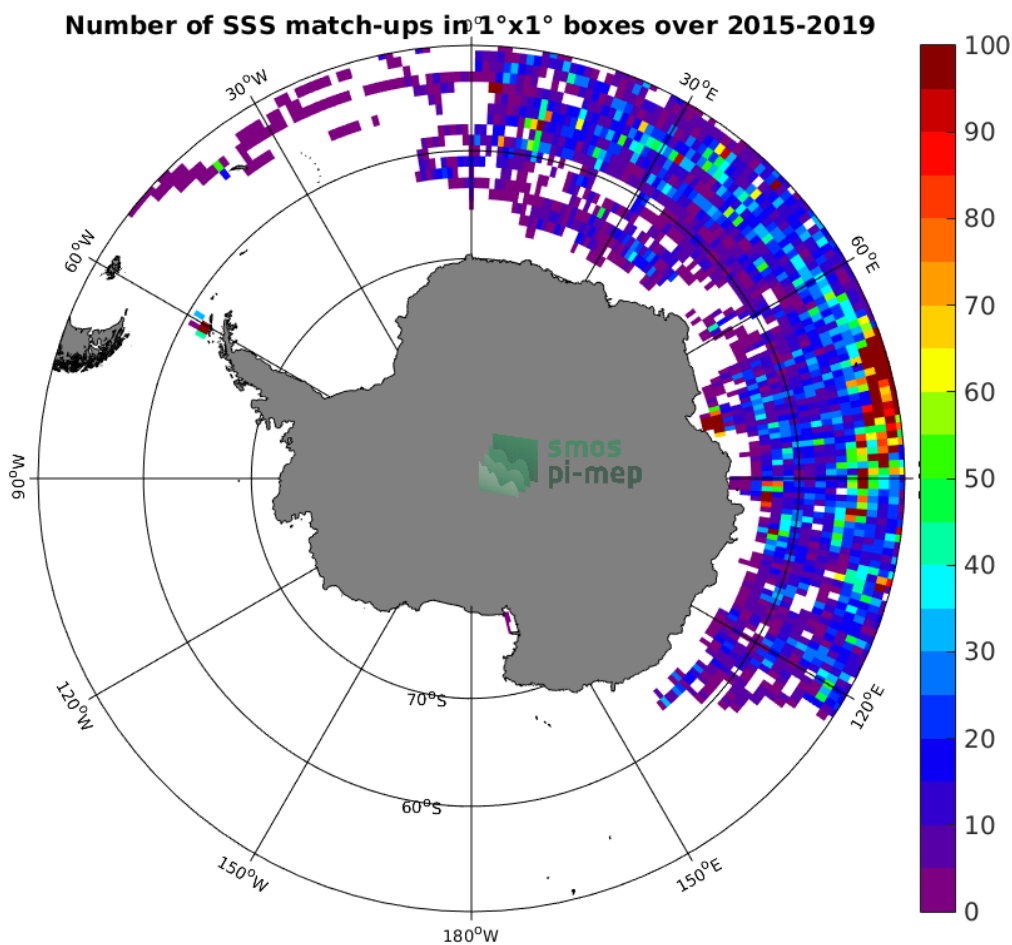
Figure 4: Number of SSS match-ups between Marine mammals SSS and the SMAP SSS L3 v4 - 8-Day running (RSS) SSS product for the Southern Ocean Pi-MEP region over 1^\circ \times 1^\circ boxes and for the full satellite product period.
