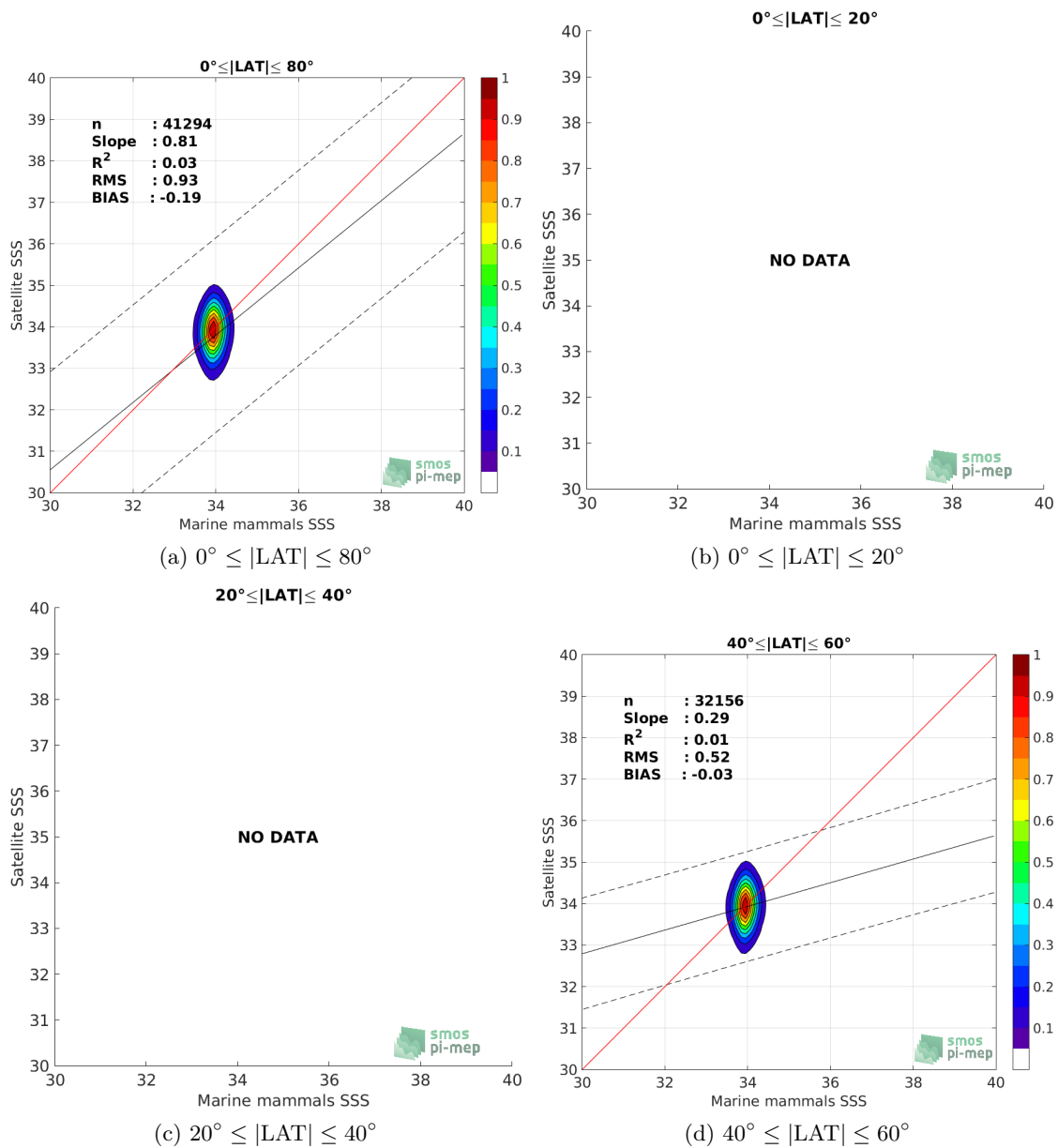
Figure 9: Contour maps of the concentration of SMAP SSS L3 v4 - 8-Day running (RSS) SSS (y-axis) versus Marine mammals SSS (x-axis) at match-up pairs for different latitude bands. For each plot, the red line shows x=y . The black thin and dashed lines indicate a linear fit through the data cloud and the \pm 95\% confidence levels, respectively. The number match-up pairs n , the slope and R^2 coefficient of the linear fit, the root mean square (RMS) and the mean bias between satellite and in situ data are indicated for each latitude band in each plots.
