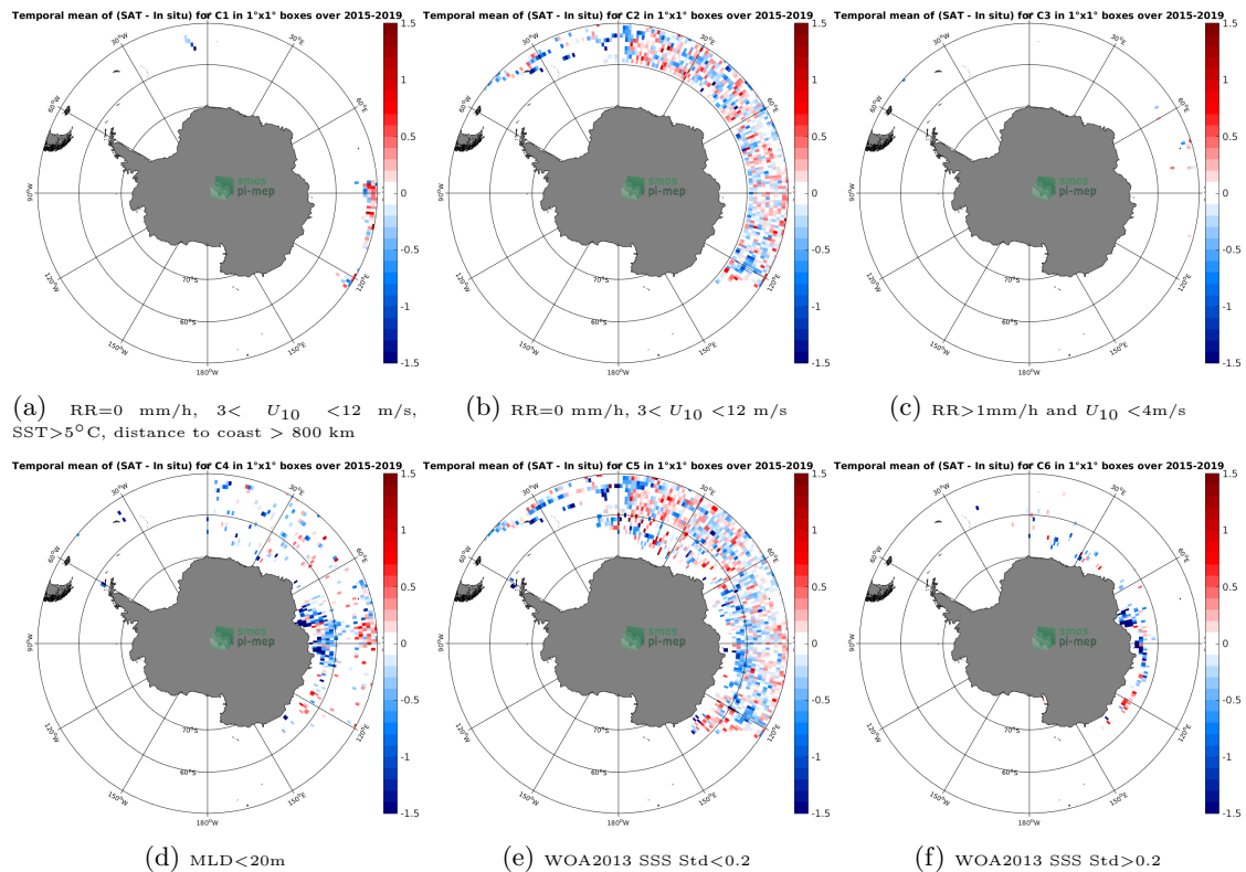
Figure 12: Temporal mean gridded over spatial boxes of size 1^{\circ}\times 1^{\circ} of \Delta\text{SSS} (SMAP SSS L3 v4 - 8-Day running (RSS) - Marine mammals) for 6 different subdatasets corresponding to:RR=0 mm/h, 3 < U_{10} < 12 m/s, SST >5^{\circ}\text{C} , distance to coast > 800 km (a), RR=0 mm/h, 3 < U_{10} < 12 m/s (b), RR >1 mm/h and U_{10} < 4 m/s (c),MLD <20 m (d),WOA2013 SSS Std <0.2 (e),WOA2013 SSS Std >0.2 (f).
