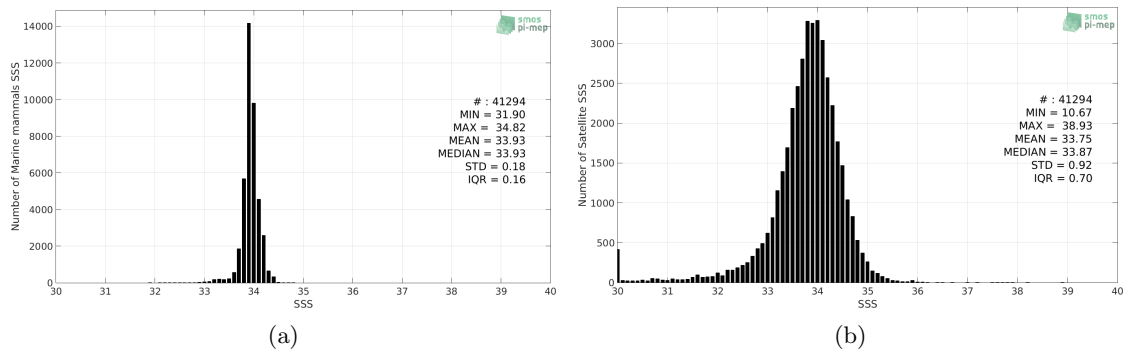
Figure 2: Histograms of SSS from Marine mammals (a) and SMAP SSS L3 v4 - 8-Day running (RSS) (b) considering all match-up pairs per bins of 0.1 over the Southern Ocean Pi-MEP region and for the full satellite product period.
