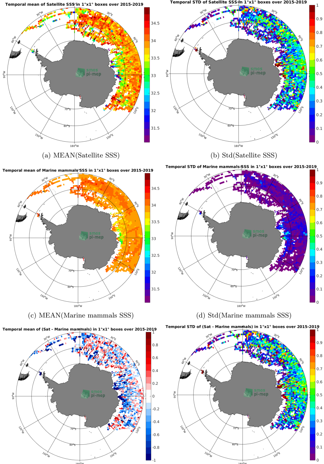
Figure 6: Temporal mean (left) and Std (right) of SSS from SMAP SSS L3 v4 - 8-Day running (RSS) (top), Marine mammals (middle), and of \Delta SSS (Satellite - Marine mammals). Only match-up pairs are used to generate these maps.
