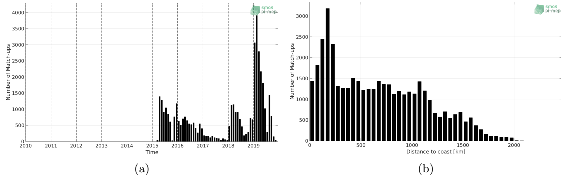
Figure 1: Number of match-ups between Marine mammals and SMAP SSS L3 v4 - 8-Day running (RSS) SSS as a function of time (a) and as function of the distance to coast (b) over the Southern Ocean Pi-MEP region and for the full satellite product period.
