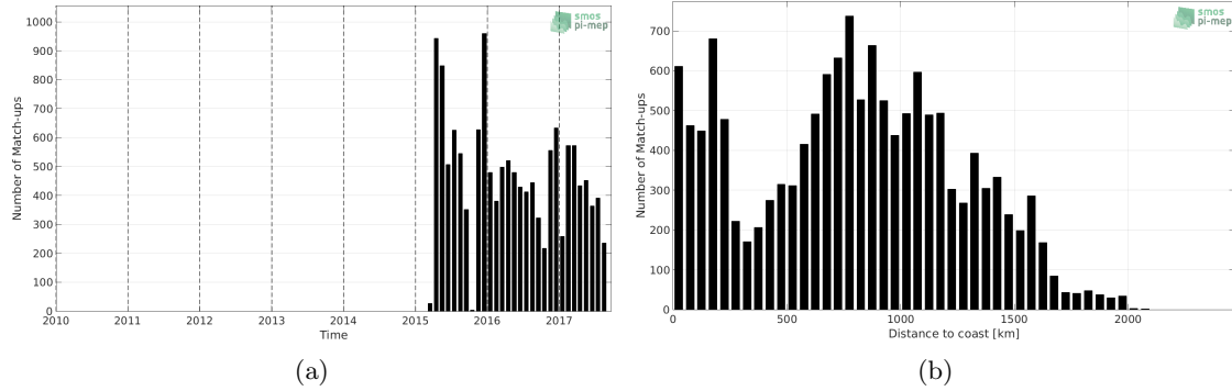
Figure 1: Number of match-ups between Sea mammals and SMAP-L3-RSS-V4-8DAY-RUNNING SSS as a function of time (a) and as function of the distance to coast (b) over the Southern Ocean Pi-MEP region and for the full satellite product period.
