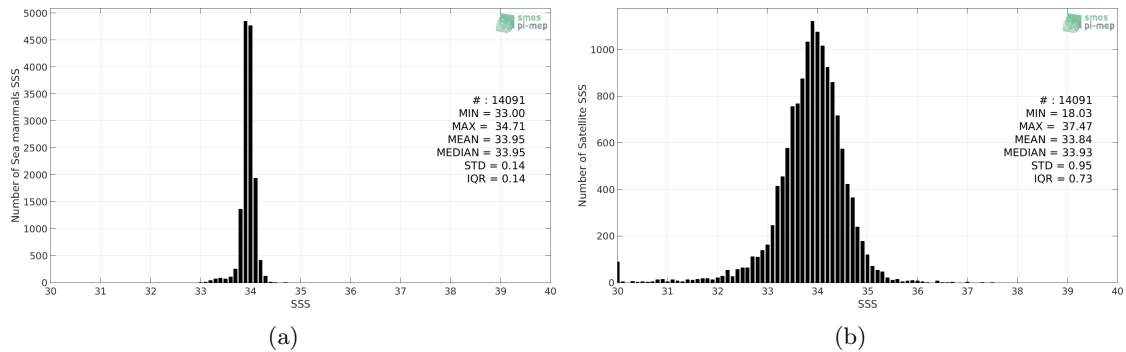
Figure 2: Histograms of SSS from Sea mammals (a) and SMAP-L3-RSS-V4-8DAY-RUNNING (b) considering all match-up pairs per bins of 0.1 over the Southern Ocean Pi-MEP region and for the full satellite product period.
