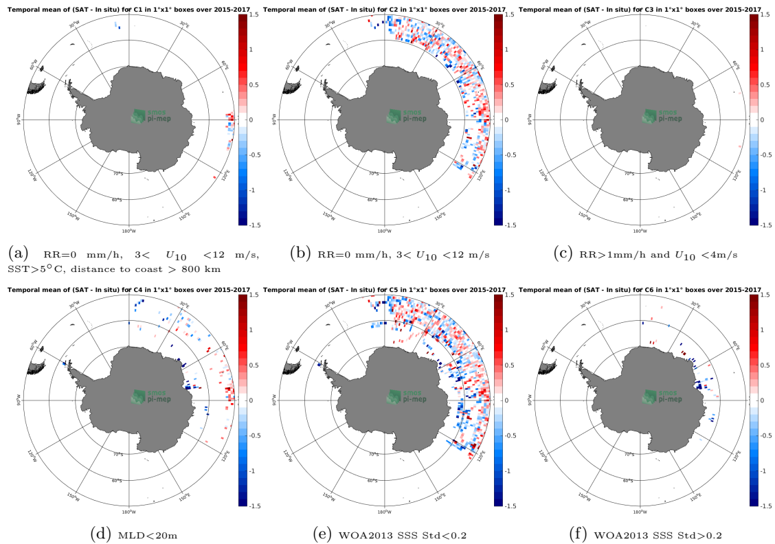
Figure 12: Temporal mean gridded over spatial boxes of size 1^{\circ}\times 1^{\circ} of \Delta\text{SSS} (SMAP-L3-RSS-V4-8DAY-RUNNING - Sea mammals) for 6 different subdatasets corresponding to:RR=0 mm/h, 3 < U_{10} < 12 m/s, SST > 5^{\circ}\text{C} , distance to coast > 800 km (a), RR=0 mm/h, 3 < U_{10} < 12 m/s (b), RR > 1\text{mm/h} and U_{10} < 4\text{m/s} (c),MLD < 20\text{m} (d),WOA2013 SSS Std < 0.2 (e),WOA2013 SSS Std > 0.2 (f).
