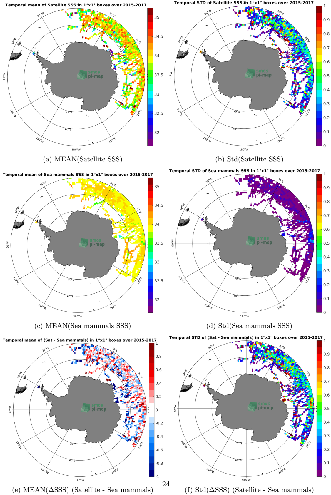
Figure 6: Temporal mean (left) and Std (right) of SSS from SMAP-L3-RSS-V4-8DAY-RUNNING (top), Sea mammals (middle), and of \Delta SSS (Satellite - Sea mammals). Only match-up pairs are used to generate these maps.
