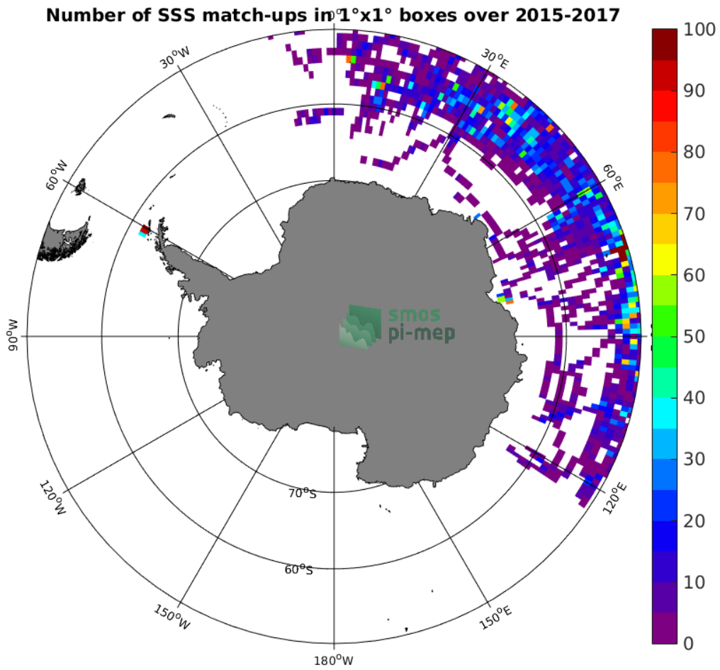
Figure 4: Number of SSS match-ups between Sea mammals SSS and the SMAP-L3-RSS-V4-8DAY-RUNNING SSS product for the Southern Ocean Pi-MEP region over 1°x1° boxes and for the full satellite product period.
