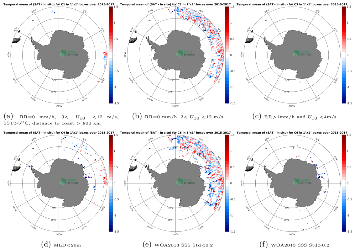
Figure 12: Temporal mean gridded over spatial boxes of size 1^\circ \times 1^\circ of \Delta SSS (SMAP-L3-RSS-V4-8DAY-RUNNING - Sea mammals) for 6 different subdatasets corresponding to:RR=0 mm/h, 3 < U_{10} < 12 m/s, SST >5^\circ C, distance to coast > 800 km (a), RR=0 mm/h, 3 < U_{10} < 12 m/s (b), RR >1 mm/h and U_{10} < 4 m/s (c),MLD <20 m (d),WOA2013 SSS Std <0.2 (e),WOA2013 SSS Std >0.2 (f).
