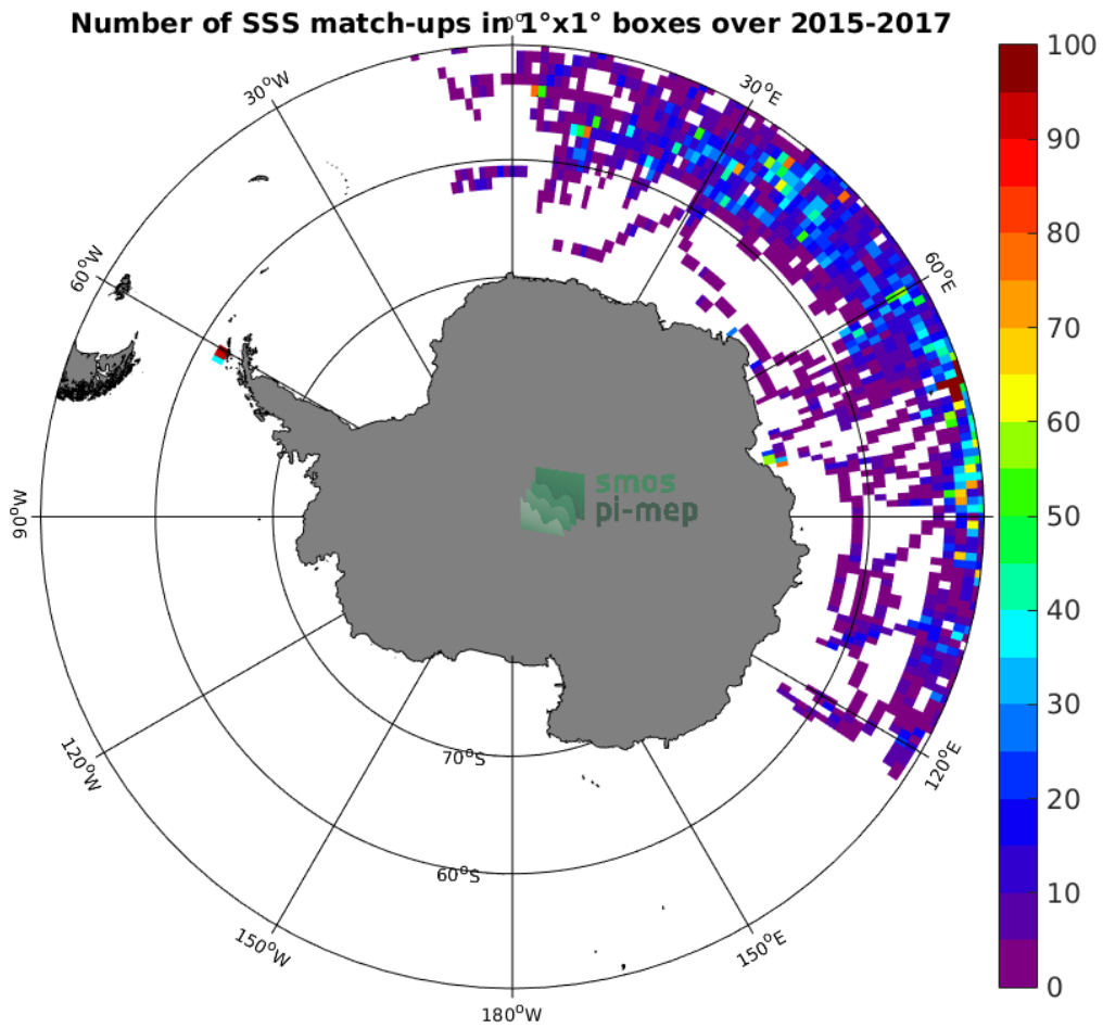
Figure 4: Number of SSS match-ups between Sea mammals SSS and the SMAP-L3-RSS-V4-8DAY-RUNNING SSS product for the Southern Ocean Pi-MEP region over 1^\circ \times 1^\circ boxes and for the full satellite product period.
