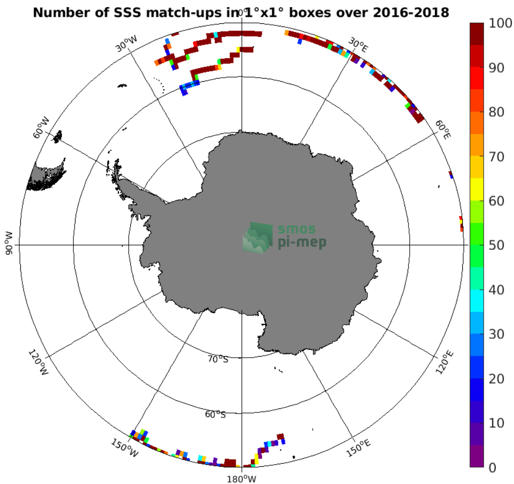
Figure 3: Number of SSS match-ups between Surface drifters SSS and the SMAP SSS L3 v4 - 8-Day running (RSS) SSS product for the Southern Ocean Pi-MEP region over 1^\circ \times 1^\circ boxes and for the full satellite product period.
