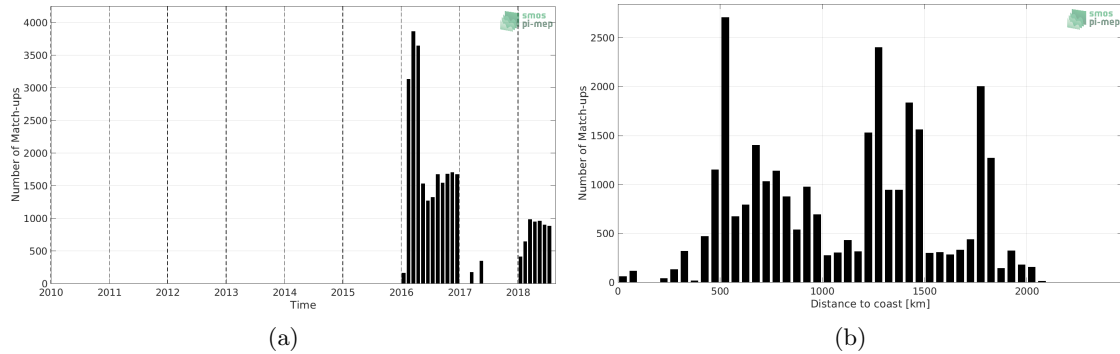
Figure 1: Number of match-ups between Surface drifters and SMAP SSS L3 v4 - 8-Day running (RSS) SSS as a function of time (a) and as function of the distance to coast (b) over the Southern Ocean Pi-MEP region and for the full satellite product period.
