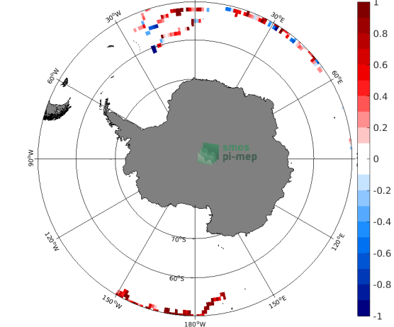
(e) MEAN( \Delta SSS) (Satellite - Surface drifters)
