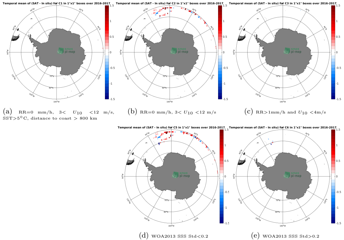
Figure 11: Temporal mean gridded over spatial boxes of size 1^\circ \times 1^\circ of \Delta SSS (SMAP-L3-RSS-V4-8DAY-RUNNING - Surface drifters) for 5 different subdatasets corresponding to:RR=0 mm/h, 3 < U_{10} < 12 m/s, SST >5^\circ C, distance to coast > 800 km (a), RR=0 mm/h, 3 < U_{10} < 12 m/s (b), RR >1 mm/h and U_{10} < 4 m/s (c), WOA2013 SSS Std <0.2 (d), WOA2013 SSS Std >0.2 (e).
