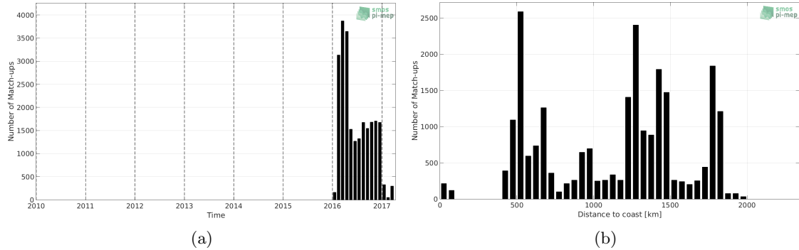
Figure 1: Number of match-ups between Surface drifters and SMAP-L3-RSS-V4-8DAY-RUNNING SSS as a function of time (a) and as function of the distance to coast (b) over the Southern Ocean Pi-MEP region and for the full satellite product period.
