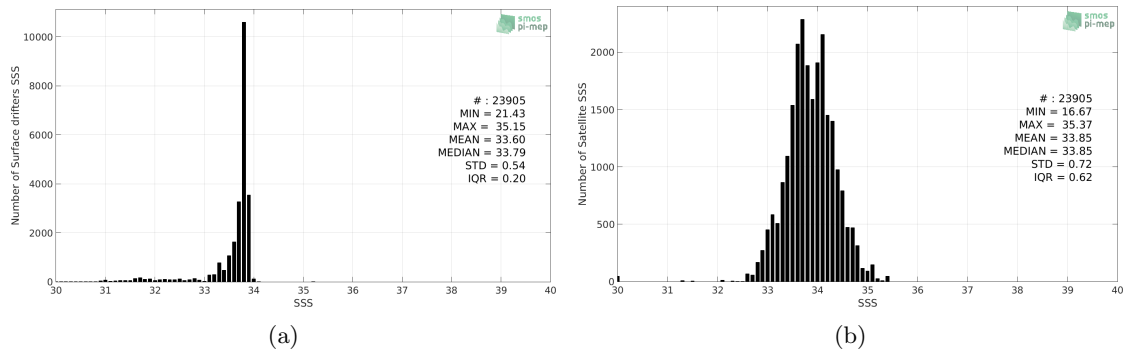
Figure 2: Histograms of SSS from Surface drifters (a) and SMAP-L3-RSS-V4-8DAY-RUNNING (b) considering all match-up pairs per bins of 0.1 over the Southern Ocean Pi-MEP region and for the full satellite product period.
