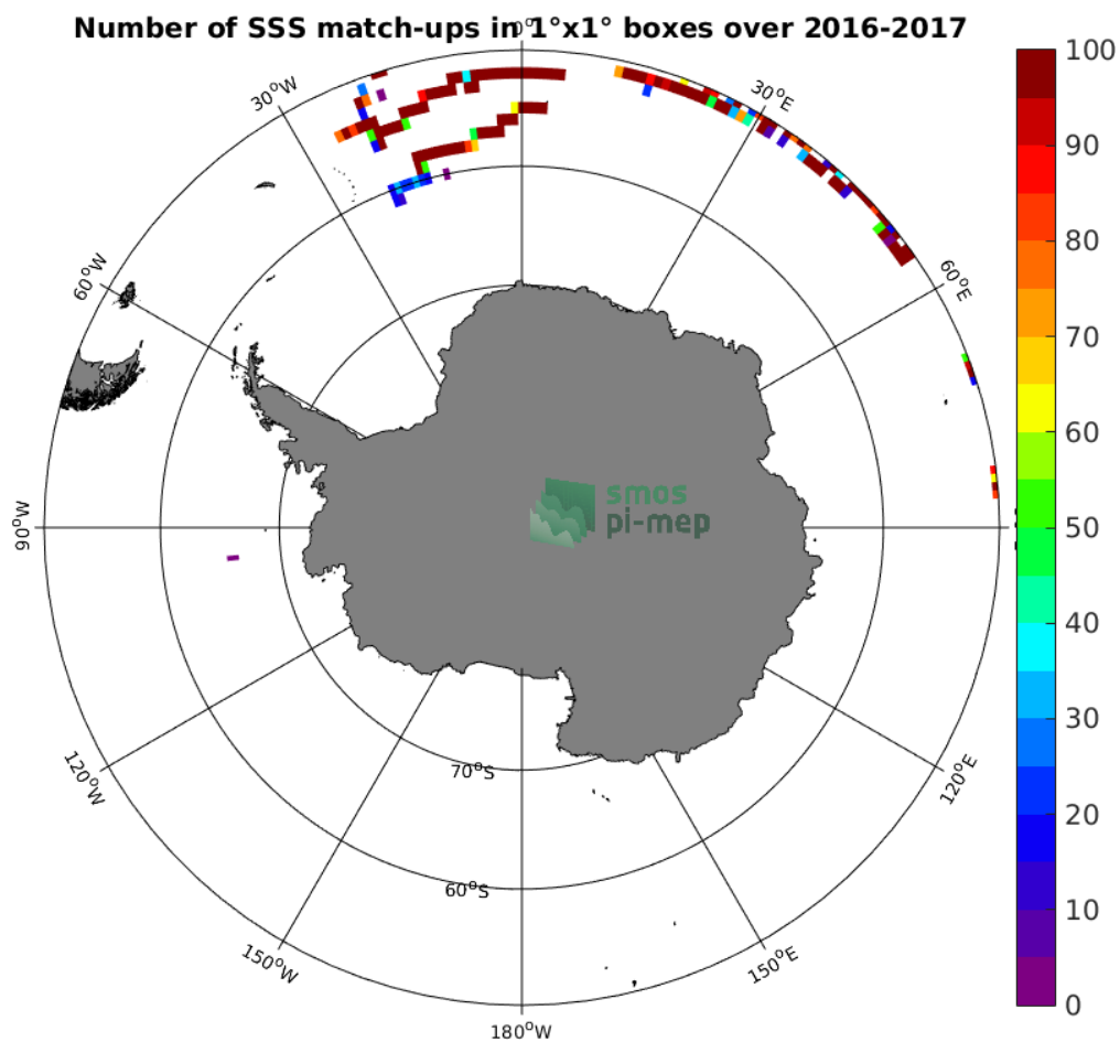
Figure 3: Number of SSS match-ups between Surface drifters SSS and the SMAP-L3-RSS-V4-8DAY-RUNNING SSS product for the Southern Ocean Pi-MEP region over 1^\circ \times 1^\circ boxes and for the full satellite product period.
