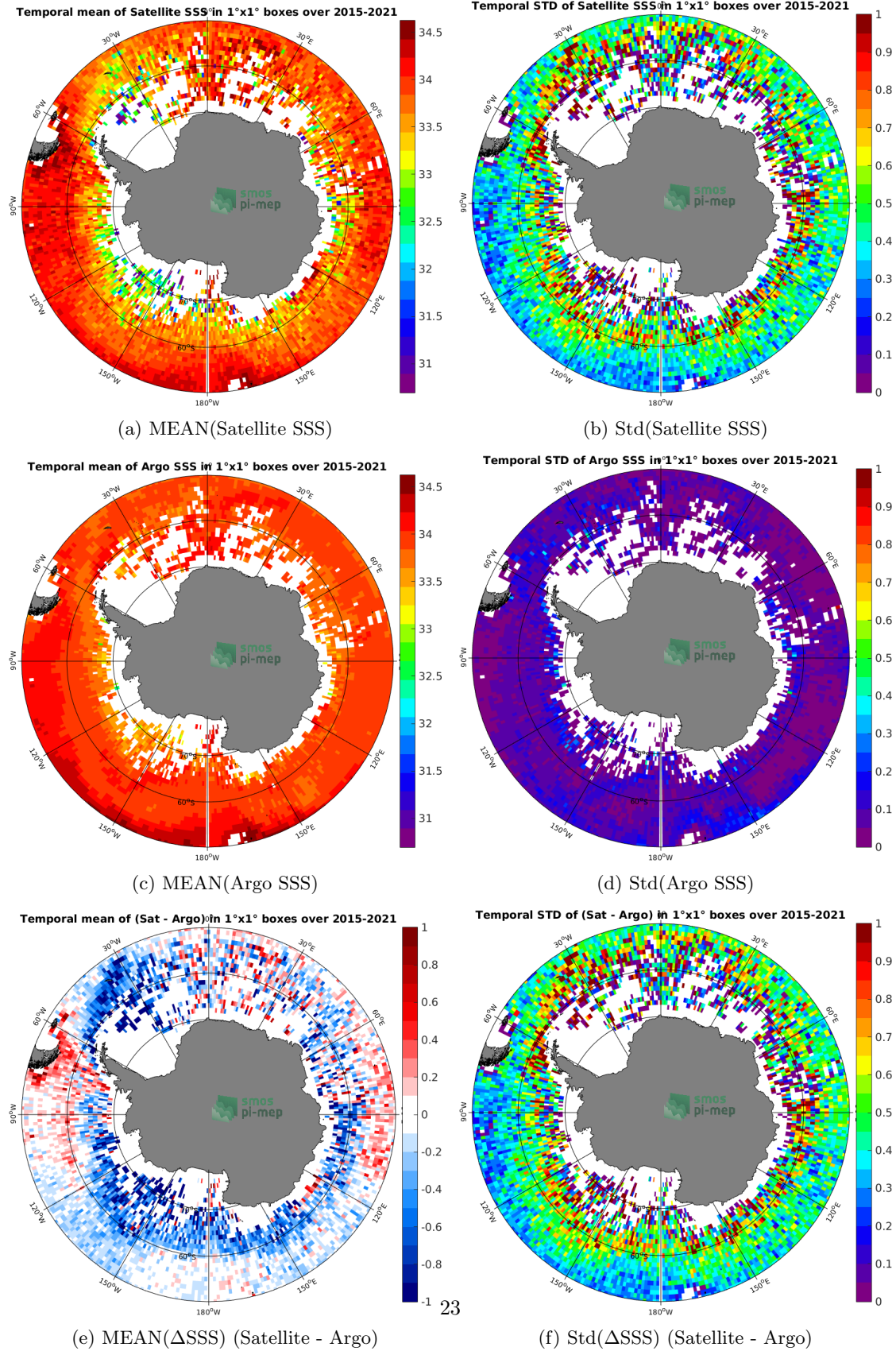
Figure 6: Temporal mean (left) and Std (right) of SSS from SMAP SSS L3 v4 - 8-Day running (RSS) (top), Argo (middle), and of \Delta SSS (Satellite - Argo). Only match-up pairs are used to generate these maps.
