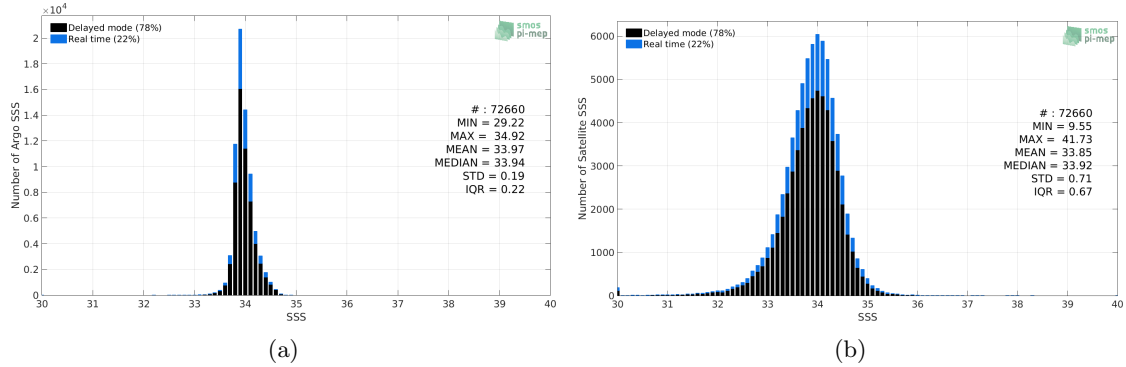
Figure 2: Histograms of SSS from Argo (a) and SMAP SSS L3 v4 - 8-Day running (RSS) (b) considering all match-up pairs per bins of 0.1 over the Southern Ocean Pi-MEP region and for the full satellite product period.
