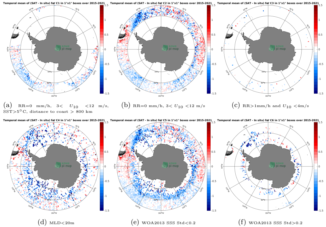
Figure 12: Temporal mean gridded over spatial boxes of size 1^{\circ} \times 1^{\circ} of \Delta\text{SSS} (SMAP SSS L3 v4 - 8-Day running (RSS) - Argo) for 6 different subdatasets corresponding to: \text{RR}=0 mm/h, 3 < U_{10} < 12 m/s, \text{SST} > 5^{\circ}\text{C} , distance to coast > 800 km (a), \text{RR}=0 mm/h, 3 < U_{10} < 12 m/s (b), \text{RR} > 1 mm/h and U_{10} < 4 m/s (c), \text{MLD} < 20\text{m} (d), \text{WOA2013 SSS Std} < 0.2 (e), \text{WOA2013 SSS Std} > 0.2 (f).
