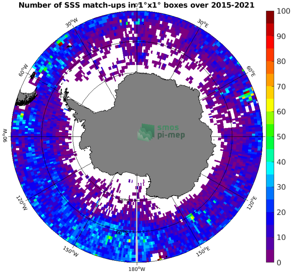
Figure 4: Number of SSS match-ups between Argo SSS and the SMAP SSS L3 v4 - 8-Day running (RSS) SSS product for the Southern Ocean Pi-MEP region over 1^\circ \times 1^\circ boxes and for the full satellite product period.
