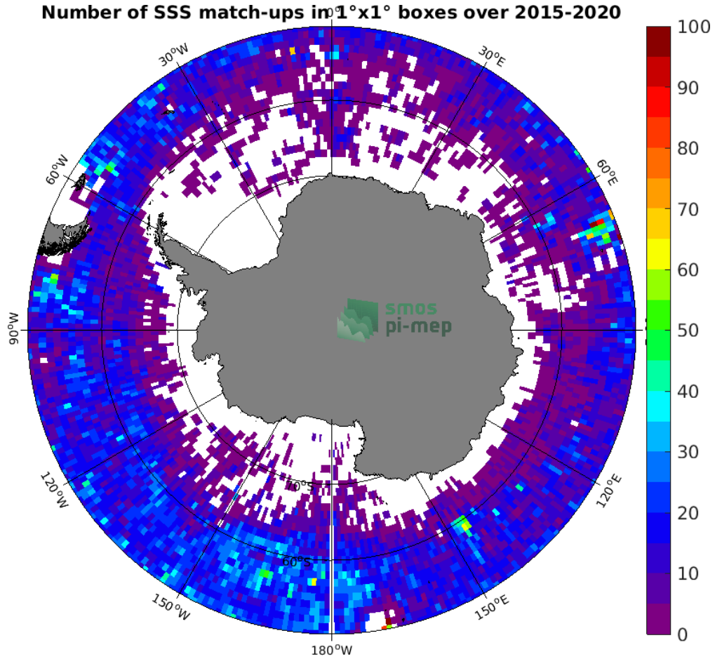
Figure 4: Number of SSS match-ups between Argo SSS and the SMAP SSS L3 v4 - 8-Day running (RSS) SSS product for the Southern Ocean Pi-MEP region over 1^\circ \times 1^\circ boxes and for the full satellite product period.
