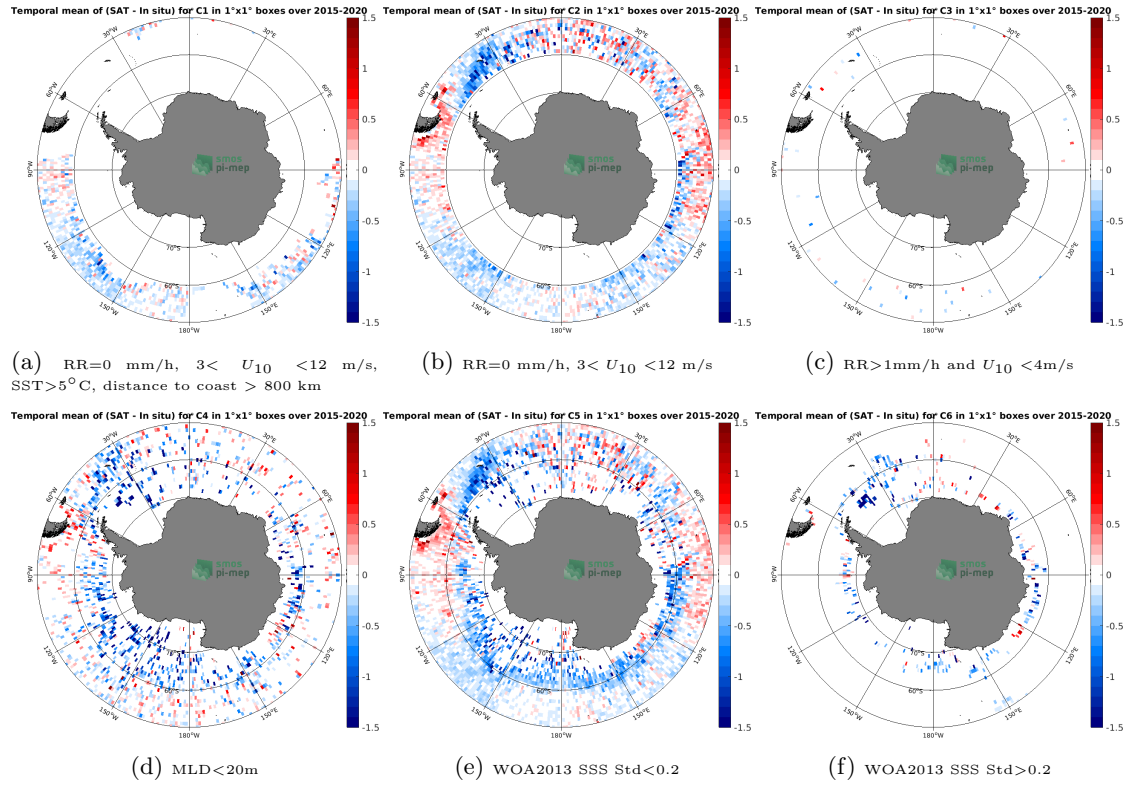
Figure 12: Temporal mean gridded over spatial boxes of size 1^{\circ}\times 1^{\circ} of \Delta\text{SSS} (SMAP SSS L3 v4 - 8-Day running (RSS) - Argo) for 6 different subdatasets corresponding to:RR=0 mm/h, 3 < U_{10} < 12 m/s, SST >5^{\circ}\text{C} , distance to coast > 800 km (a), RR=0 mm/h, 3 < U_{10} < 12 m/s (b), RR >1\text{mm/h} and U_{10} < 4\text{m/s} (c),MLD <20\text{m} (d),WOA2013 SSS Std <0.2 (e),WOA2013 SSS Std >0.2 (f).
