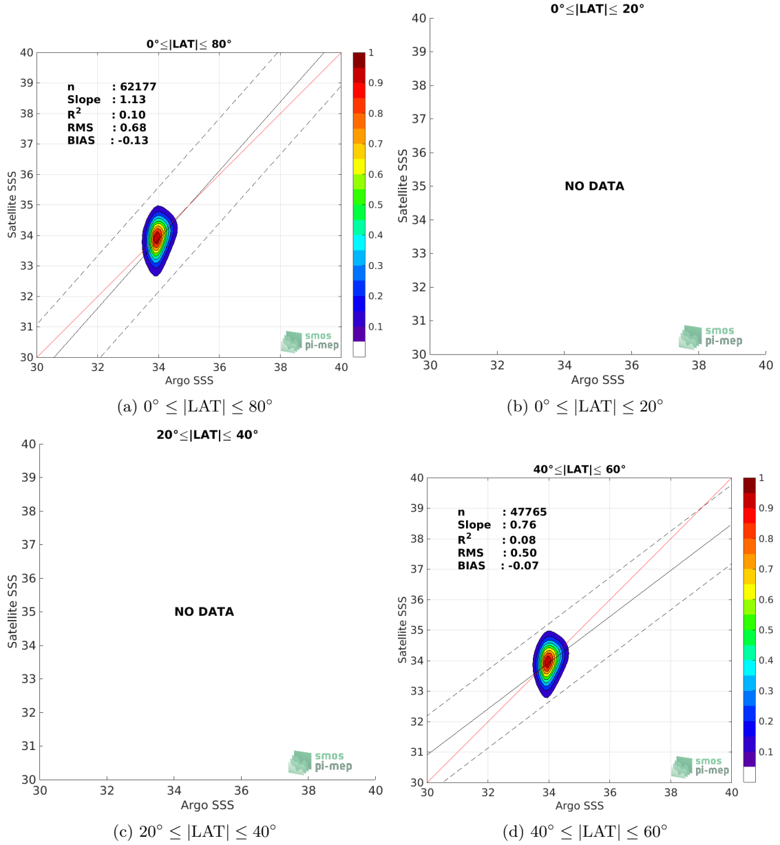
Figure 9: Contour maps of the concentration of SMAP SSS L3 v4 - 8-Day running (RSS) SSS (y-axis) versus Argo SSS (x-axis) at match-up pairs for different latitude bands. For each plot, the red line shows x=y . The black thin and dashed lines indicate a linear fit through the data cloud and the \pm 95\% confidence levels, respectively. The number match-up pairs n , the slope and R^2 coefficient of the linear fit, the root mean square (RMS) and the mean bias between satellite and in situ data are indicated for each latitude band in each plots.
