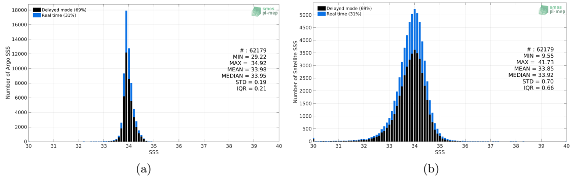
Figure 2: Histograms of SSS from Argo (a) and SMAP SSS L3 v4 - 8-Day running (RSS) (b) considering all match-up pairs per bins of 0.1 over the Southern Ocean Pi-MEP region and for the full satellite product period.
