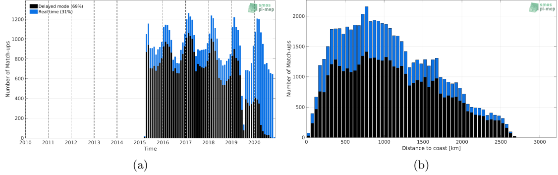
Figure 1: Number of match-ups between Argo and SMAP SSS L3 v4 - 8-Day running (RSS) SSS as a function of time (a) and as function of the distance to coast (b) over the Southern Ocean Pi-MEP region and for the full satellite product period.
