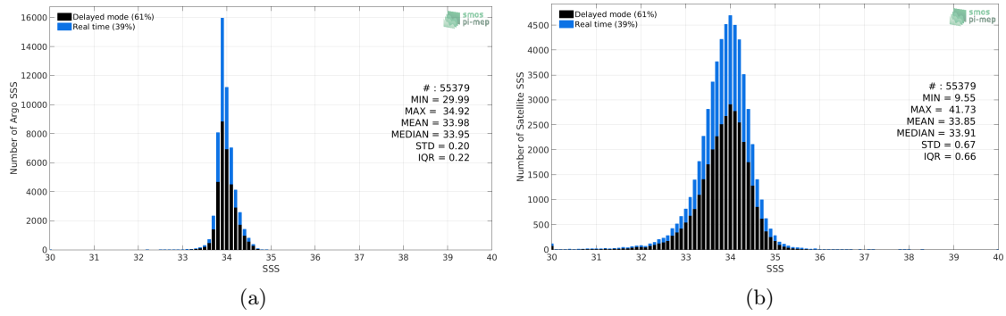
Figure 2: Histograms of SSS from Argo (a) and SMAP-L3-RSS-V4-8DAY-RUNNING (b) considering all match-up pairs per bins of 0.1 over the Southern Ocean Pi-MEP region and for the full satellite product period.
