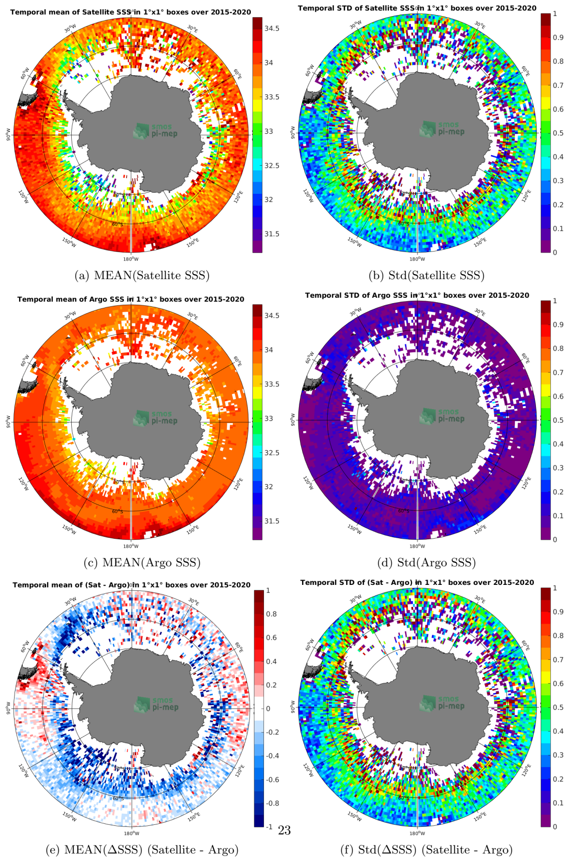
Figure 6: Temporal mean (left) and Std (right) of SSS from SMAP-L3-RSS-V4-8DAY-RUNNING (top), Argo (middle), and of \Delta SSS (Satellite - Argo). Only match-up pairs are used to generate these maps.
