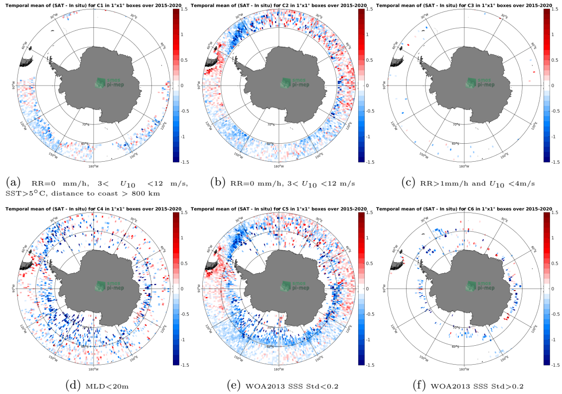
Figure 12: Temporal mean gridded over spatial boxes of size 1^{\circ}\times 1^{\circ} of \Delta\text{SSS} (SMAP-L3-RSS-V4-8DAY-RUNNING - Argo) for 6 different subdatasets corresponding to: \text{RR}=0 mm/h, 3 < U_{10} < 12 m/s, \text{SST} > 5^{\circ}\text{C} , distance to coast > 800 km (a), \text{RR}=0 mm/h, 3 < U_{10} < 12 m/s (b), \text{RR} > 1 mm/h and U_{10} < 4 m/s (c), \text{MLD} < 20\text{m} (d), WOA2013 SSS Std < 0.2 (e), WOA2013 SSS Std > 0.2 (f).
