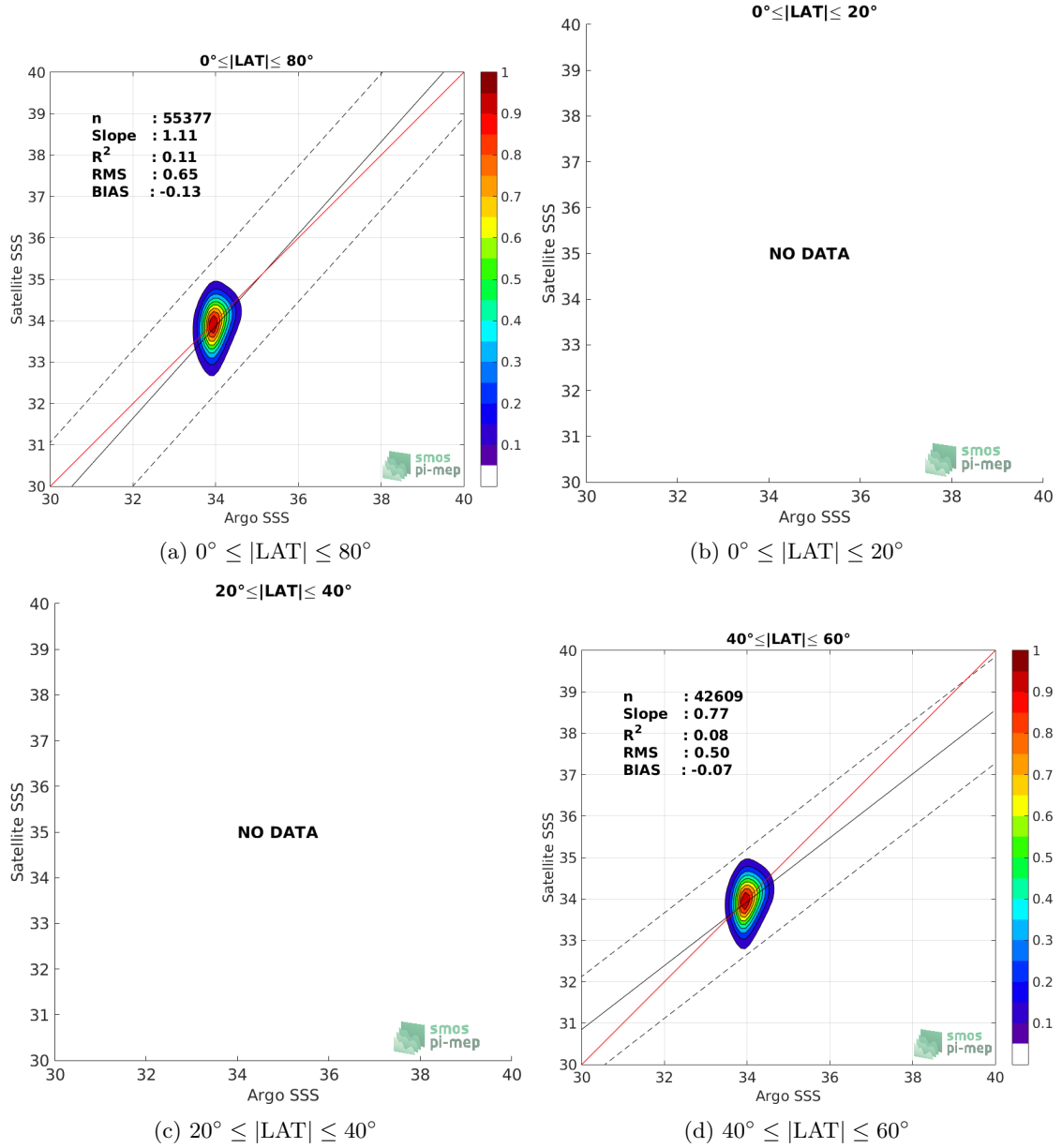
Figure 9: Contour maps of the concentration of SMAP-L3-RSS-V4-8DAY-RUNNING SSS (y-axis) versus Argo SSS (x-axis) at match-up pairs for different latitude bands. For each plot, the red line shows x=y . The black thin and dashed lines indicate a linear fit through the data cloud and the \pm 95\% confidence levels, respectively. The number match-up pairs n , the slope and R^2 coefficient of the linear fit, the root mean square (RMS) and the mean bias between satellite and in situ data are indicated for each latitude band in each plots.
