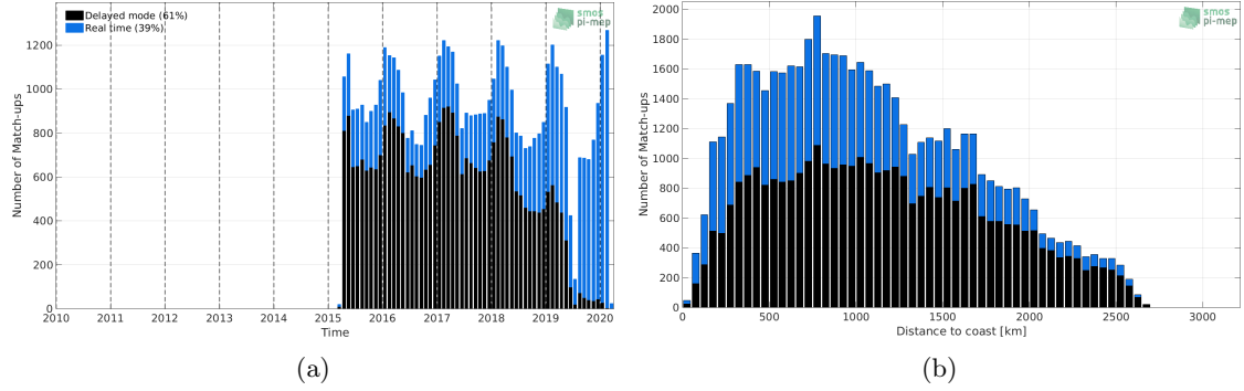
Figure 1: Number of match-ups between Argo and SMAP-L3-RSS-V4-8DAY-RUNNING SSS as a function of time (a) and as function of the distance to coast (b) over the Southern Ocean Pi-MEP region and for the full satellite product period.
