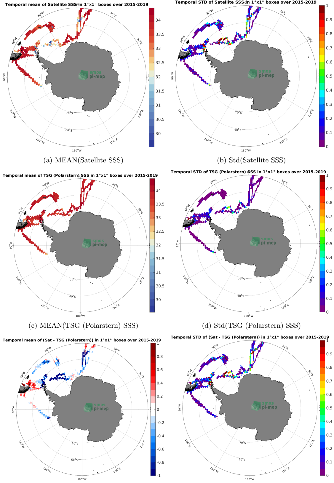
(e) MEAN( \Delta SSS) (Satellite - TSG (Polarstern)) 23 (f) Std( \Delta SSS) (Satellite - TSG (Polarstern)) Figure 6: Temporal mean (left) and Std (right) of SSS from SMAP SSS L3 v4 - Monthly (RSS) (top), TSG (Polarstern) (middle), and of \Delta SSS (Satellite - TSG (Polarstern)). Only match-up pairs are used to generate these maps.
