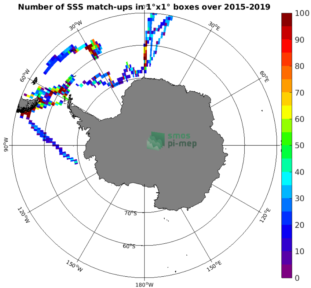
Figure 4: Number of SSS match-ups between TSG (Polarstern) SSS and the SMAP SSS L3 v4 - Monthly (RSS) SSS product for the Southern Ocean Pi-MEP region over 1^\circ \times 1^\circ boxes and for the full satellite product period.
