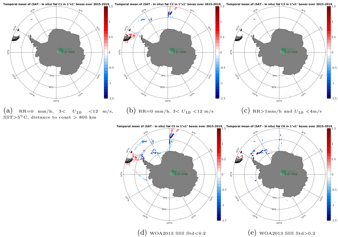
Figure 12: Temporal mean gridded over spatial boxes of size 1^{\circ}\times 1^{\circ} of \Delta\text{SSS} (SMAP-L3-RSS-V4-MONTHLY - TSG-POLARSTERN) for 5 different subdatasets corresponding to:RR=0 mm/h, 3 < U_{10} < 12 m/s, SST >5^{\circ}\text{C} , distance to coast > 800 km (a), RR=0 mm/h, 3 < U_{10} < 12 m/s (b), RR >1 mm/h and U_{10} < 4 m/s (c), WOA2013 SSS Std <0.2 (d), WOA2013 SSS Std >0.2 (e).
