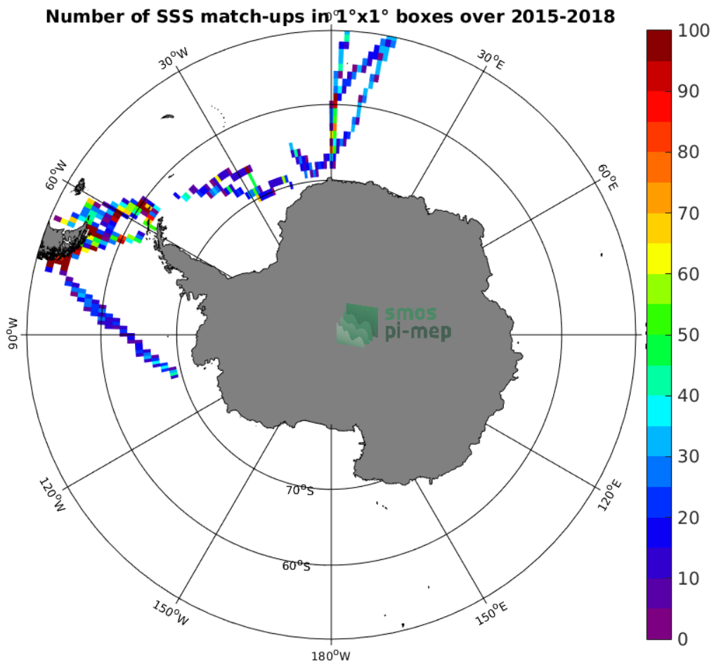
Figure 4: Number of SSS match-ups between TSG-POLARSTERN SSS and the SMAP-L3-RSS-V4-MONTHLY SSS product for the Southern Ocean Pi-MEP region over 1^\circ \times 1^\circ boxes and for the full satellite product period.
