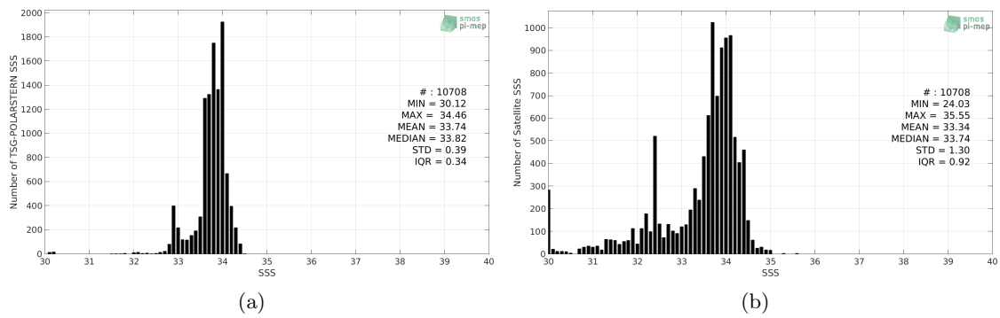
Figure 2: Histograms of SSS from TSG-POLARSTERN (a) and SMAP-L3-RSS-V4-MONTHLY (b) considering all match-up pairs per bins of 0.1 over the Southern Ocean Pi-MEP region and for the full satellite product period.
