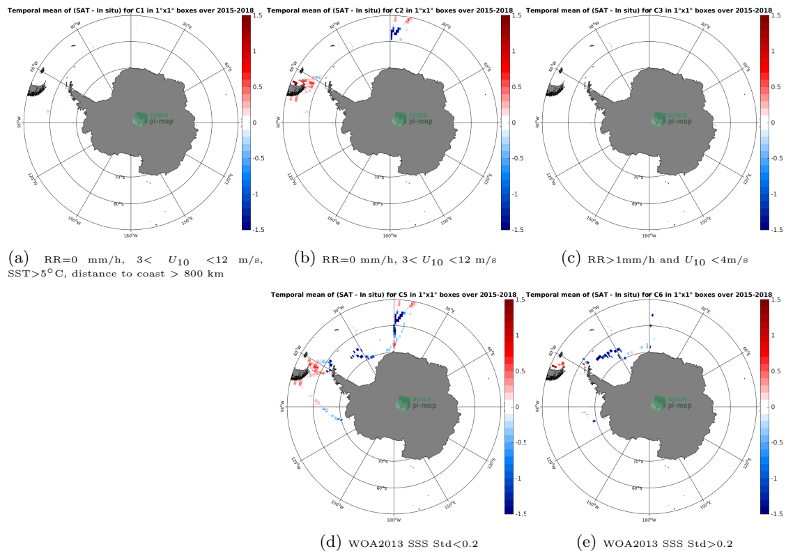
Figure 12: Temporal mean gridded over spatial boxes of size 1^\circ \times 1^\circ of \Delta SSS (SMAP-L3-RSS-V4-MONTHLY - TSG-POLARSTERN) for 5 different subdatasets corresponding to: RR=0 mm/h, 3 < U_{10} < 12 m/s, SST > 5^\circ\text{C} , distance to coast > 800 km (a), RR=0 mm/h, 3 < U_{10} < 12 m/s (b), RR > 1 mm/h and U_{10} < 4 m/s (c), WOA2013 SSS Std < 0.2 (d), WOA2013 SSS Std > 0.2 (e).
