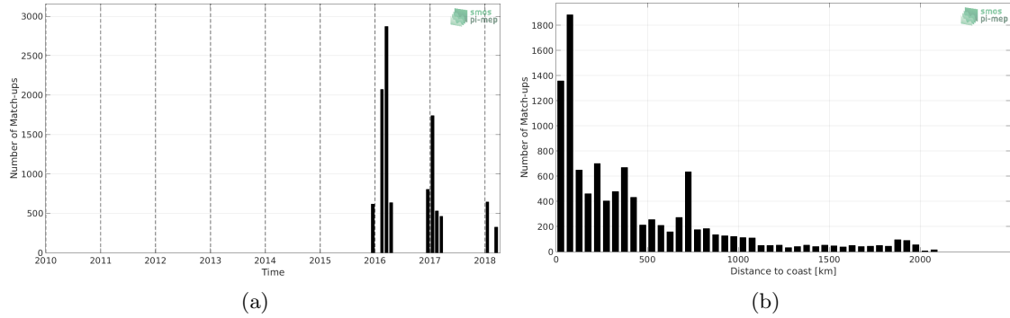
Figure 1: Number of match-ups between TSG-POLARSTERN and SMAP-L3-RSS-V4-MONTHLY SSS as a function of time (a) and as function of the distance to coast (b) over the Southern Ocean Pi-MEP region and for the full satellite product period.
