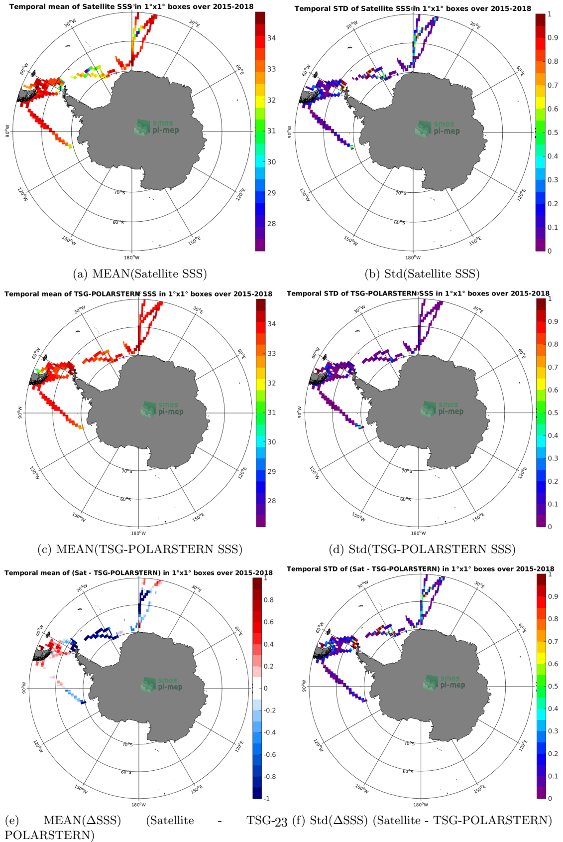
Figure 6: Temporal mean (left) and Std (right) of SSS from SMAP-L3-RSS-V4-MONTHLY (top), TSG-POLARSTERN (middle), and of \Delta SSS (Satellite - TSG-POLARSTERN). Only match-up pairs are used to generate these maps.
