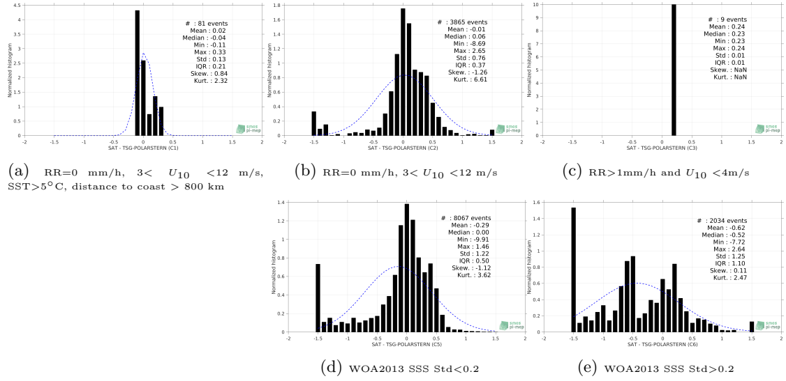
Figure 13: Normalized histogram of \Delta SSS (SMAP-L3-RSS-V4-MONTHLY - TSG-POLARSTERN) for 5 different subdatasets corresponding to: RR=0 mm/h, 3 < U_{10} < 12 m/s, SST > 5°C, distance to coast > 800 km (a), RR=0 mm/h, 3 < U_{10} < 12 m/s (b), RR > 1mm/h and U_{10} < 4 m/s (c), WOA2013 SSS Std < 0.2 (d), WOA2013 SSS Std > 0.2 (e).
