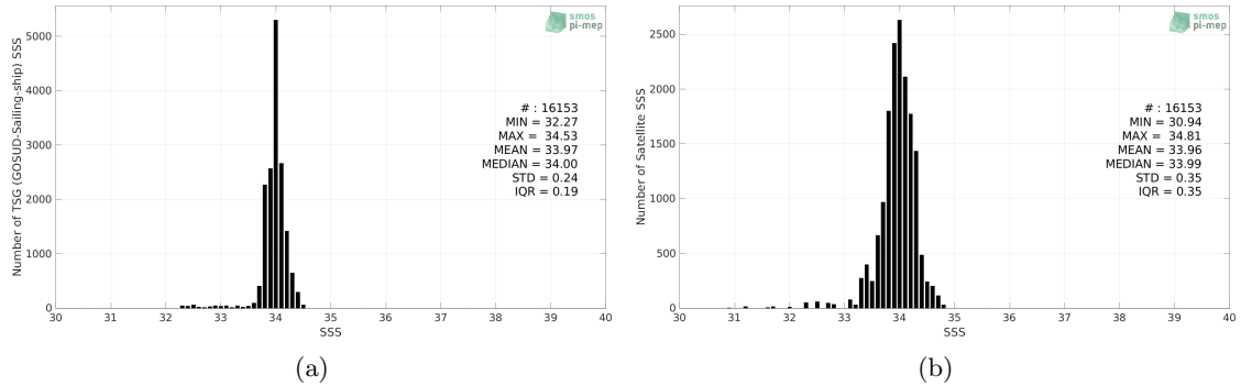
Figure 2: Histograms of SSS from TSG (GOSUD-Sailing-ship) (a) and SMAP SSS L3 v4 - Monthly (RSS) (b) considering all match-up pairs per bins of 0.1 over the Southern Ocean Pi-MEP region and for the full satellite product period.
