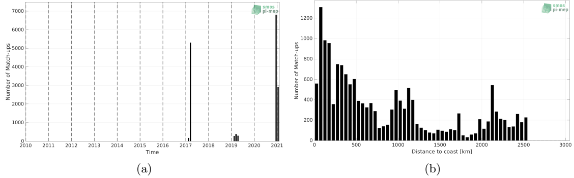
Figure 1: Number of match-ups between TSG (GOSUD-Sailing-ship) and SMAP SSS L3 v4 - Monthly (RSS) SSS as a function of time (a) and as function of the distance to coast (b) over the Southern Ocean Pi-MEP region and for the full satellite product period.
