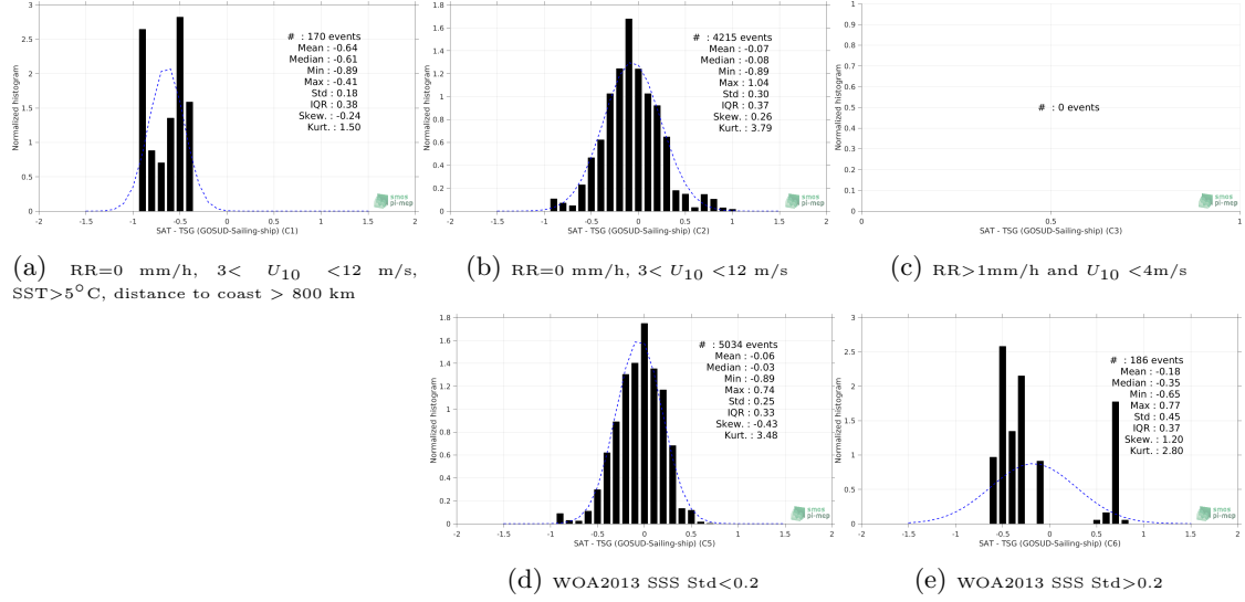
Figure 13: Normalized histogram of \Delta\text{SSS} (SMAP SSS L3 v4 - Monthly (RSS) - TSG (GOSUD-Sailing-ship)) for 5 different subdatasets corresponding to: RR=0 mm/h, 3 < U_{10} < 12 m/s, SST > 5^{\circ}\text{C} , distance to coast > 800 km (a), RR=0 mm/h, 3 < U_{10} < 12 m/s (b), RR > 1\text{mm/h} and U_{10} < 4\text{m/s} (c), WOA2013 SSS Std < 0.2 (d), WOA2013 SSS Std > 0.2 (e).
