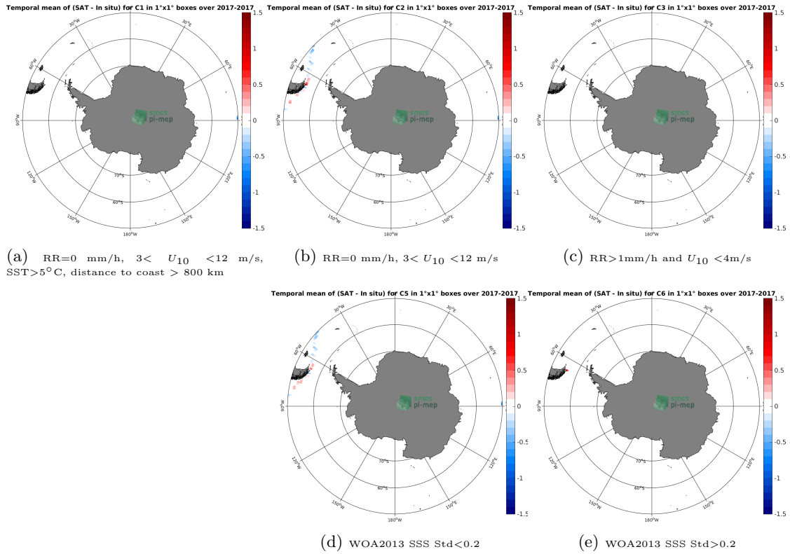
Figure 12: Temporal mean gridded over spatial boxes of size 1°x1° of \Delta SSS (SMAP-L3-RSS-V4-MONTHLY - TSG-GOSUD-Sailing-ship) for 5 different subdatasets corresponding to: RR=0 mm/h, 3 < U_{10} < 12 m/s, SST > 5°C, distance to coast > 800 km (a), RR=0 mm/h, 3 < U_{10} < 12 m/s (b), RR > 1mm/h and U_{10} < 4 m/s (c), WOA2013 SSS Std < 0.2 (d), WOA2013 SSS Std > 0.2 (e).
