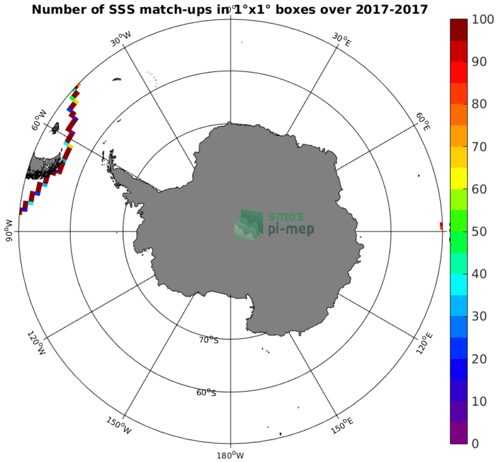
Figure 4: Number of SSS match-ups between TSG-GOSUD-Sailing-ship SSS and the SMAP-L3-RSS-V4-MONTHLY SSS product for the Southern Ocean Pi-MEP region over 1°x1° boxes and for the full satellite product period.
