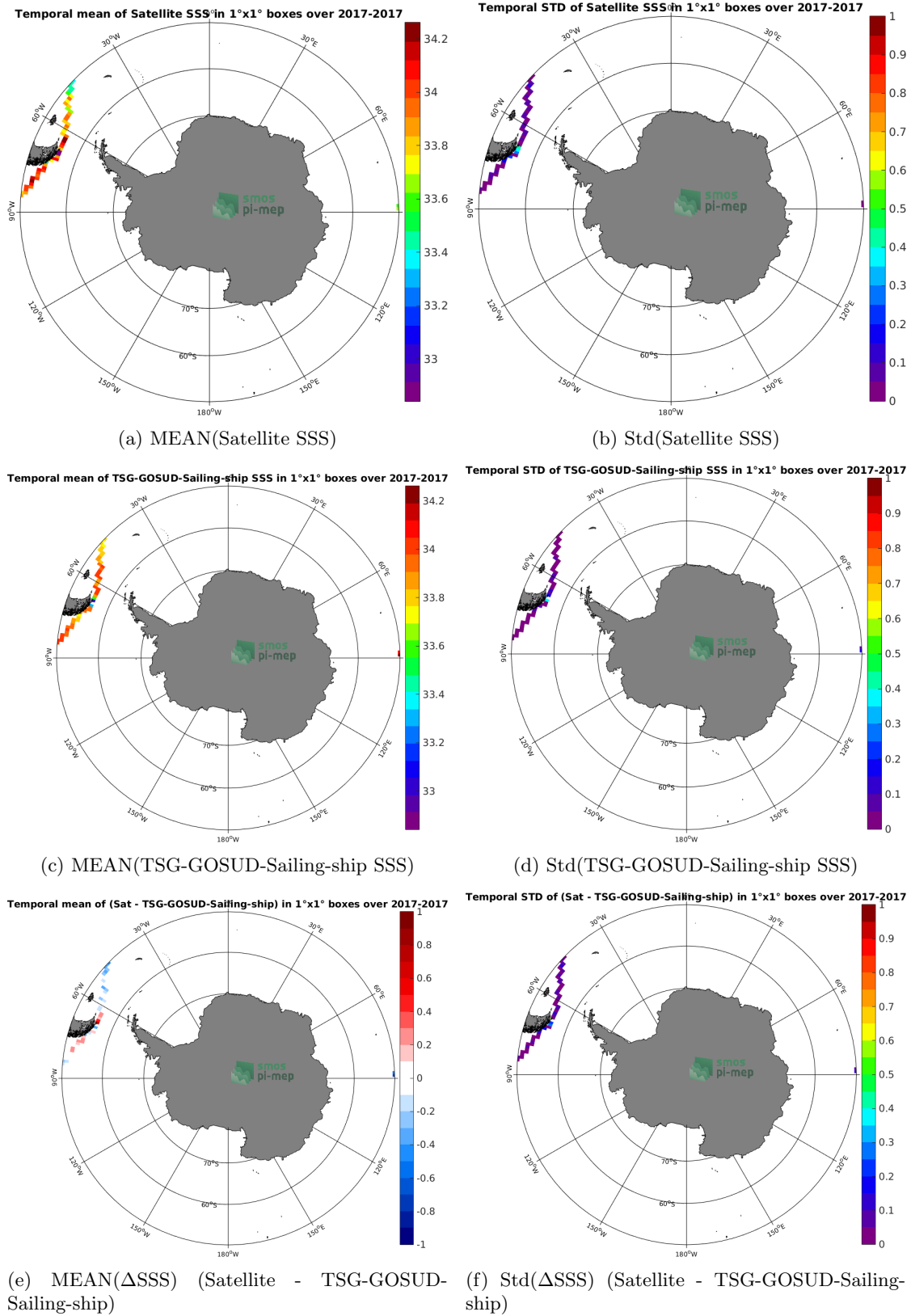
Figure 6: Temporal mean (left) and Std (right) of SSS from SMAP-L3-RSS-V4-MONTHLY (top), TSG-GOSUD-Sailing-ship (middle), and of \Delta SSS (Satellite - TSG-GOSUD-Sailing-ship). Only match-up pairs are used to generate these maps.
