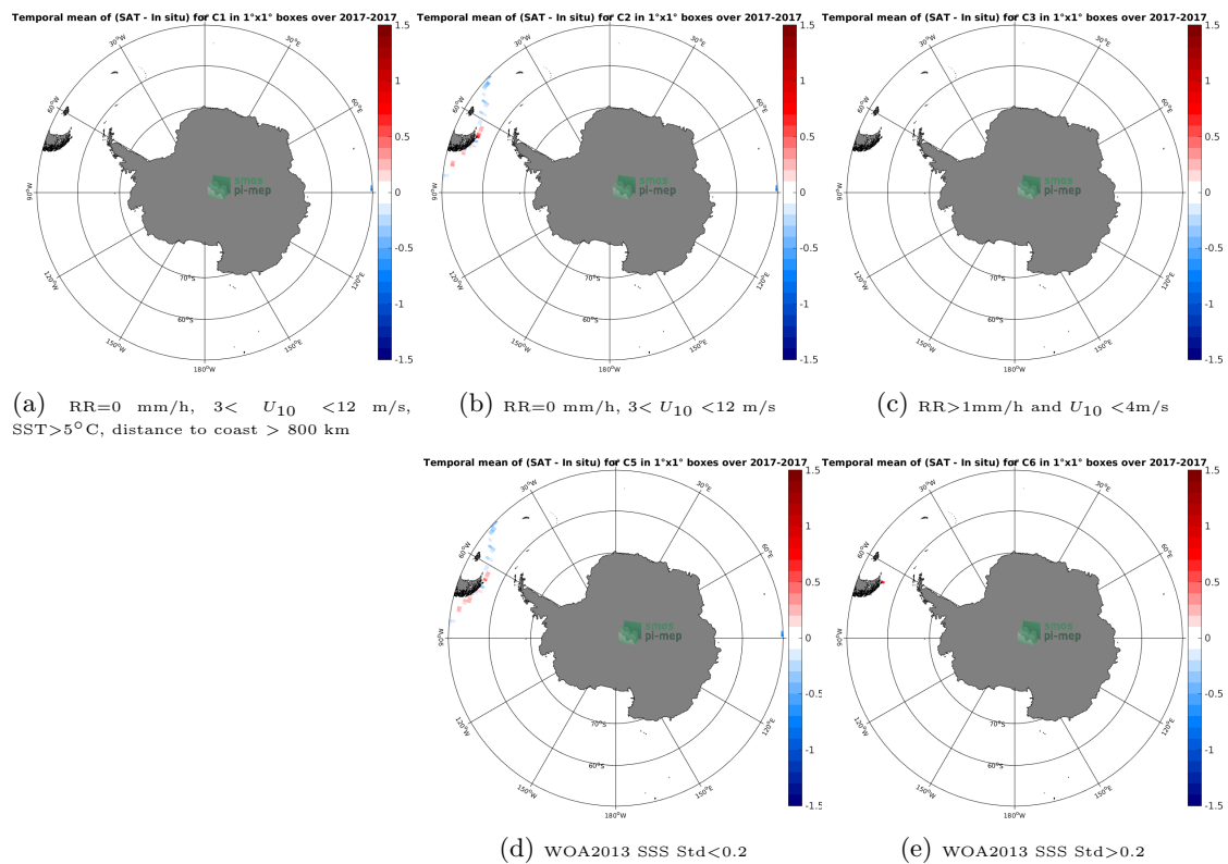
Figure 12: Temporal mean gridded over spatial boxes of size 1^\circ \times 1^\circ of \Delta SSS (SMAP-L3-RSS-V4-MONTHLY - TSG-GOSUD-Sailing-ship) for 5 different subdatasets corresponding to:RR=0 mm/h, 3 < U_{10} < 12 m/s, SST >5^\circ\text{C} , distance to coast > 800 km (a), RR=0 mm/h, 3 < U_{10} < 12 m/s (b), RR >1 mm/h and U_{10} < 4 m/s (c), WOA2013 SSS Std <0.2 (d), WOA2013 SSS Std >0.2 (e).
