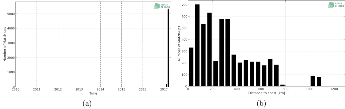
Figure 1: Number of match-ups between TSG-GOSUD-Sailing-ship and SMAP-L3-RSS-V4-MONTHLY SSS as a function of time (a) and as function of the distance to coast (b) over the Southern Ocean Pi-MEP region and for the full satellite product period.
