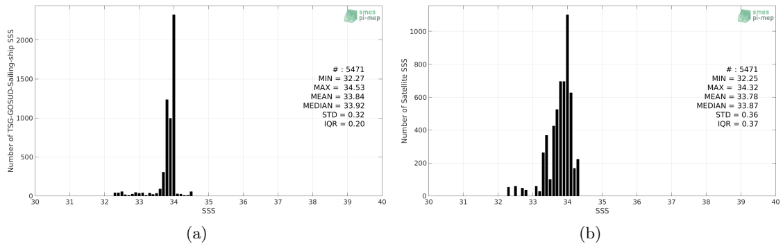
Figure 2: Histograms of SSS from TSG-GOSUD-Sailing-ship (a) and SMAP-L3-RSS-V4-MONTHLY (b) considering all match-up pairs per bins of 0.1 over the Southern Ocean Pi-MEP region and for the full satellite product period.
