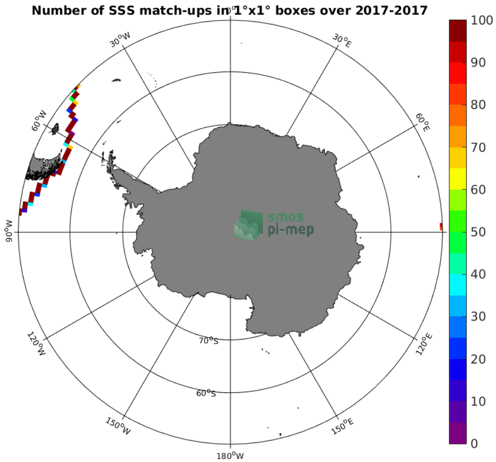
Figure 4: Number of SSS match-ups between TSG-GOSUD-Sailing-ship SSS and the SMAP-L3-RSS-V4-MONTHLY SSS product for the Southern Ocean Pi-MEP region over 1^{\circ} \times 1^{\circ} boxes and for the full satellite product period.
