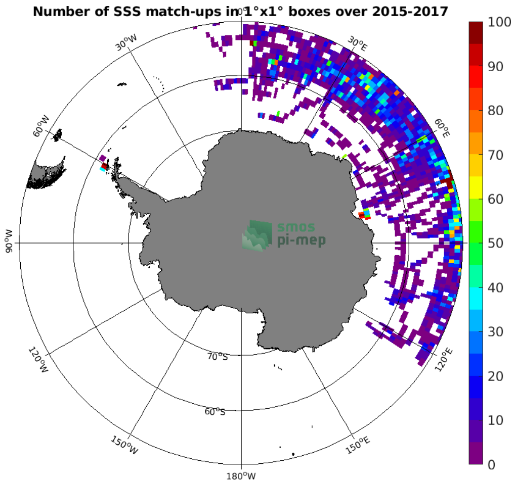
Figure 4: Number of SSS match-ups between Sea mammals SSS and the SMAP SSS L3 v4 - Monthly (RSS) SSS product for the Southern Ocean Pi-MEP region over 1^\circ \times 1^\circ boxes and for the full satellite product period.
