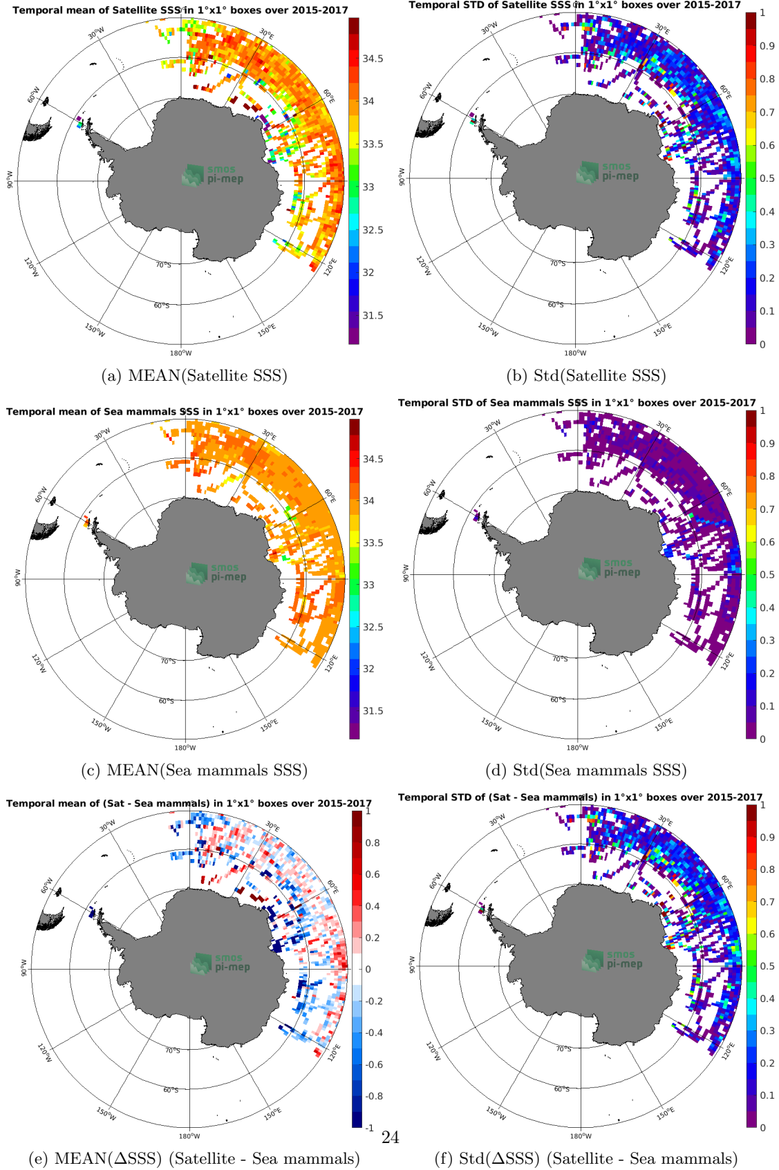
Figure 6: Temporal mean (left) and Std (right) of SSS from SMAP SSS L3 v4 - Monthly (RSS) (top), Sea mammals (middle), and of \Delta SSS (Satellite - Sea mammals). Only match-up pairs are used to generate these maps.
