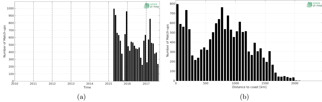
Figure 1: Number of match-ups between Sea mammals and SMAP-L3-RSS-V4-MONTHLY SSS as a function of time (a) and as function of the distance to coast (b) over the Southern Ocean Pi-MEP region and for the full satellite product period.
