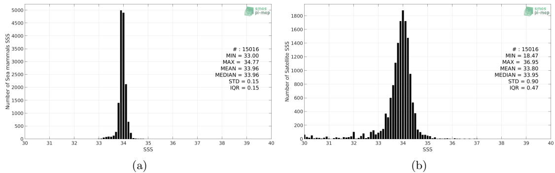
Figure 2: Histograms of SSS from Sea mammals (a) and SMAP-L3-RSS-V4-MONTHLY (b) considering all match-up pairs per bins of 0.1 over the Southern Ocean Pi-MEP region and for the full satellite product period.
