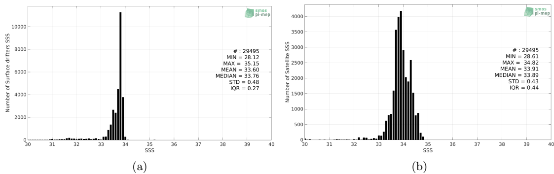
Figure 2: Histograms of SSS from Surface drifters (a) and SMAP SSS L3 v4 - Monthly (RSS) (b) considering all match-up pairs per bins of 0.1 over the Southern Ocean Pi-MEP region and for the full satellite product period.
