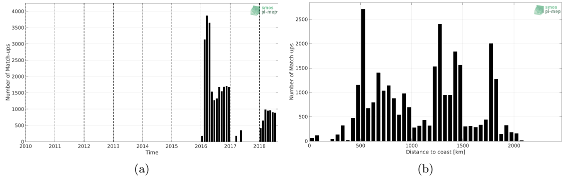
Figure 1: Number of match-ups between Surface drifters and SMAP SSS L3 v4 - Monthly (RSS) SSS as a function of time (a) and as function of the distance to coast (b) over the Southern Ocean Pi-MEP region and for the full satellite product period.
