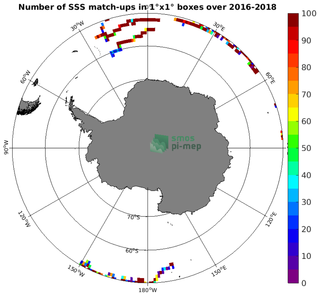
Figure 3: Number of SSS match-ups between Surface drifters SSS and the SMAP SSS L3 v4 - Monthly (RSS) SSS product for the Southern Ocean Pi-MEP region over 1^\circ \times 1^\circ boxes and for the full satellite product period.
