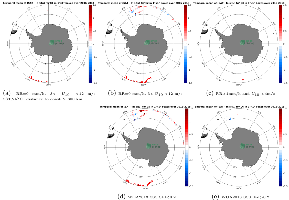
Figure 11: Temporal mean gridded over spatial boxes of size 1^{\circ}\times 1^{\circ} of \Delta\text{SSS} (SMAP SSS L3 v4 - Monthly (RSS) - Surface drifters) for 5 different subdatasets corresponding to: \text{RR}=0 mm/h, 3 < U_{10} < 12 m/s, \text{SST}>5^{\circ}\text{C} , distance to coast > 800 km (a), \text{RR}=0 mm/h, 3 < U_{10} < 12 m/s (b), \text{RR}>1\text{mm/h} and U_{10} < 4\text{m/s} (c), WOA2013 SSS Std < 0.2 (d), WOA2013 SSS Std > 0.2 (e).
