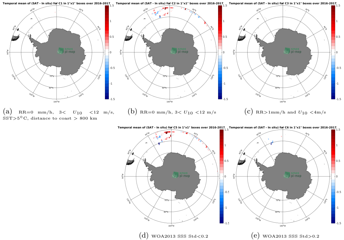
Figure 11: Temporal mean gridded over spatial boxes of size 1^\circ \times 1^\circ of \Delta SSS (SMAP-L3-RSS-V4-MONTHLY - Surface drifters) for 5 different subdatasets corresponding to:RR=0 mm/h, 3 < U_{10} < 12 m/s, SST >5^\circ C, distance to coast > 800 km (a), RR=0 mm/h, 3 < U_{10} < 12 m/s (b), RR >1 mm/h and U_{10} < 4 m/s (c), WOA2013 SSS Std <0.2 (d), WOA2013 SSS Std >0.2 (e).
